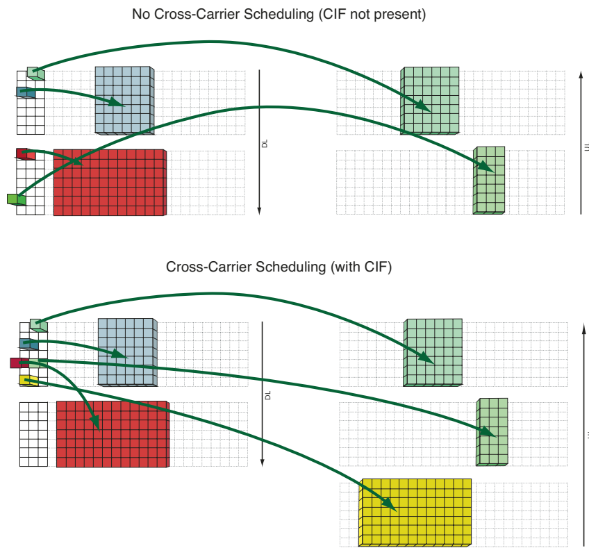
Figure 17 - Cross-Carrier scheduling.
