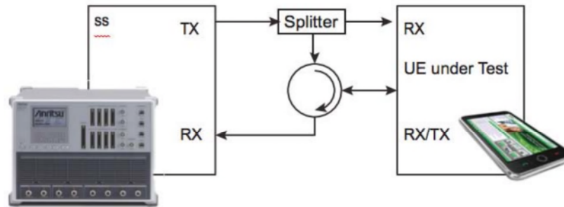
Test setup
