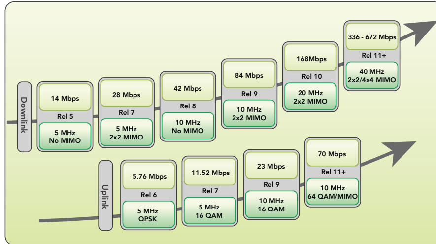
Figure 2 - Evolution of throughput in HSPA with Carrier Aggregation.
