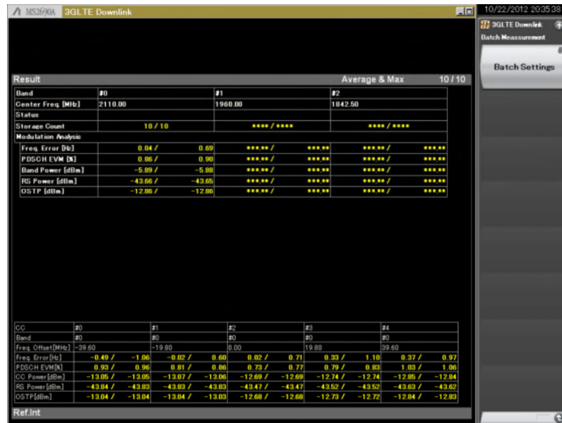
Figure 23 - Measurement software MX269020A-001. Example of Batch Measurement Result Display (Component Carrier: CC #0 to #4)
