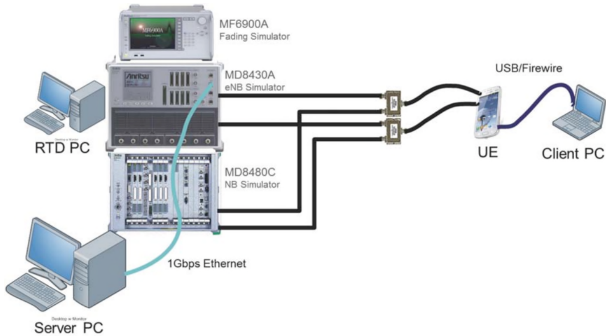
Test setup
