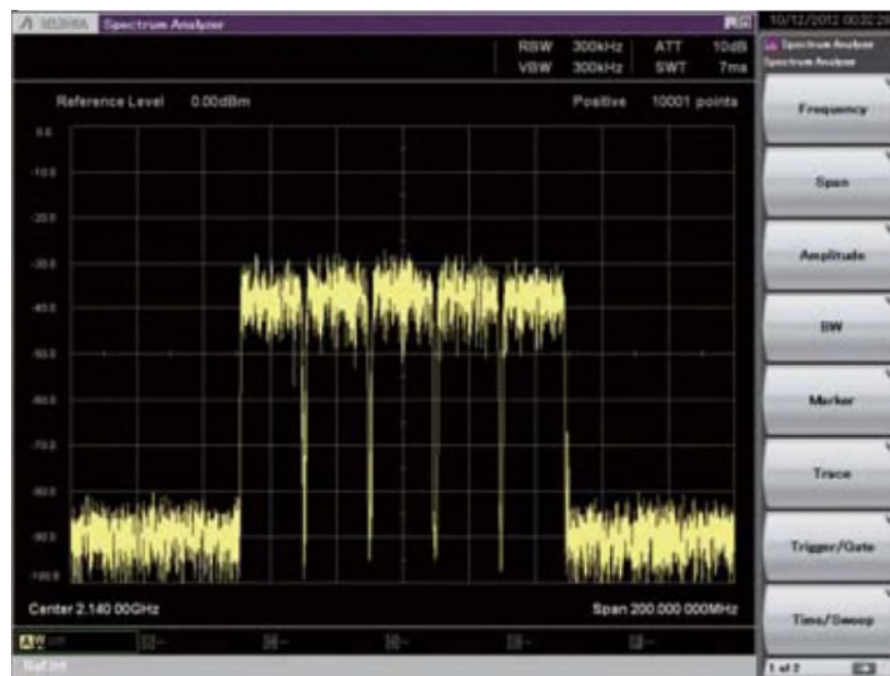
Figure 22 - Spectrum analyzer MS269xA/MS2830A . Example of Spectrum of LTE- Advanced signal (Component Carrier: Bandwidth 20 MHz, 5CC)
