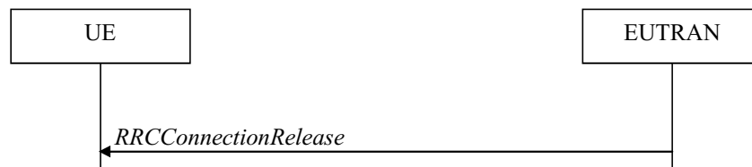
Figure 5.3.8.1-1: RRC connection release, successful
