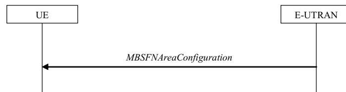
Figure 5.8.2.1-1: MCCH information acquisition
