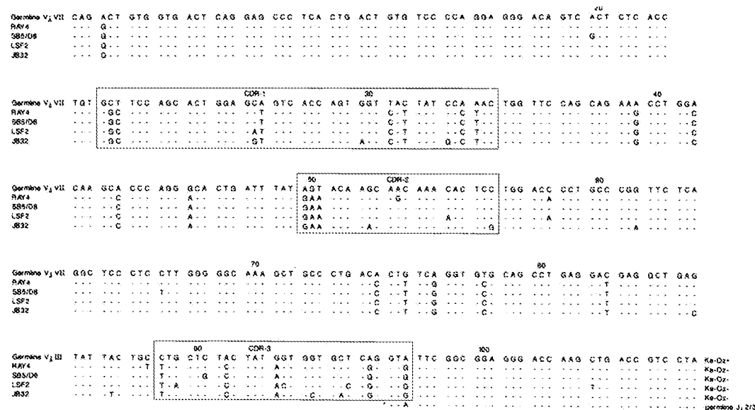
Figure 1. Nucleotide sequences of the V λ and J λ genes from four hybridoma cell lines (RAY4, SB5/D6, LSF2, JB32), and from the V λ VII germline gene, 4A (33). Numbering is according to Kabat (23). These sequence data are available from EMBL/GenBank Data Libraries under accession numbers M80917 (RAY4), M80918 (SB5/D6), M80915 (LSF2), and M80919 (JB32).
