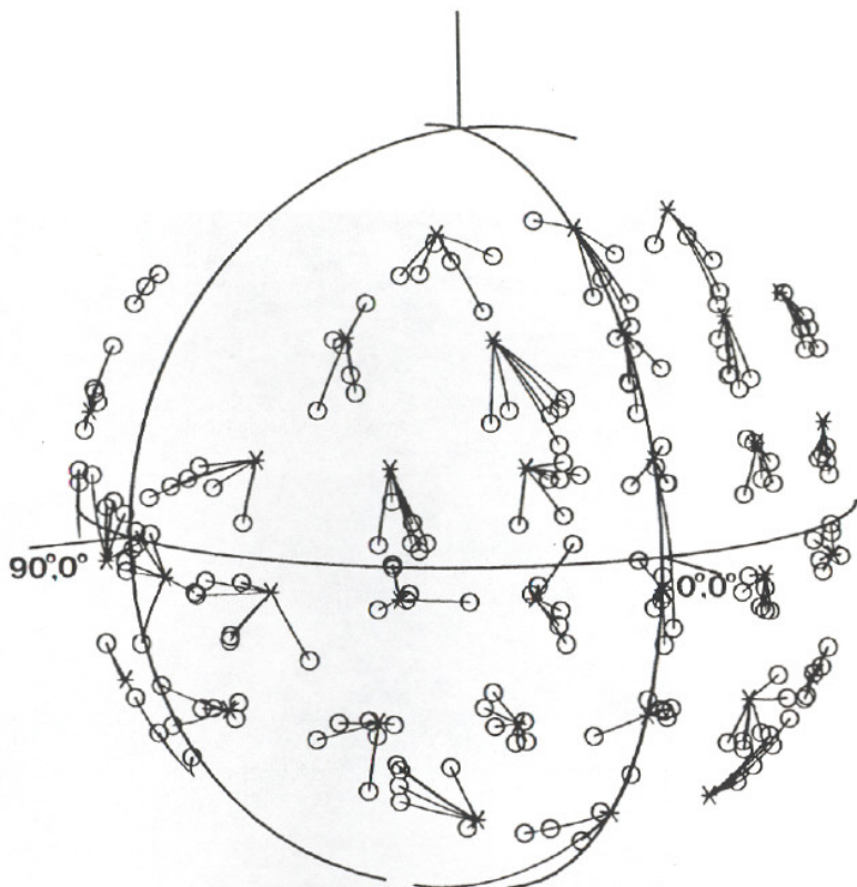
Figure 1 Localization of a broadband sound. Stimulus and response locations are drawn on the surface of an imaginary sphere as if looking in toward the subject from point 30° to the subject's right and elevated 10°. Asterisks indicate the stimulus location and open circles indicate five responses to that stimulus given by a single subject. For clarity, stimulus locations are shown in 20° steps of azimuth and elevation, although data were collected in 10° steps. The data are from the study by Makous & Middlebrooks (1990).
