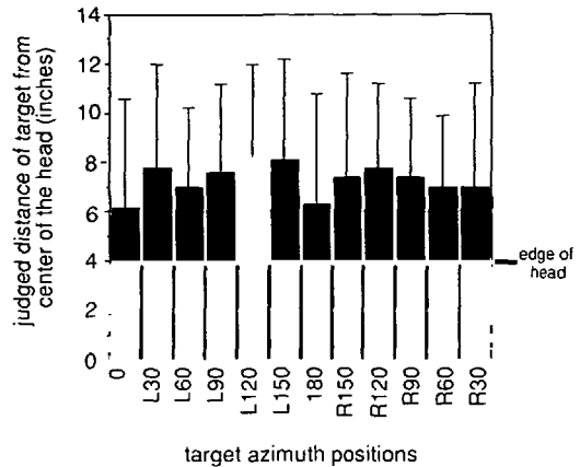
Figure 9. Means and standard deviations of distance judgments collapsed across all subjects. Total of 1650 judgments for 0- and 180-degree targets; 165 judgments for other targets. Distances beyond 4 inches are externalized.
