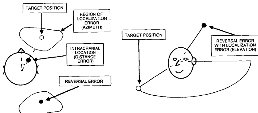
Figure 1. Types of localization error reported in the literature and discussed in the current experiment. Target position is the position of the sound source where the HRTF was measured. Left side: overhead view. Right side: perspective view.
