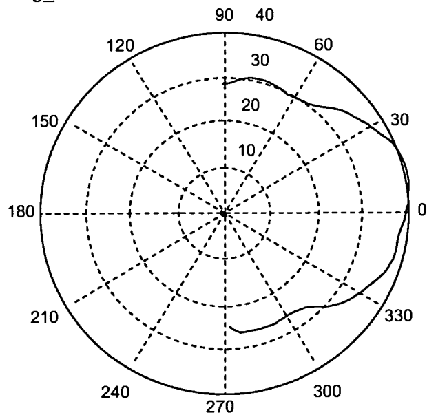
polar_0deg_1000Hz
