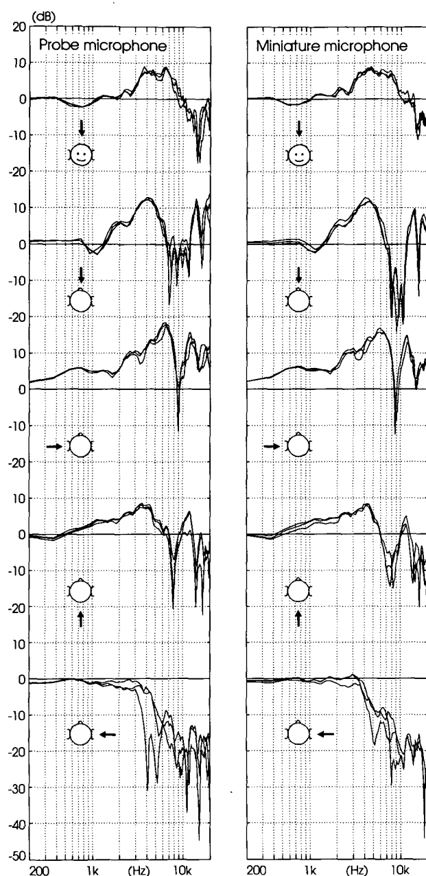
Fig. 20. Three repetition measurements of HRTFs for left ear of subject DOL shown for the five directions measured with both microphone techniques ( \theta = 0^\circ, 90^\circ, 180^\circ , and -90^\circ in horizontal plane; \theta = 90^\circ ).
