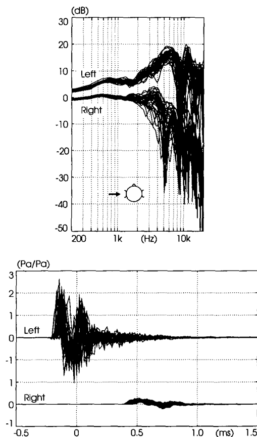
Fig. 10. HRTFs and HRIRs for direction (\phi, \theta) = (90^\circ, 0^\circ) , same as in Fig. 9, but for all 40 subjects.
