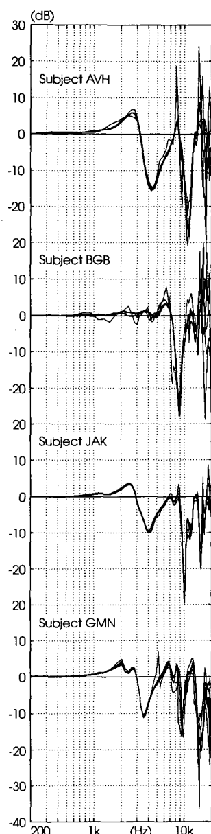
Fig. 17. Examples of pressure division P_3/P_2 for left ears of four subjects. Curves are shown for the five directions ( \phi = 0^\circ, 90^\circ, 180^\circ , and -90^\circ in horizontal plane; \theta = 90^\circ ).
