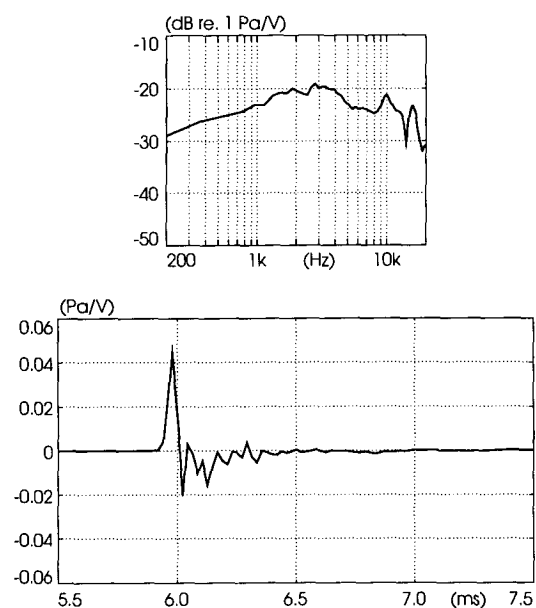
Fig. 7. Typical frequency response and impulse response for loudspeakers (Vifa M10MD-39 mounted in 15.5-mm hard plastic ball), measured at a distance of 2 m with Brüel & Kjær 4136 microphone, 90° incidence.
