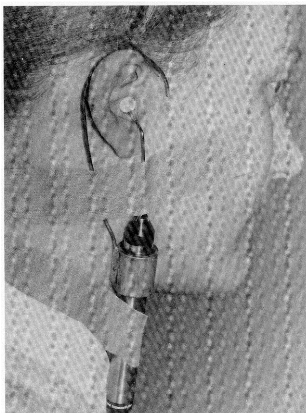
Fig. 3. Probe microphone mounted on human subject to measure blocked ear canal pressure P_2 .
