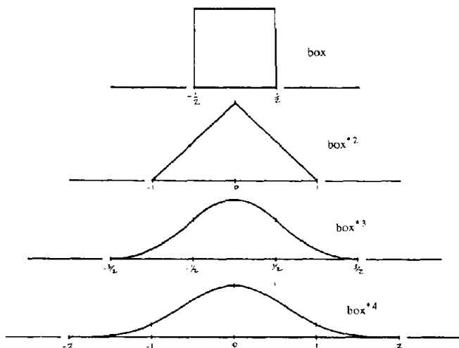
Figure 1: repeated box filters of order 1-4
