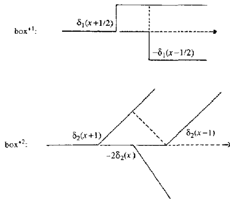
Figure 4: superposition of ramp functions to create first and second order box filters
