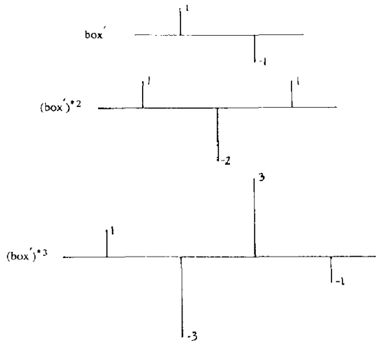
Figure 2: the n th derivative of an n th order box filter is an impulse train
