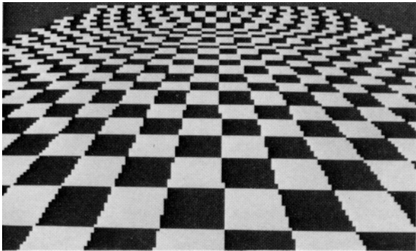
Figure 10: point sampled (order 0)
