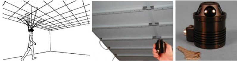
Figure 4.3: Conceptual drawing of inside-looking-out system (Left). Roof mounted infrared led arrays (Middle) and the Hi-ball camera tracker (Right). [Welch et al., 1999]
