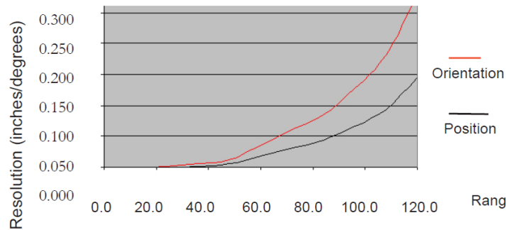
Figure 4.1: Resolution of position and orientation measurements for a magnetic tracker as a function of range between the transmitter and receiver. (Image courtesy of Polhemus http://www.polhemus.com )
