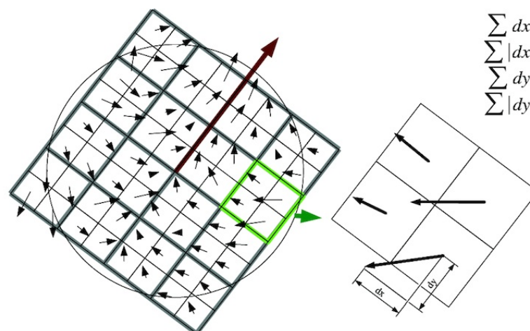
Figure 4.12: The SURF Feature descriptor operates on an oriented square region around a feature point. Haar-wavelets are computed over 4x4 sub-regions, and each sub-region's descriptor field is comprised of the resulting responses \sum dx, \sum dy, \sum |dx|, \sum |dy| . [Bay et al., 2008]
