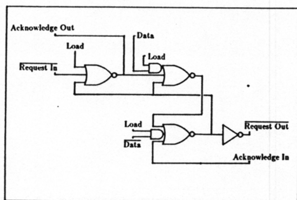
Figure 9 Self-timed packer circuit
