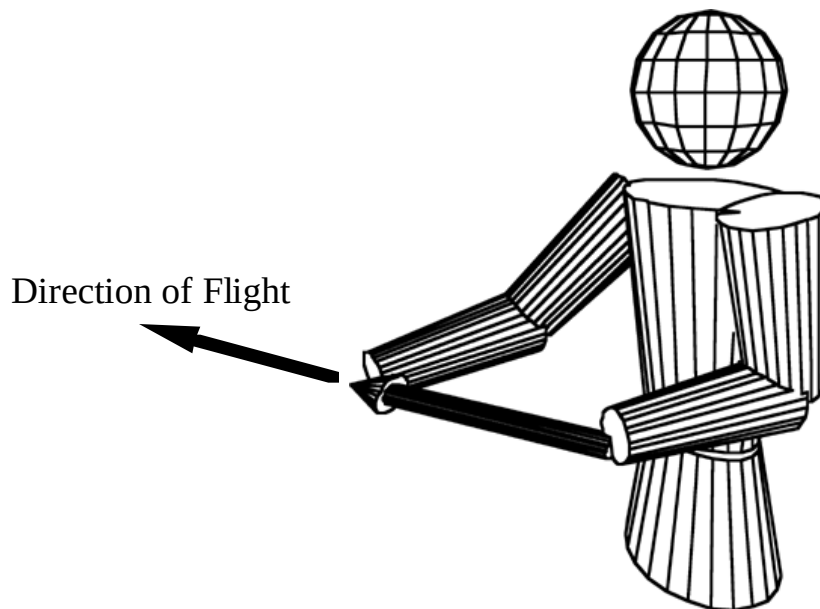
Figure 3.7: Two-handed flying.
