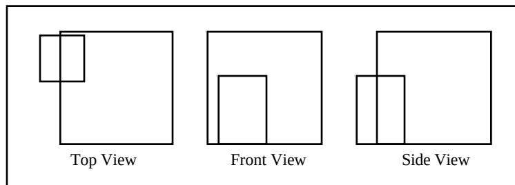
Figure A.2b: Three orthogonal views of the object in Figure A.2a.
