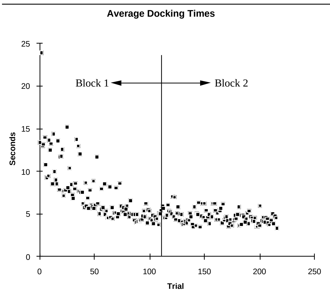
Figure 4.2: Average trial completion time over all users and all techniques.
