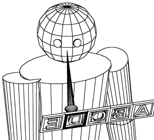
Figure 3.6: Look-at menu.
