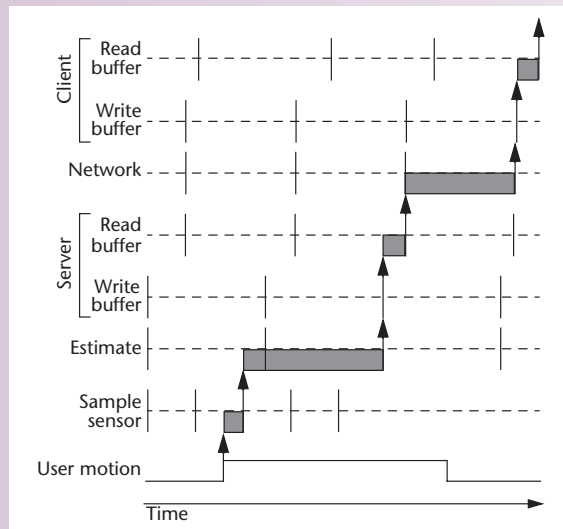
A Typical tracker pipeline.
