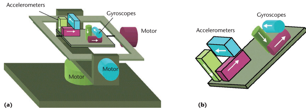
1 (a) Stable-platform (gimbaled) INS. (b) Strapdown INS.
