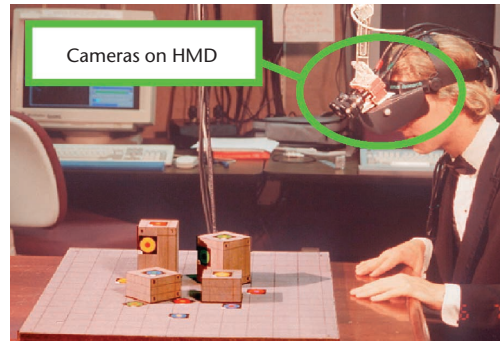
8 Video-based head-mounted display for augmented reality.
