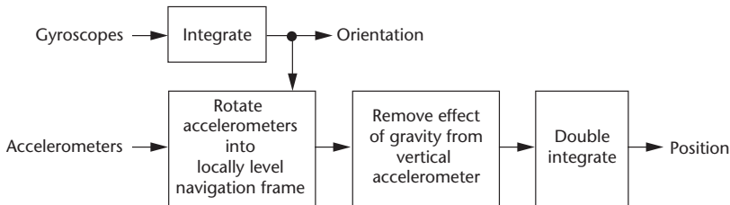
2 Basic strap-down inertial navigation algorithm.
