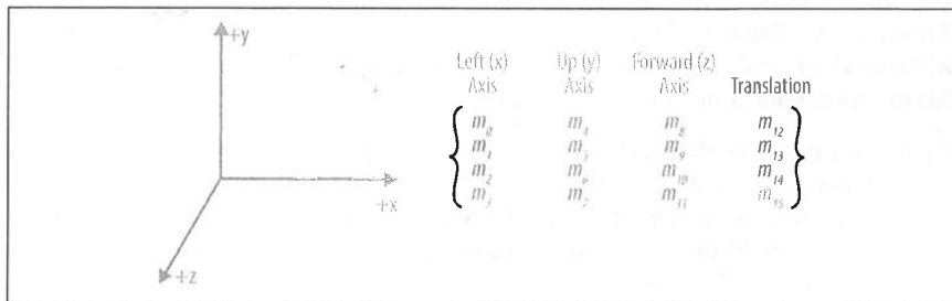
Figure 3-4. A 4x4 transformation matrix defining translation, rotation, and scale
