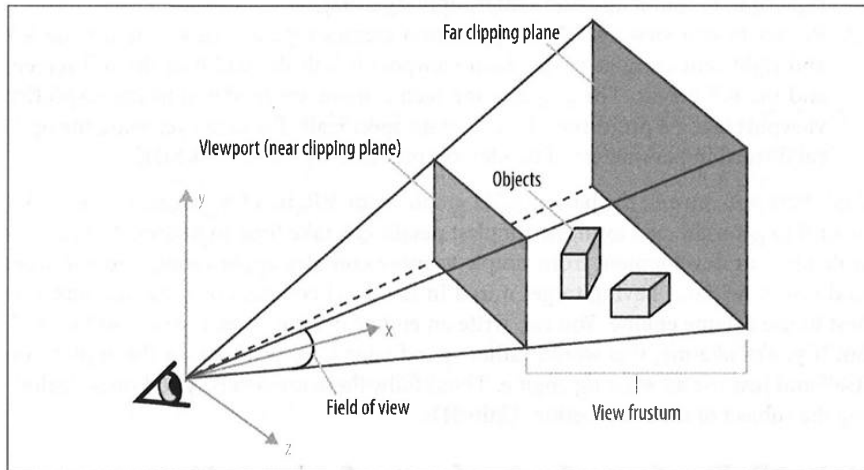
Figure 3-5. Camera, viewport, and perspective projection
