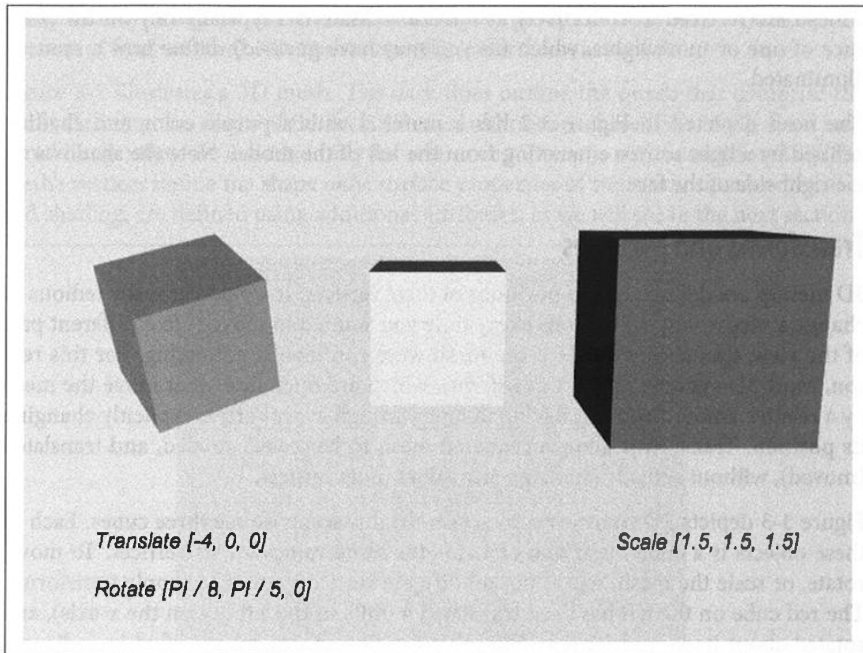
Figure 3-3. 3D transforms: translation, rotation, and scale
