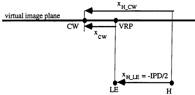
Figure 5. Dependence of x_{cw} on IPD (left eye).
