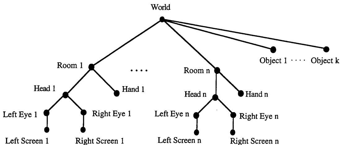
Figure 2. Coordinate systems for a multi-user virtual world.
