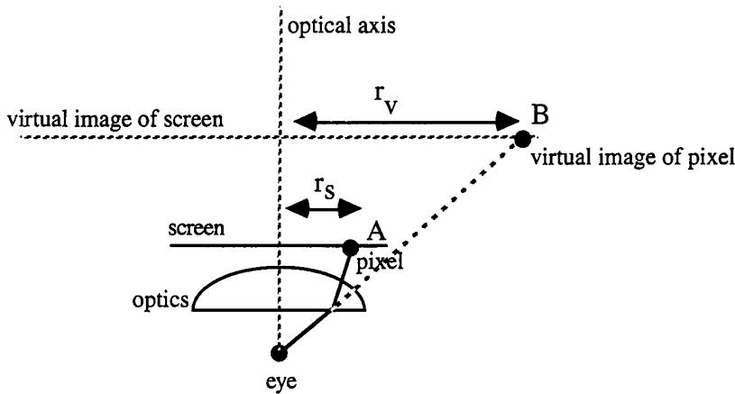
Figure 7. Single-eye optics model.
