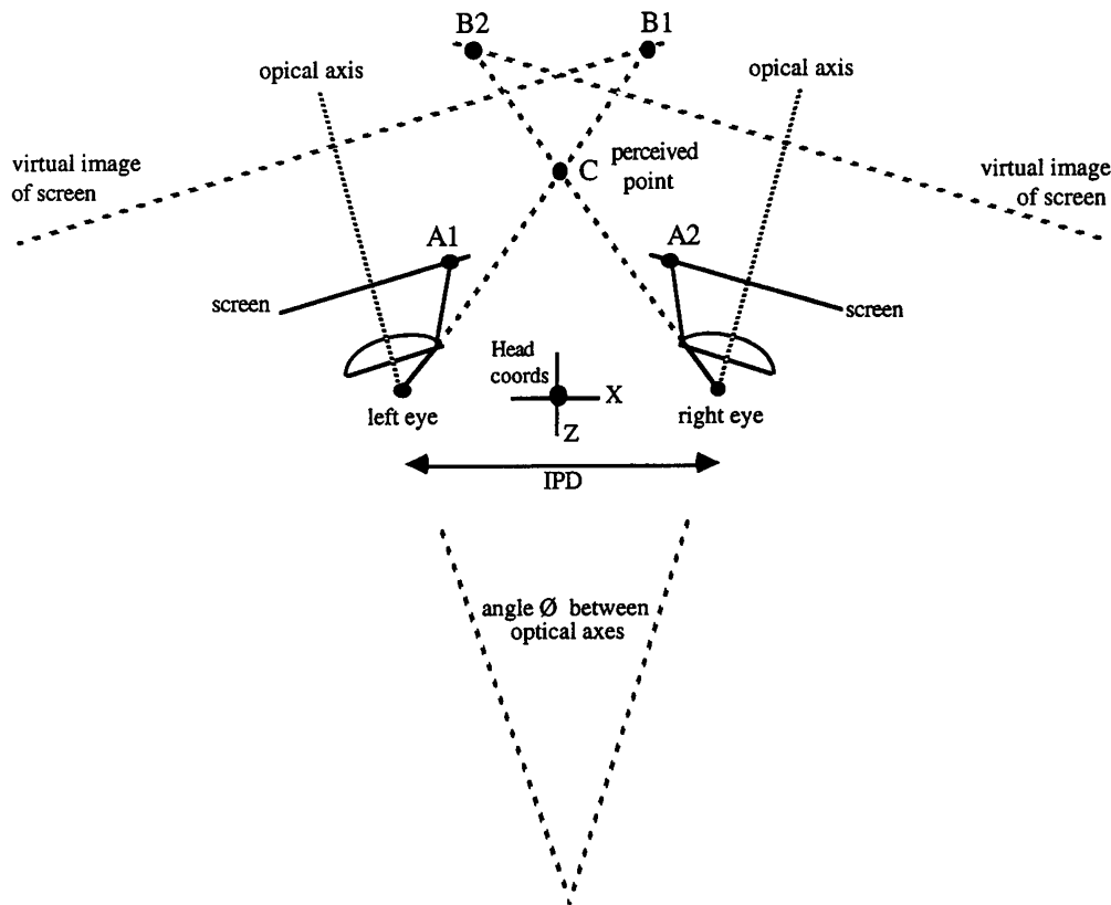
Figure 3. Stereoscopic optics model for an HMD.
