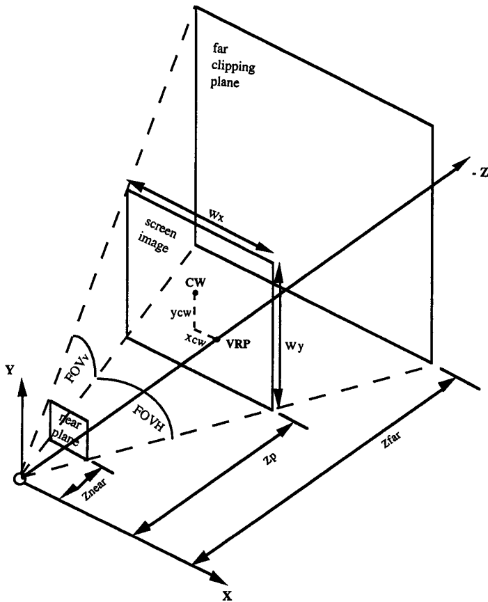
Figure 4. Viewing parameters for one eye using an off-center perspective projection.
