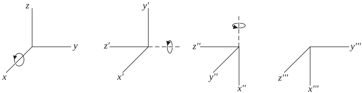
Figure 2a: 90^\circ rotations of a reference frame about the initial x, y, z axes, respectively
