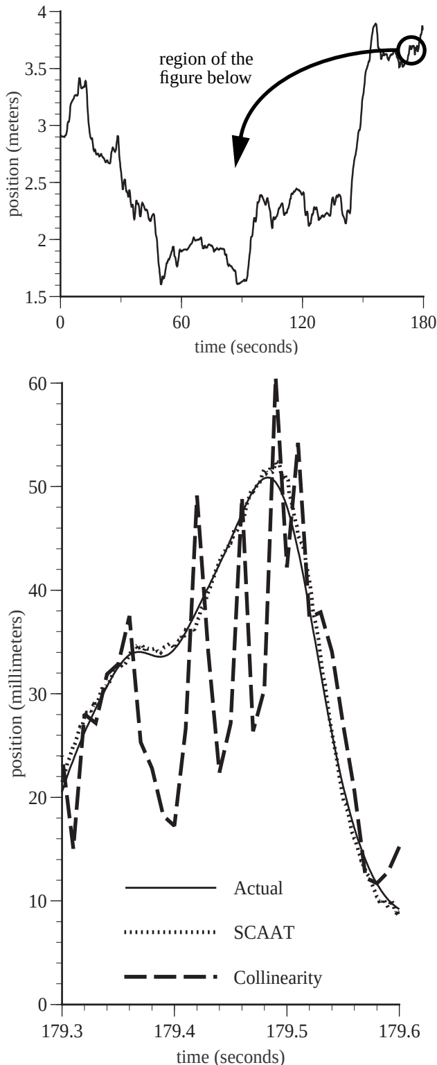
Figure 4: The upper plot depicts the entire 3 minutes of x-axis position data from user motion data set ‘a’ of sets ‘a’-‘f’. The lower plot shows a close-up of a short portion of the simulation. Collinearity here used N = 10 beacons per observation, hence its lower estimate rate. On the other hand, notice that the SCAAT estimates and the actual (truth) data are almost indistinguishable.
