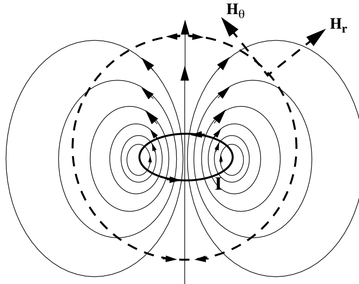
Figure 3.13: Magnetic Dipole
