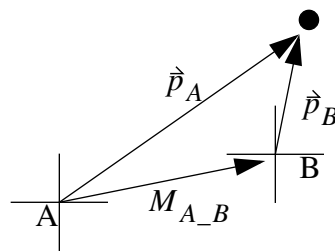
Figure 2.6: Transformation M_{A\_B}
