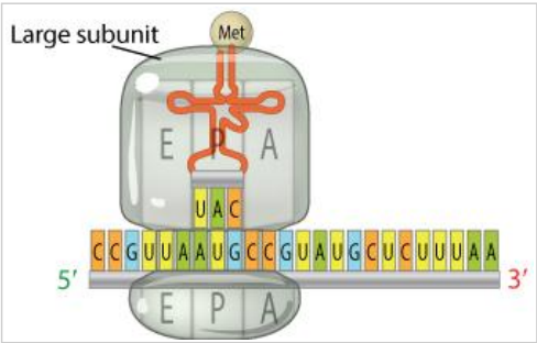
Figure 5: The large ribosomal subunit binds to the small ribosomal subunit to complete the initiation complex. The initiator tRNA molecule, carrying the methionine amino acid that will serve as the first amino acid of the polypeptide chain, is bound to the P site on the ribosome. The A site is aligned with the next codon, which will be bound by the anticodon of the next incoming tRNA. © 2013 Nature Education All rights reserved.
