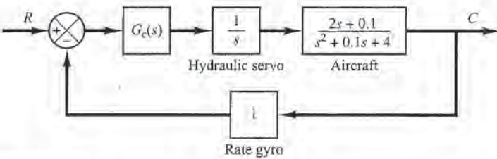
Figure 9-66 Control system.
