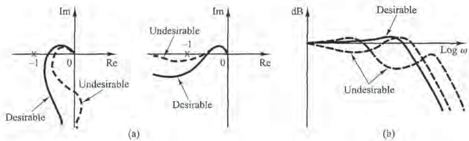
Figure 9-1 (a) Examples of desirable and undesirable open-loop frequency-response curves; (b) examples of desirable and undesirable closed-loop frequency-response curves.
