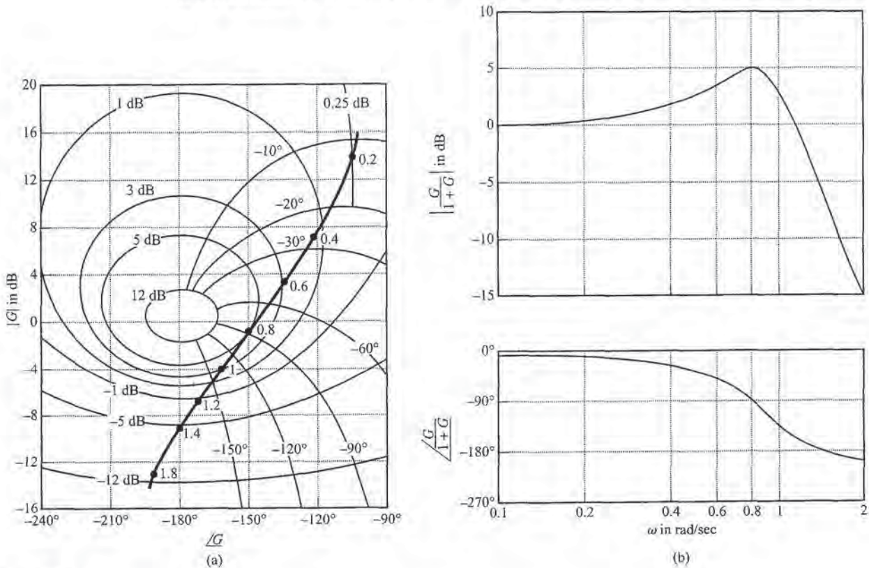
Figure 8–88 (a) Plot of G(j\omega) superimposed on Nichols chart; (b) closed-loop frequency-response curves.
