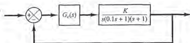
Figure 9-63 Closed-loop system.
