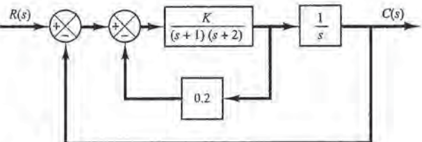
Figure 7-72 Control system.
