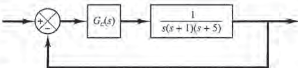
Figure 9-67 Control system.
