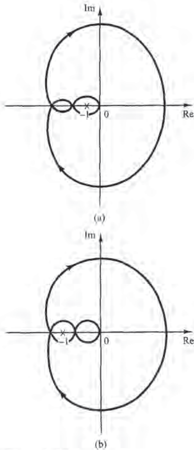
Figure 8-119 Nyquist plots.
