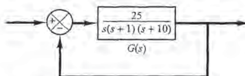
Figure 8-123 Control system.
