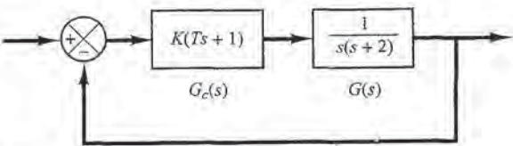
Figure 7-61 Control system.
