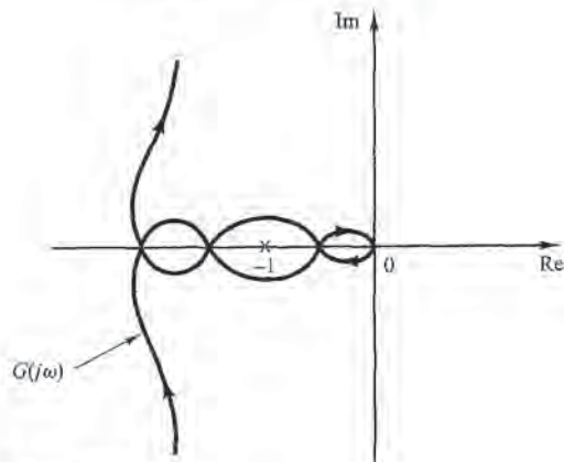
Figure 8-120 Nyquist plot.
