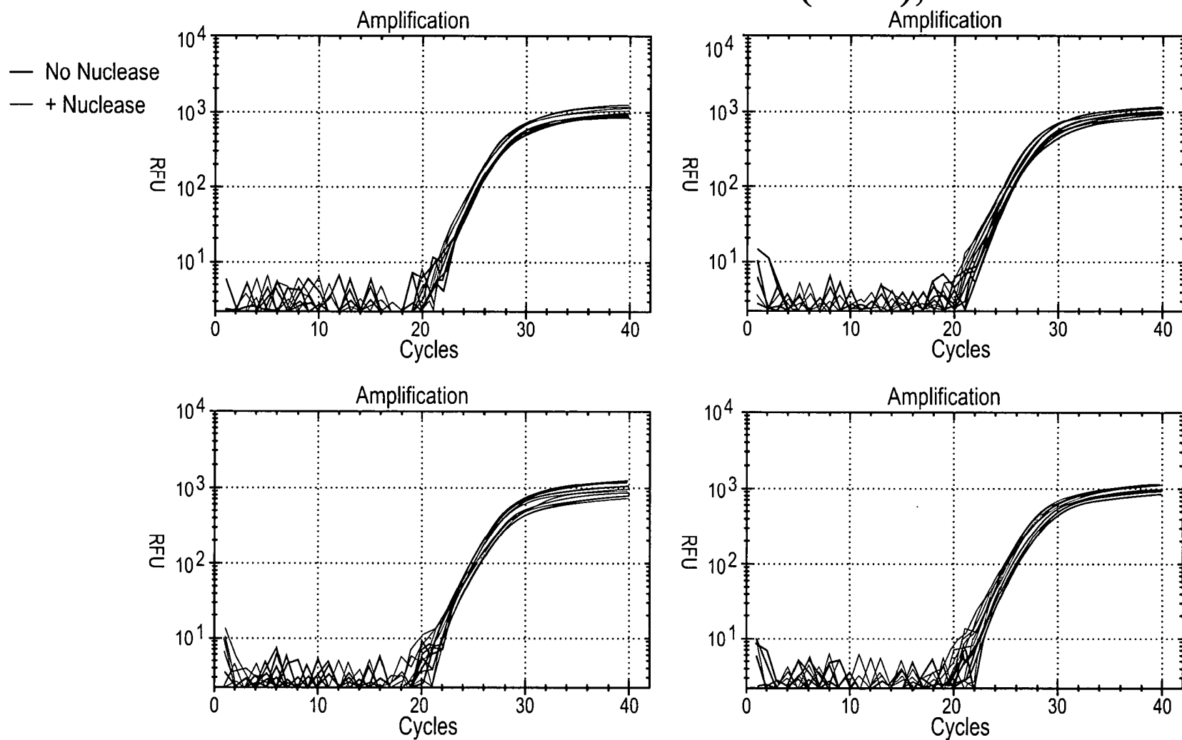
FIG. 18 Reference Gene Control Reactions (HBB), DNase I
