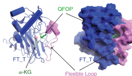
Figure 5. FT enzyme crystal structure. X-ray crystallography was used to solve the structure of FT enzymes (FT T shown in both ribbons and space fill views). The binding of the co-substrates \alpha -KG and QFOP (shown in light and dark green) resulted in an ordering of loops surrounding the active pocket (highlighted in purple) that also contained a metal ion. Cobalt is used to replace the iron atom during crystallization. The view as a monomer is shown for clarity.
