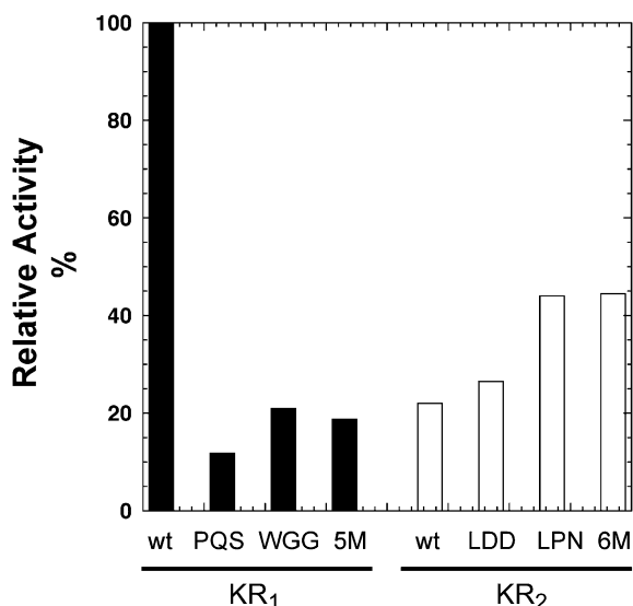
Figure 4. Ketoreductase Activity of Recombinant KR Domains Mutant and wild-type KR domains, purified as their GST fusion proteins, were assayed for NADPH-dependent ketoreductase activity with (2 R , 3 S )-2-methyl-3-oxopentanoic acid NAC ester (IUPAC name: S -2-acetamidoethyl 3-hydroxy-2-methyl-pentanethioate) 1 as substrate.
