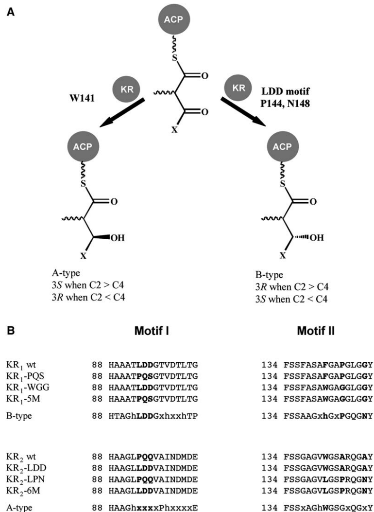
Figure 2. Amino Acid Motifs that Are Putatively Involved in the Control of Stereochemistry by KR Domains from Modular PKSs
