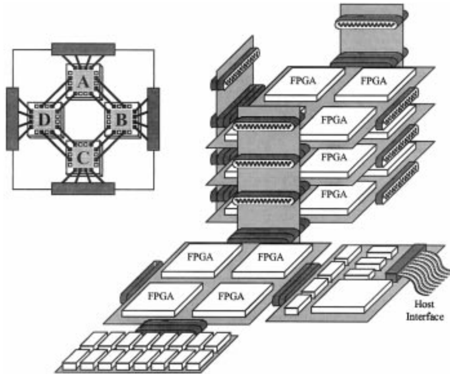
Fig. 24. Base module (upper left) and example topology built in the COBRA system [81]. The mapping includes a tower of three base modules surrounded by three bus modules (top), a base module (center), a RAM module (bottom), and an I/O module (right).
