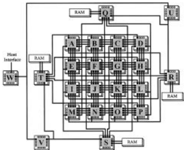
Fig. 17. The DECPerLe-1 topology [133]. The central 4 \times 4 mesh (A-P) is augmented with global buses to four support FPGA's (Q-T), which feed to three other FPGA's (U-W).
