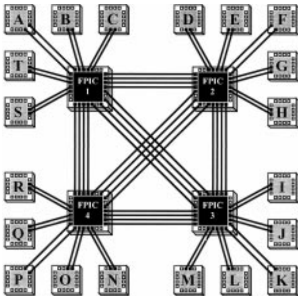
Fig. 14. The Aptix AXB-AP4 topology [9]. Logic-bearing FPGA's are connected only to routing-only FPIC's, but the FPIC's connect to both FPGA's and other FPIC's.
