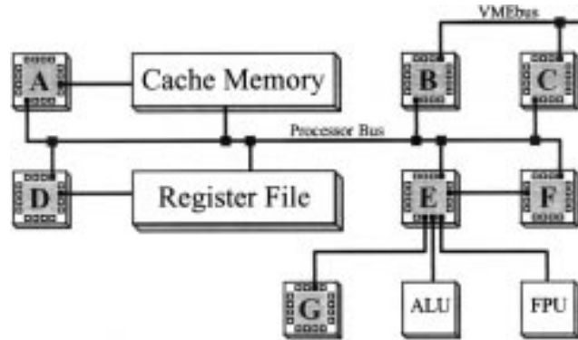
Fig. 20. System similar to the Mushroom processor prototyping system [137].
