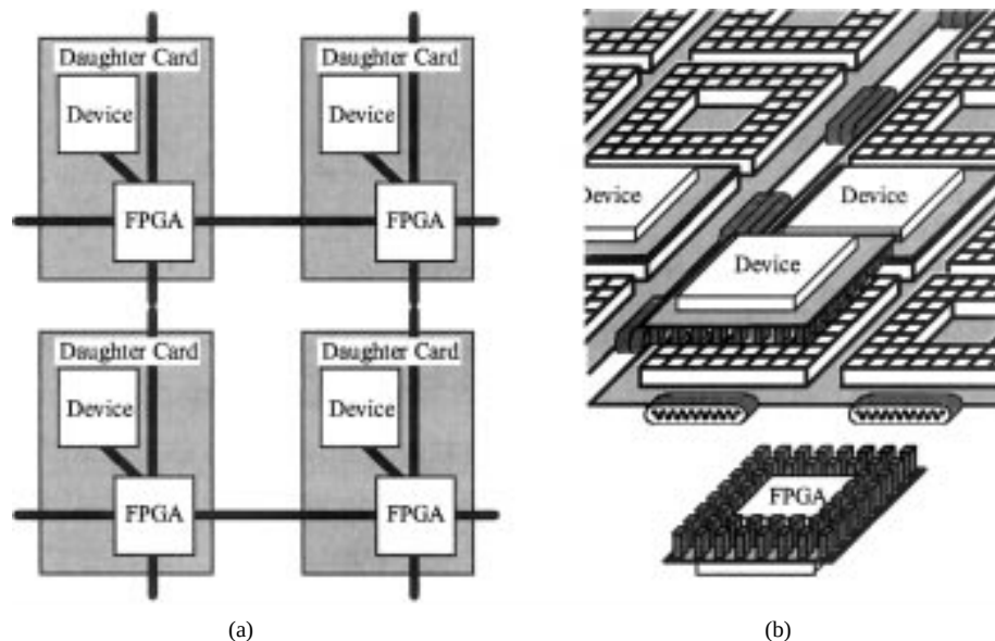
Fig. 25. (a) The Springbok interconnection pattern and (b) two connected Springbok base plates with four daughter cards. The card at front is similar to the other daughter cards (with an FPGA on one side and an arbitrary device on the other) but is shown upside down.
