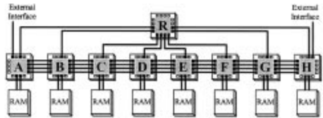
Fig. 15. The Splash 2 topology [10]. The linear array of FPGA's (A-H) is augmented by a routing-only crossbar (R). Note that the real topology has 16 FPGA's in the linear array.
