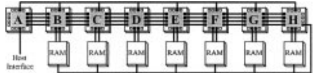
Fig. 16. The Anyboard topology [125], [128]. The linear array of FPGA's is augmented with a global bus.
