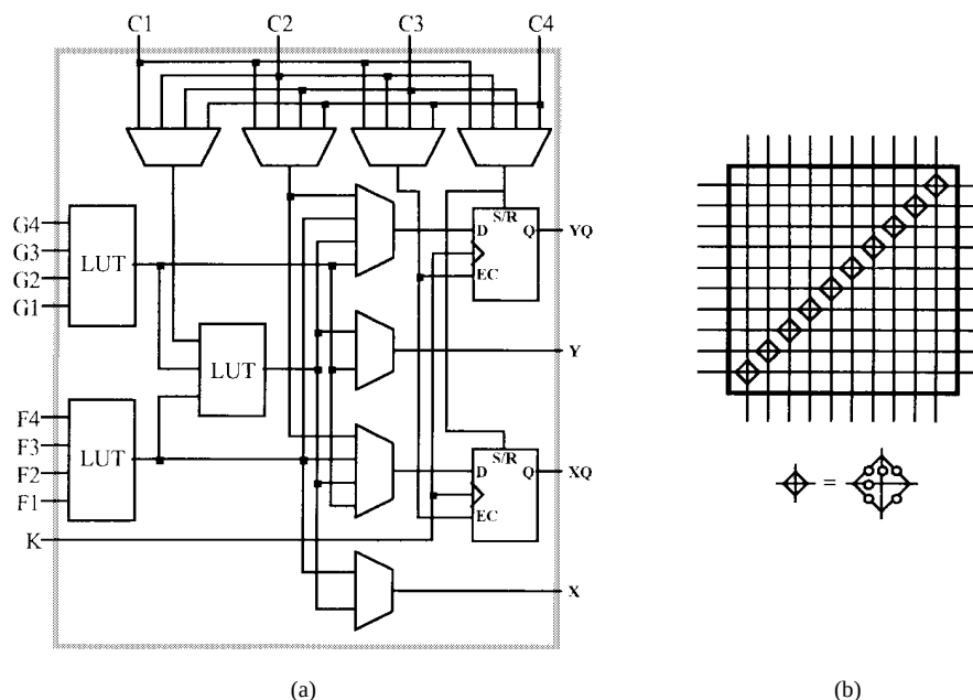
Fig. 6. Details of the Xilinx (a) CLB and [(b), top] switchbox [145]. The multiplexers, LUT's, and latches in the CLB are configured by SRAM bits. Diamonds in the switchbox represent six individual connections [(b), bottom], allowing any permutation of connections among the four signals incident to the diamond.
