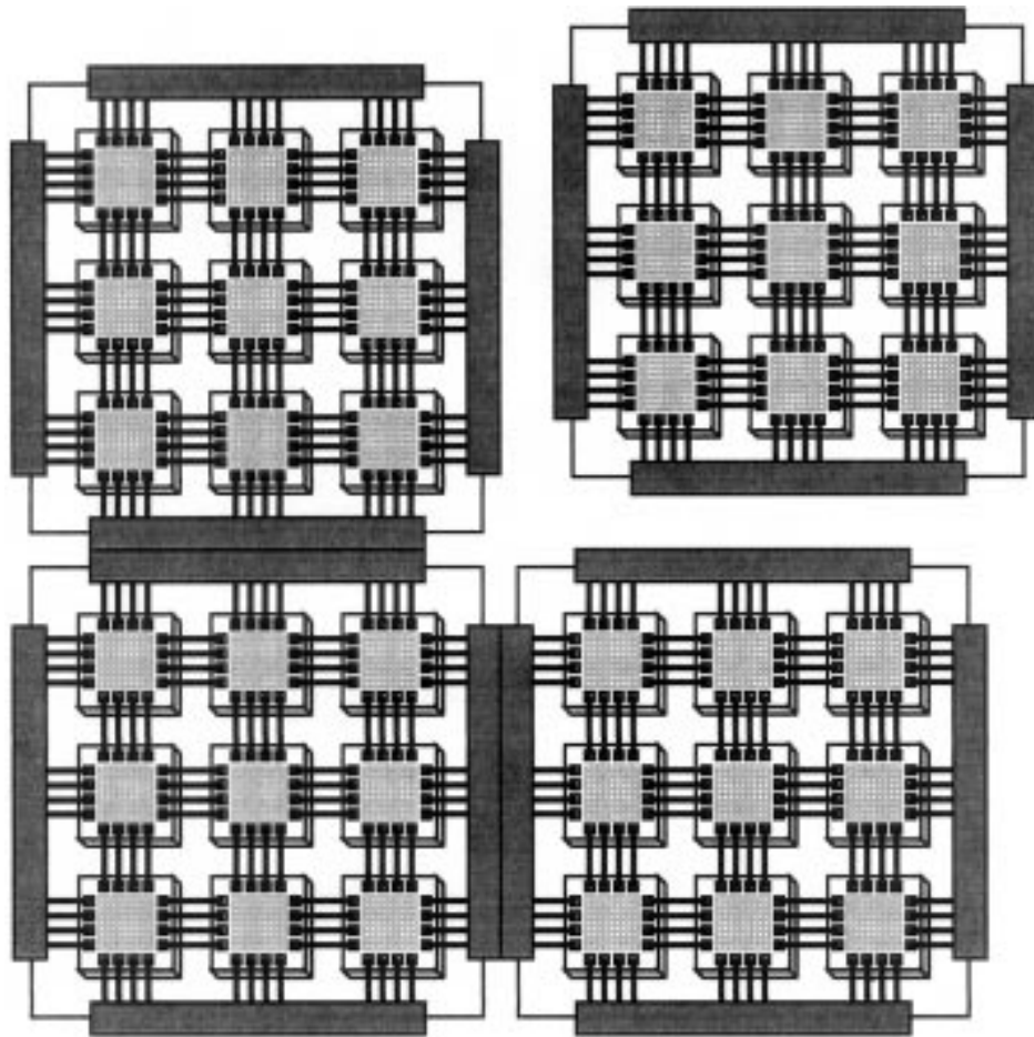
Fig. 21. Expandable mesh topology similar to the Virtual Wires Emulation System [124]. Individual boards are built with edge connectors and limited logic resources and can be interconnected to form a larger mesh.
