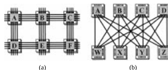
Fig. 12. (a) Mesh and (b) crossbar topologies. In the crossbar, chips A–D are routing only, while W–Z hold all the logic in the system.
