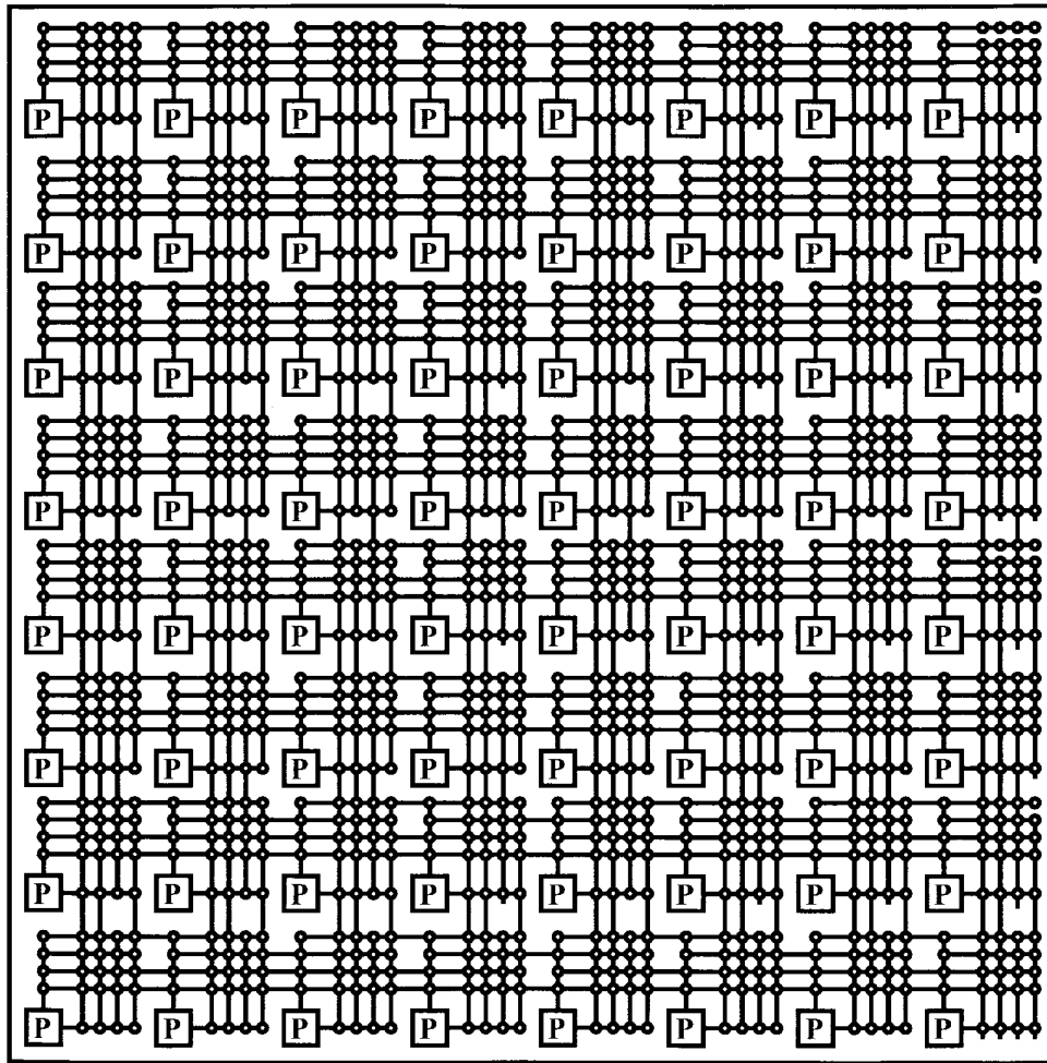
Fig. 10. The Aptix FPIC architecture [8]. The boxed “P” indicates an I/O pin.
