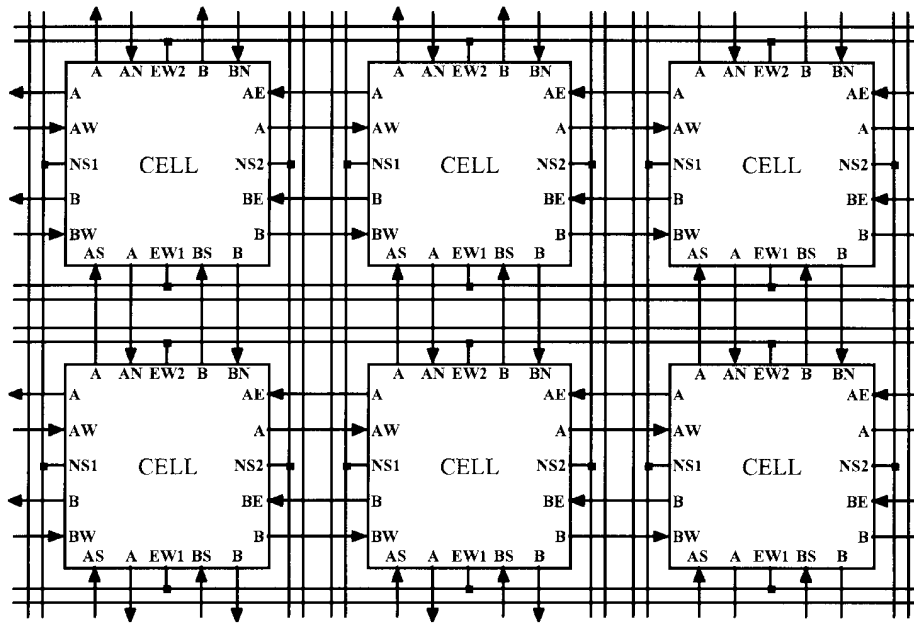
Fig. 8. Details of the CLi routing architecture [75].
