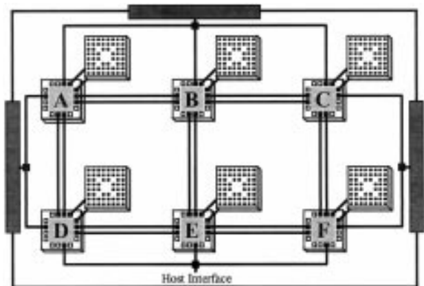
Fig. 22. The MORRPH topology [38]. Sockets next to the FPGA's allow arbitrary devices to be added to the array. Buses connected to external connectors allow multiple boards to be hooked together to build an arbitrarily large system.
