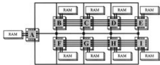
Fig. 19. The RM-nc system [42]. The linear arrays can be grown larger than the system shown.
