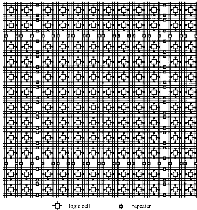
Fig. 7. The CLi6000 routing architecture [75]. One 8 \times 8 tile, plus a few surrounding rows and columns, is shown. The full array has many of these tiles abutted horizontally and vertically.
