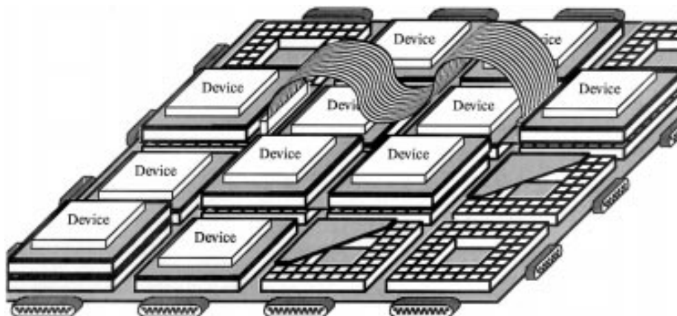
Fig. 26. Nondevice daughter cards and extender cards, including cards to add more FPGA logic (lower left), bandwidth (double-sized card in the second row), long-distance communication (third row), and edge bandwidth (two cards at front right). All but the edge bandwidth cards have FPGA's on the bottom.
