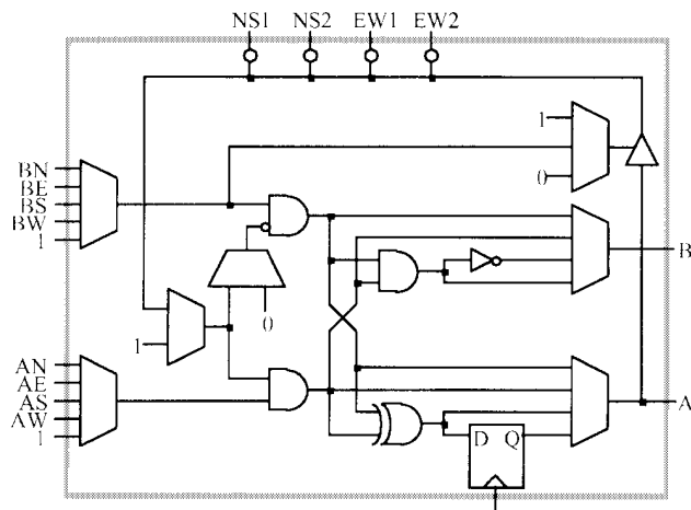
Fig. 9. The CLi logic cell [75].
