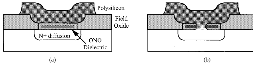
Fig. 1. Actel's programmable low-impedance circuit element (PLICE). As shown in (a), an unblown antifuse has an oxide-nitride-oxide (ONO) dielectric preventing current from flowing between diffusion and polysilicon. The antifuse can be blown by applying a 16-V pulse across the dielectric. This melts the dielectric, allowing a conducting channel to be formed (b). Current is then free to flow between the diffusion and the polysilicon [1], [54].
