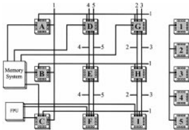
Fig. 18. The Marc-1 topology [86]. The complete topology consists of two copies of the left subsystem (A–I, Memory, and FPU) and one copy of the right (1–5). Numbers by themselves indicate connections to the FPGA's at right.
