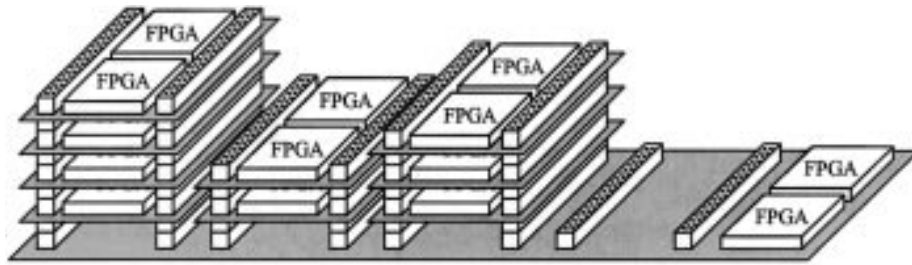
Fig. 23. The G800 board [49]. The base board has two FPGA's and four sockets. The socket at left holds four computing module boards (the maximum allowed in a socket), while the socket at right has none.
