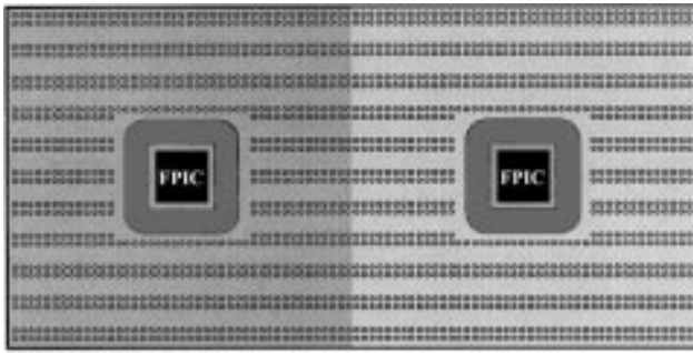
Fig. 27. The Aptix FPCB. Holes in each of the two shaded regions are connected to the corresponding FPIC.
