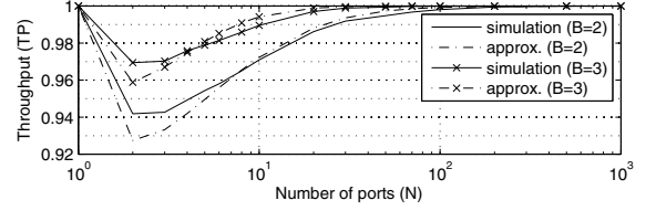
Fig. 6. Throughput of the exhaustive round-robin scheduling algorithm.
