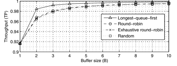
Fig. 2. Throughput of a 32 \times 32 CQ switch under uniform traffic
