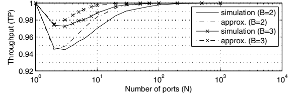
Fig. 5. Throughput of the random scheduling algorithm.
