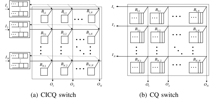
Fig. 1. Illustration of the CICQ and CQ switch architectures, with inputs I_i , outputs O_j , and crosspoint buffers B_{i,j} . In the CICQ switch, the dashed lines represent the communication between the linecards and the buffers.
