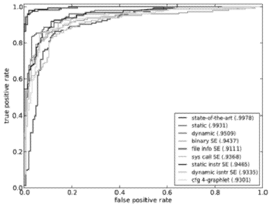
(a) Full ROC Image
