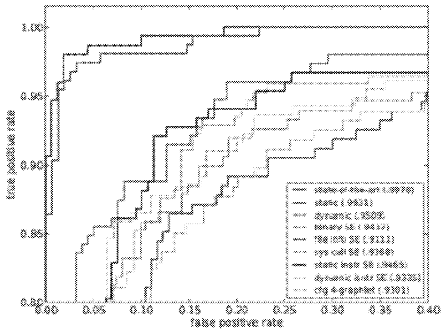
(b) Zoomed ROC Image
