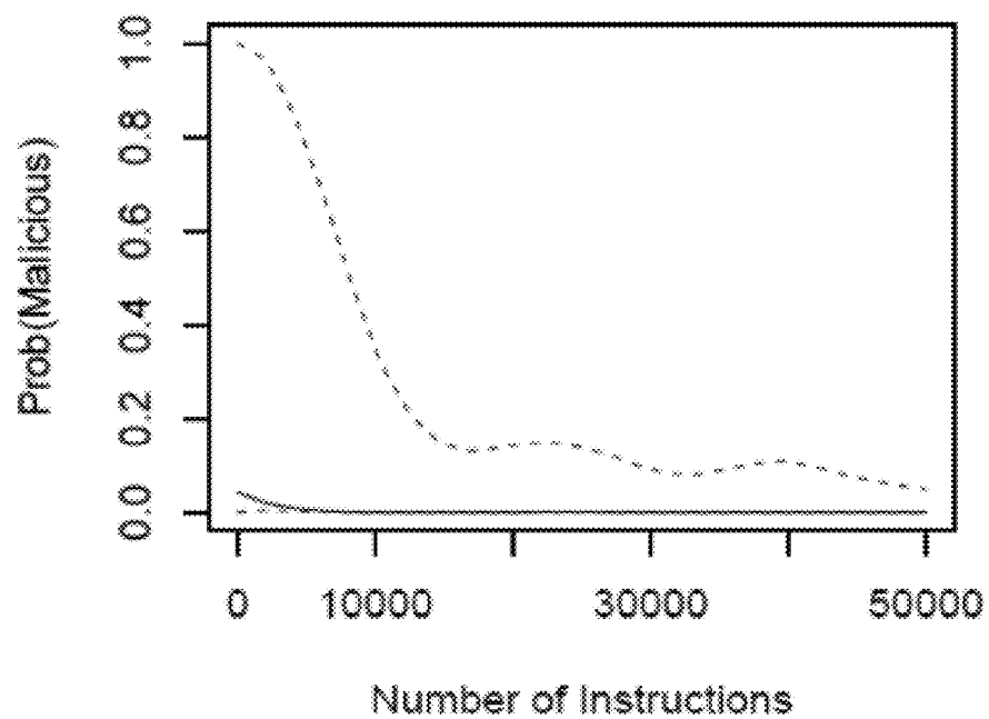
(b) Dynamic trace from a benign program
