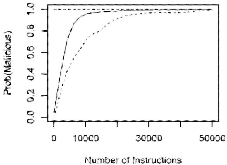
(a) Dynamic trace from a malicious program
