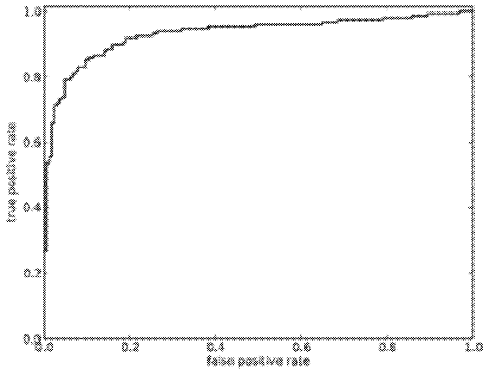
(a) Binary SE
