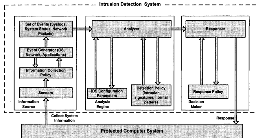
Figure 2.2: Component details of an IDS
