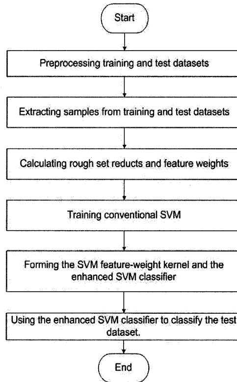
Figure 4.1: Enhanced SVM model for intrusion detection
