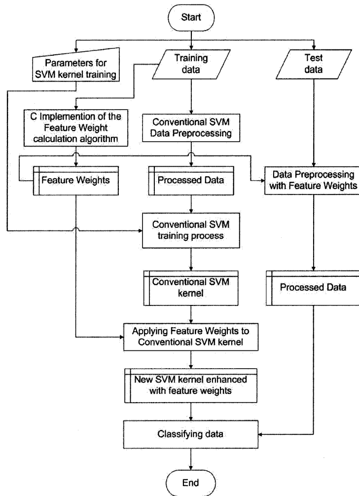
Figure 3.1: Flowchart of the modified SVMLight
