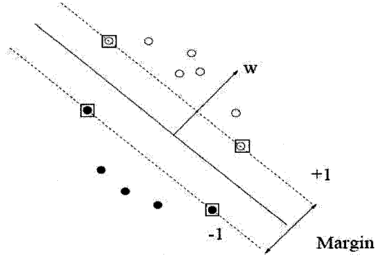
Figure 2.4: Decision plane for a linear separable dataset [7]
