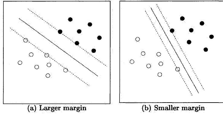
Figure 2.3: Hyperplanes with different margins [7]
