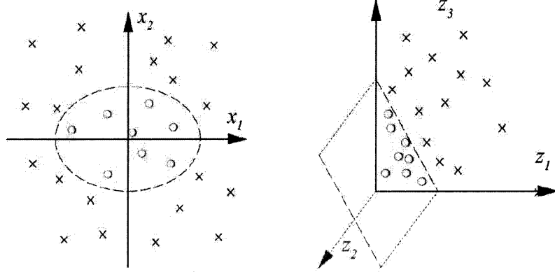
Figure 2.5: SVM data transforming between space \Phi and space H [7]
