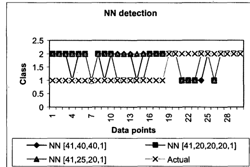
Fig. 3. Neural network testing on KDD intrusion detection
