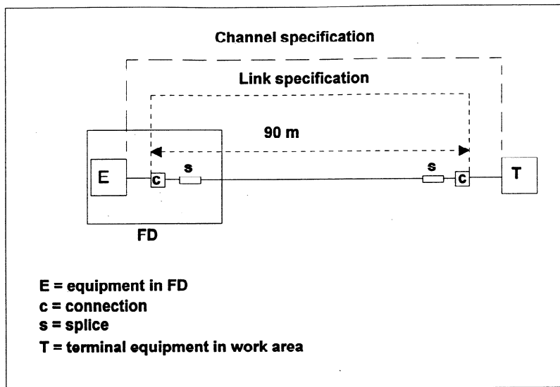
Figure 7b - Horizontal cabling model - fibre
