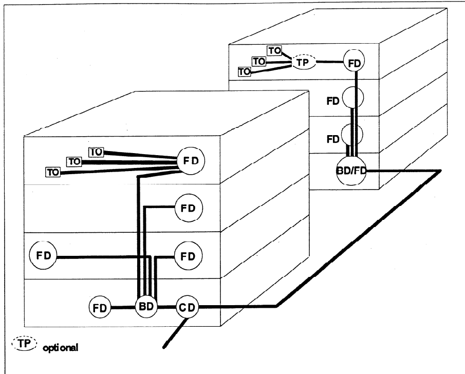
Figure 3 - Example of the generic cabling system
