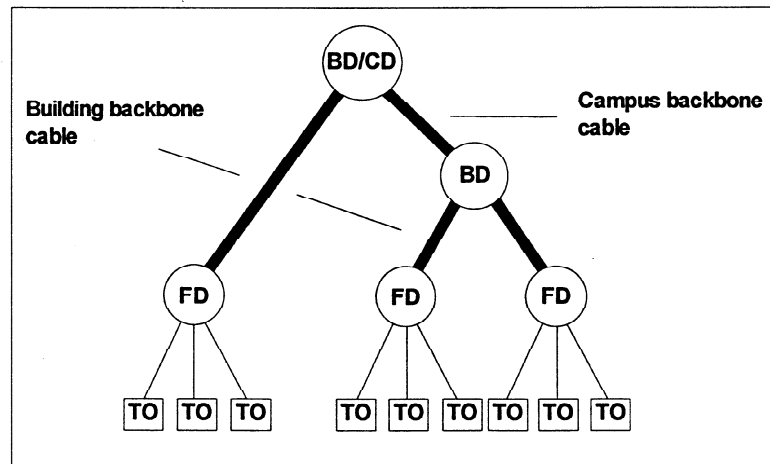
Figure 9 - Backbone star topology
