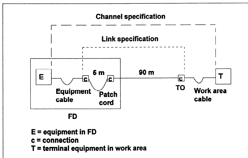
Figure 7a - Horizontal cabling model - copper
