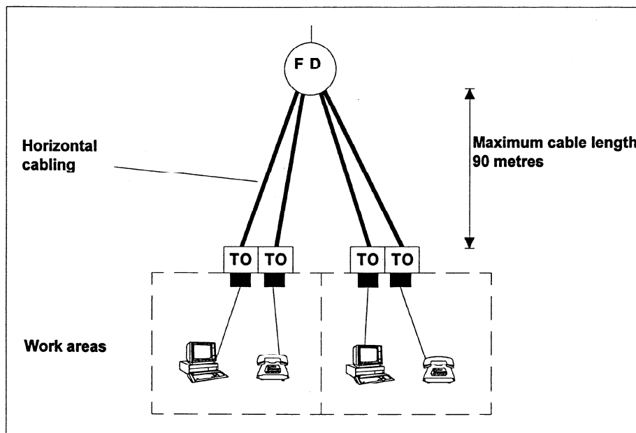
Figure 8 - Typical horizontal and work area cabling
