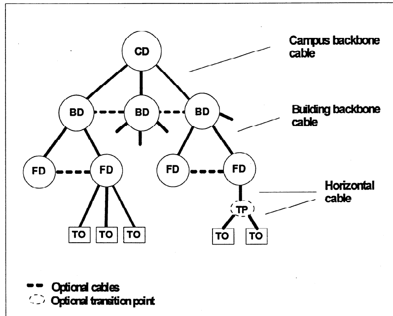
Figure 2 - Inter-relationship of functional elements
