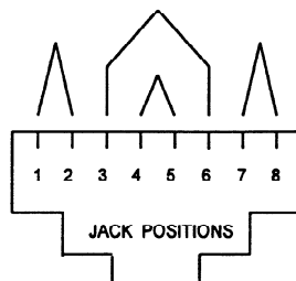
Figure 12 - Eight position jack pin and pair grouping assignments (This illustration is a front view of the connector.)
