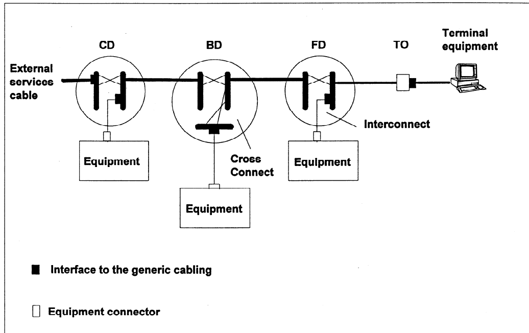
Figure 5 - Potential interfaces to generic cabling
