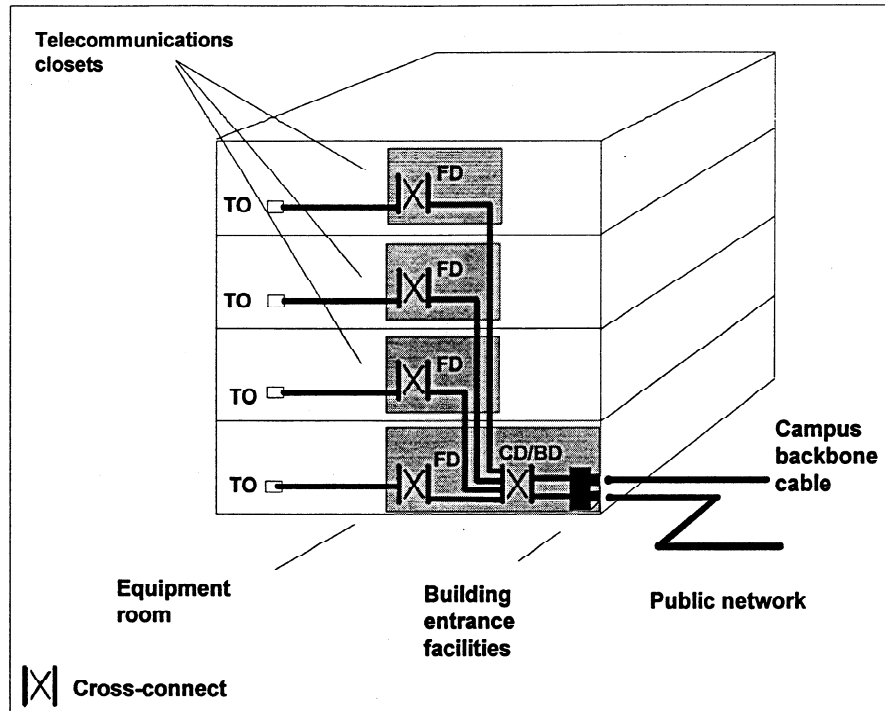
Figure 4 - Typical accommodation of functional elements
