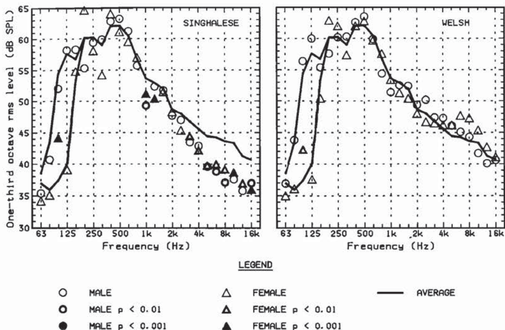
FIG. 4. Male and female LTASS values for Singalese and Welsh. Solid line shows LTASS average across 17 speech samples.
