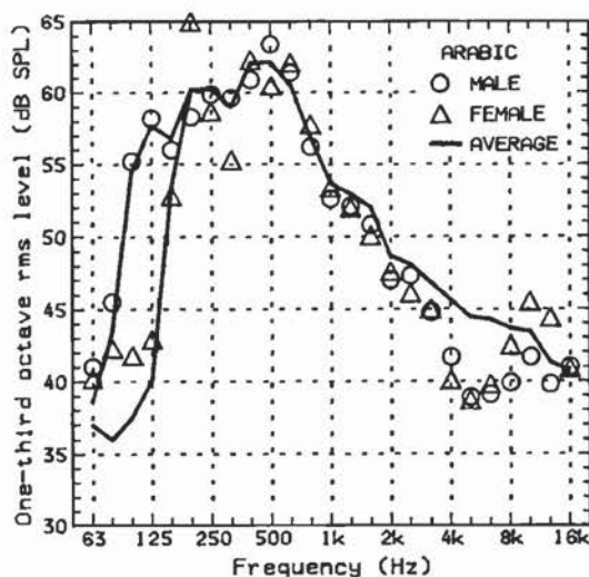
FIG. 9. Male and female long-term average speech spectrum for Arabic. Solid line shows LTASS averaged across the other 17 samples (i.e., excluding Arabic).
