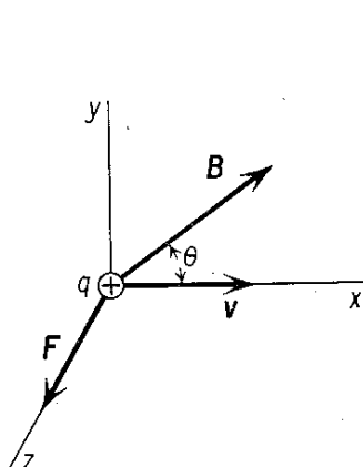
Fig. 31-1 The force \mathbf{F} exerted on a charge q moving with velocity \mathbf{v} in a magnetic field of induction \mathbf{B} . \mathbf{B} and \mathbf{v} are in the x - y plane; \mathbf{F} is along the z axis.
