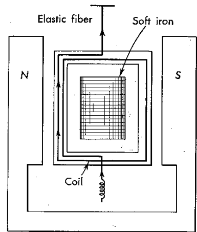
Fig. 31-10 Essentials of a D'Arsonval type of galvanometer. The soft iron core is introduced to shape the magnetic field so that it is radial, thus obtaining a galvanometer in which the deflection is proportional to the current through the coil.
