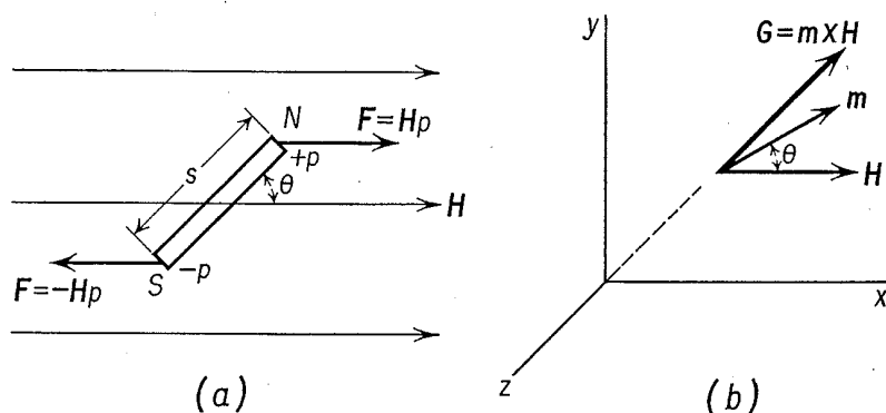
Fig. 29-7 (a) Forces on a bar magnet in a uniform magnetic field. The plane of the paper is the x - y plane. (b) When the magnetic moment vector \mathbf{m} and the magnetic field \mathbf{H} lie in the x - y plane as shown, the torque \mathbf{G} on the magnet is parallel to the z axis.
