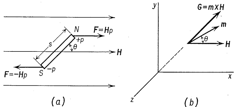
Fig. 29-7 (a) Forces on a bar magnet in a uniform magnetic field. The plane of the paper is the x - y plane. (b) When the magnetic moment vector m and the magnetic field H lie in the x - y plane as shown, the torque G on the magnet is parallel to the z axis.
