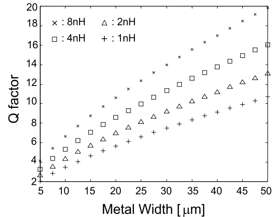
Fig. 3. The dependence of Q_{ind} on the metal width W where \omega = 2 GHz, S = 1 \mu\text{m} , D_i = 50 \mu\text{m} , and \rho_{sh} = 40 m \Omega/\square .
