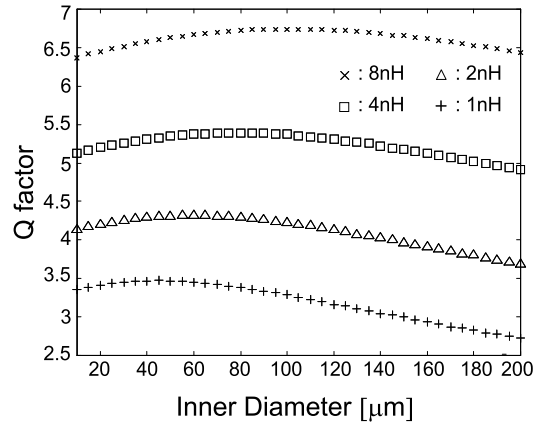
Fig. 4. The dependence of Q_{ind} on the inner-diameter D_i where \omega = 2 GHz, S = 1 \mu\text{m} , W = 10 \mu\text{m} , and \rho_{sh} = 40 m \Omega/\square .
