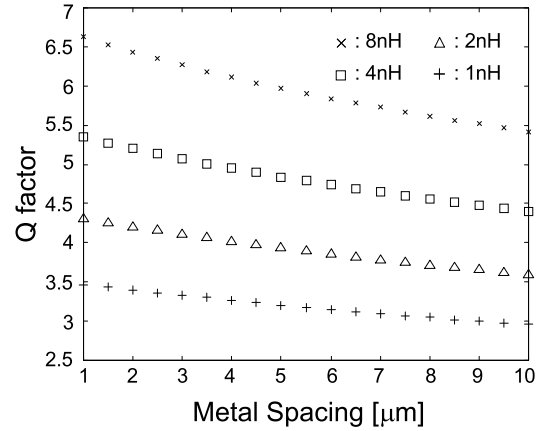
Fig. 2. The dependence of Q_{ind} on the metal spacing S where \omega = 2 GHz, W = 10 \mu\text{m} , D_i = 50 \mu\text{m} , and \rho_{sh} = 40 m \Omega/\square .
