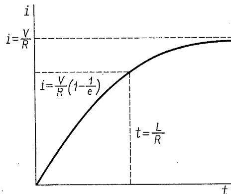
Fig. 32-13 Growth of current in a circuit containing inductance and resistance.
