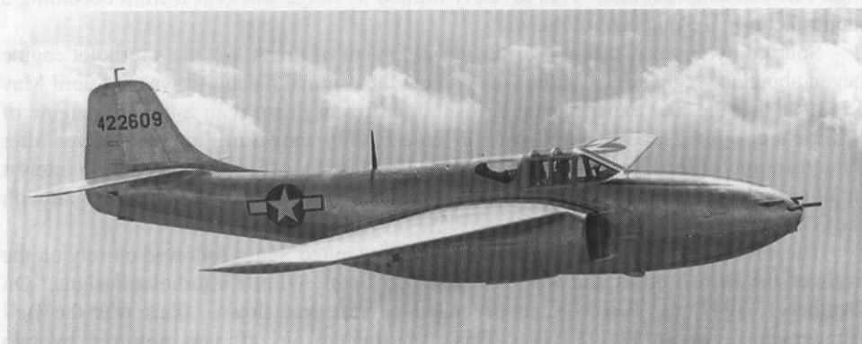
Figure 2.1.10. The first U.S. jet aircraft was the Bell Airacomet, powered by two GE 1-A engines each weighing 1,000 pounds and developing 1,250 pounds of thrust. (U.S. Air Force)
