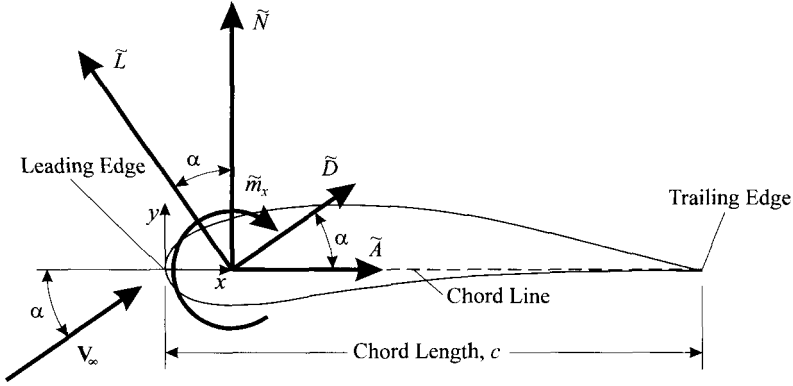
Figure 1.1.2. Section forces and moment.
