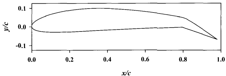
Figure 1.7.1. NACA 4412 airfoil section with a 20 percent trailing-edge flap.
