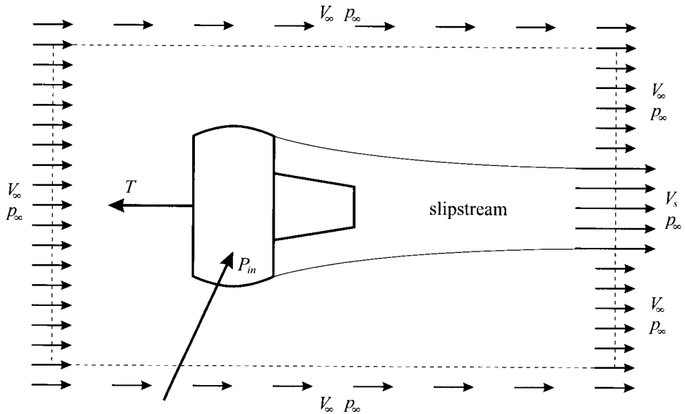
Figure 2.1.1. Schematic diagram of a control volume surrounding an ideal propulsion system.
