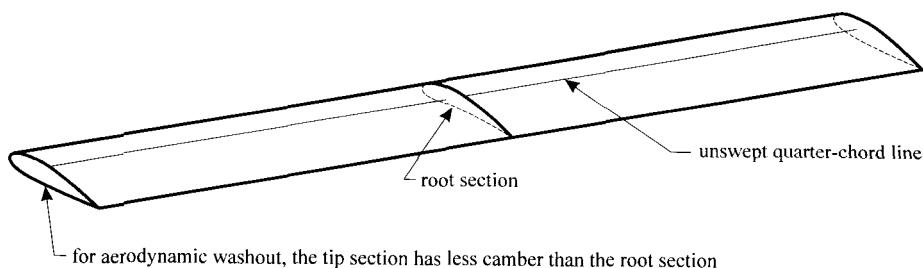
Figure 1.8.8. Aerodynamic twist in an unswept rectangular wing.
