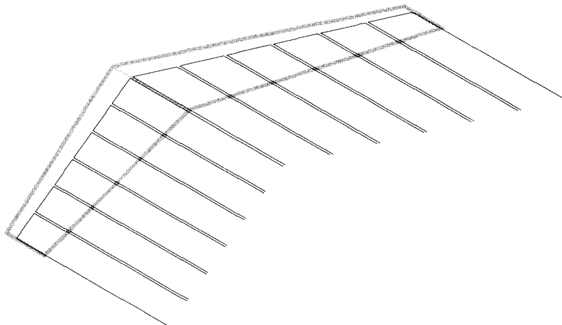
Figure 1.9.2. Horseshoe-shaped vortices distributed along the lifting line of a finite wing with sweep and dihedral.
