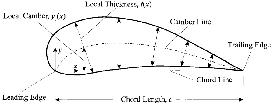
Figure 1.6.1. Airfoil coordinates and nomenclature.
