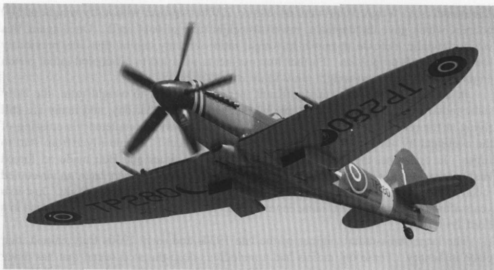
Figure 2.1.5. The early Spitfire Mark XVIII was powered by a liquid-cooled, 12-cylinder, Rolls-Royce Griffon engine that weighed 2,050 pounds, developed 2,035 horsepower, and provided a power-to-weight ratio of almost 1.0 hp/lb. (Photograph by Barry Santana)
