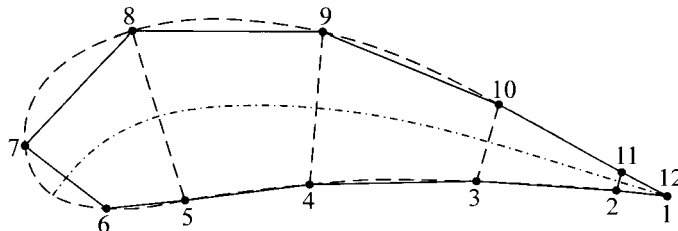
Figure 1.6.4. Vortex panel distribution with cosine clustering and an even number of nodes.
