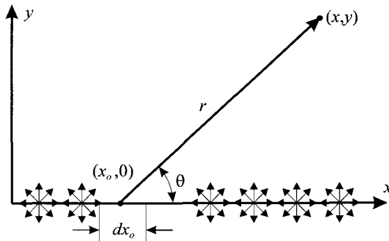
Figure 1.5.2. Edge view of a 2-D source panel on the x -axis.
