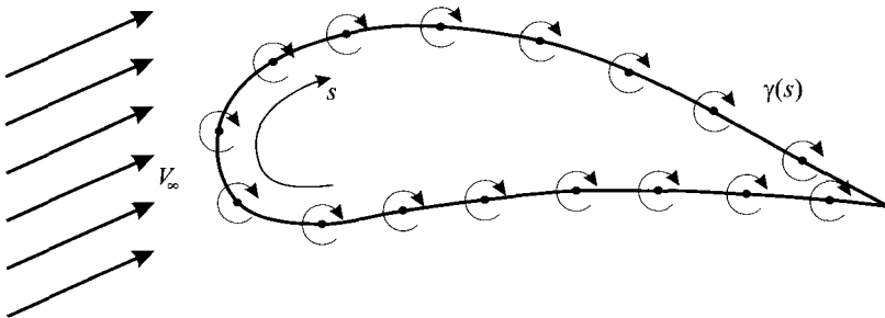
Figure 1.6.3. Synthesis of an arbitrary airfoil section from a uniform flow and a vortex sheet.
