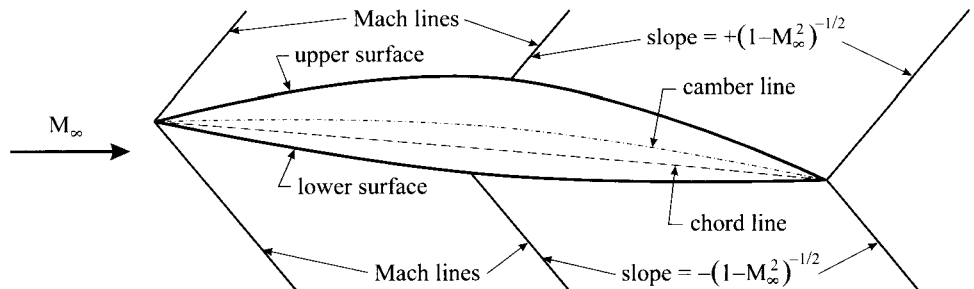
Figure 1.12.1. Small-angle supersonic potential flow over an airfoil.
