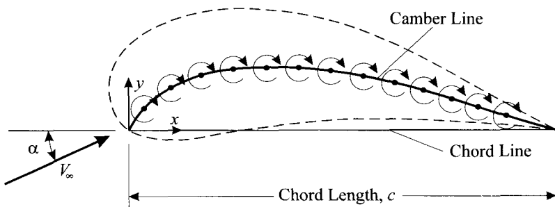
Figure 1.6.2. Synthesis of a thin airfoil section from a uniform flow and a curved vortex sheet distributed along the camber line.
