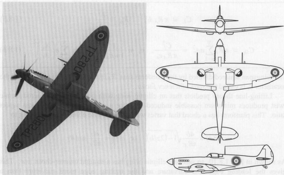
Figure 1.8.11. Elliptic wing used on the famous British Spitfire. (Photograph by Barry Santana)
