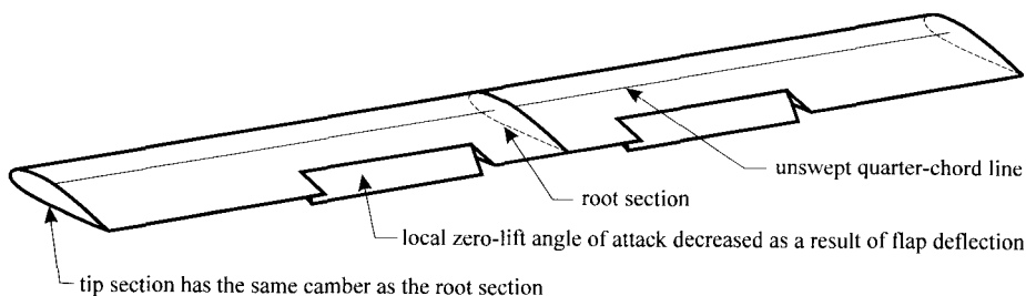
Figure 1.8.9. Aerodynamic twist resulting from deflection of a trailing-edge flap spanning only a portion of the wing.
