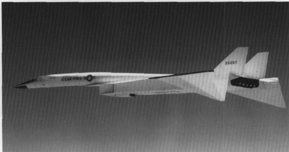
Figure 2.1.13. The North American XB-70 reached Mach 3 powered by six General Electric YJ-93 turbojet engines that each delivered 30,000 pounds of thrust with afterburners employed. (U.S. Air Force)
