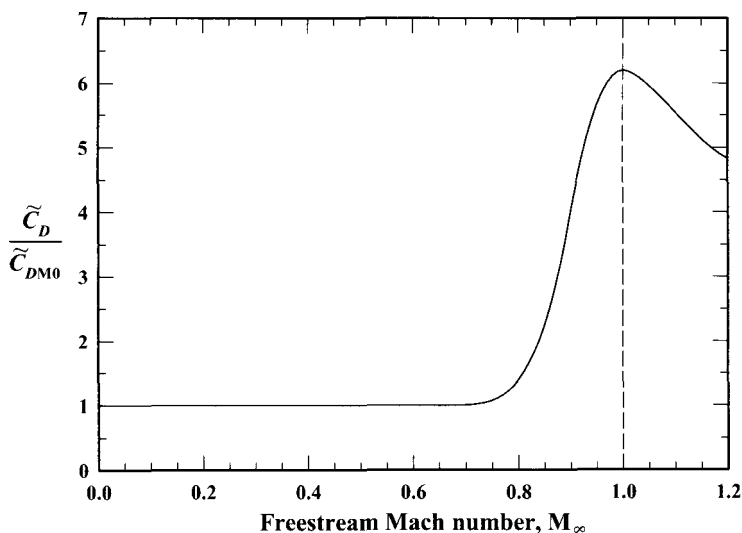
Figure 1.11.1. Sketch of typical variation in section drag coefficient with Mach number.
