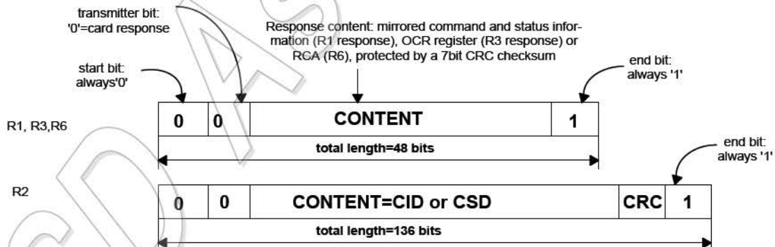
Figure 3-8: Response Token Format
