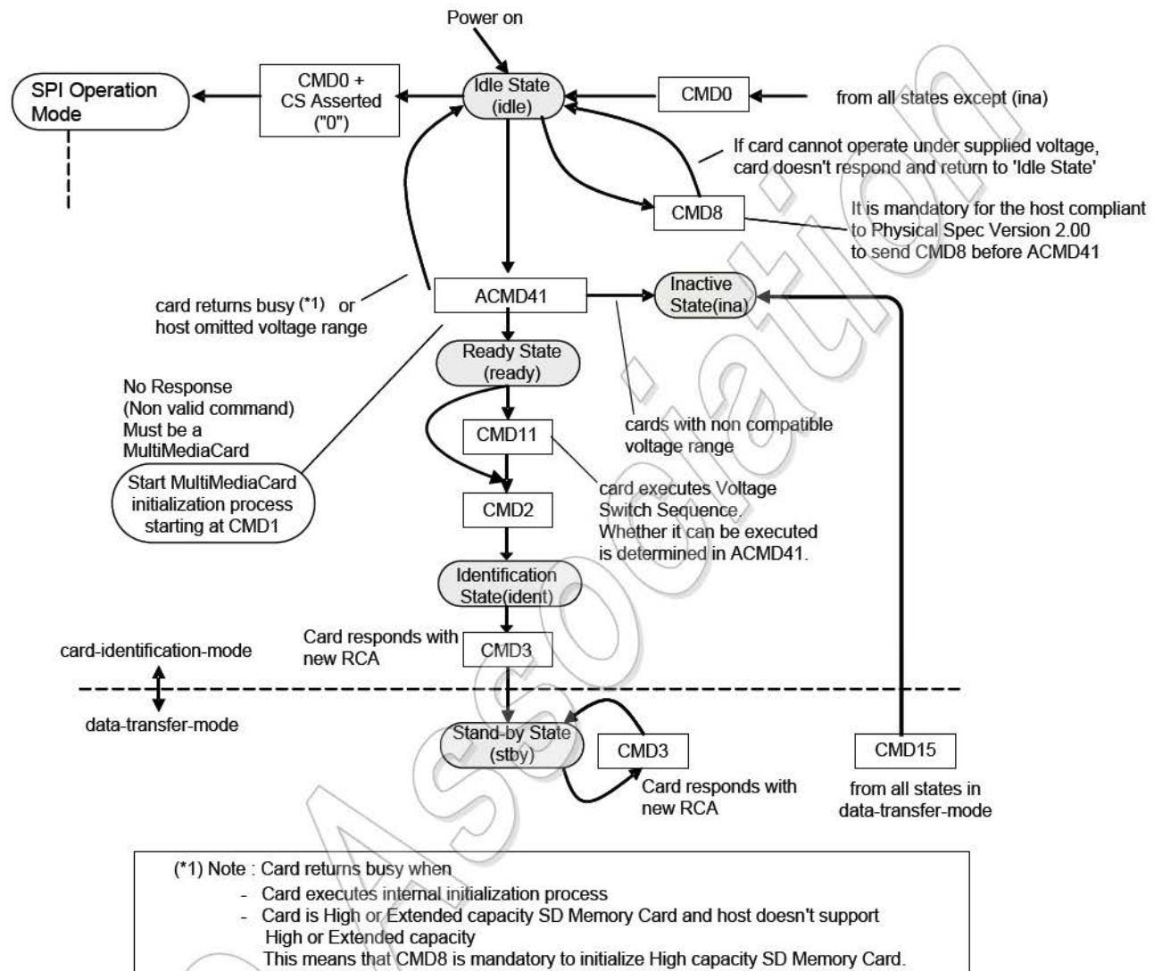
Figure 4-1 shows State Diagram of card Identification mode for SD I/F. In case of UHS-II mode, refer to SD-TRAN Section of the UHS-II Addendum.
