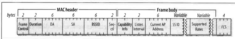
Figure 4-45. Reassociation Request frame
