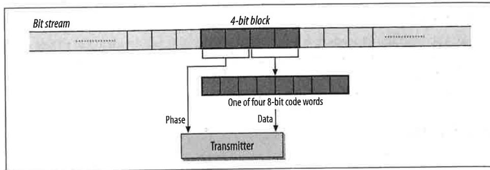
Figure 10-29. 802.11b transmission at 5.5 Mbps
