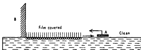
Fig 19-11. Insoluble monomolecular film compressed between a fixed barrier, B, and a movable barrier, A. 6
