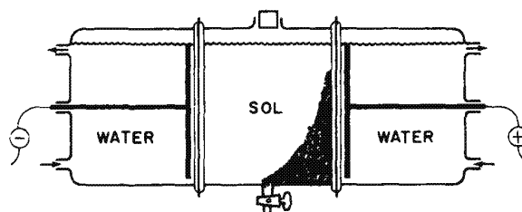
Fig 19-21. Electrodialyzer showing electrodecentration
