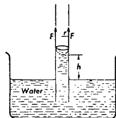
Fig 19-6. Capillary rise for a liquid exhibiting zero contact angle. 1
