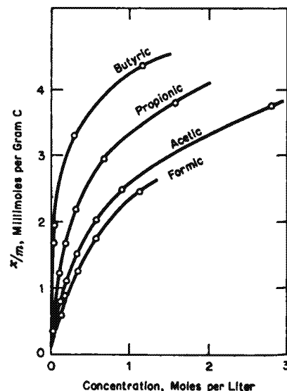
Fig 19-15. The relation between adsorption and molecular weight for fatty acids. 9
