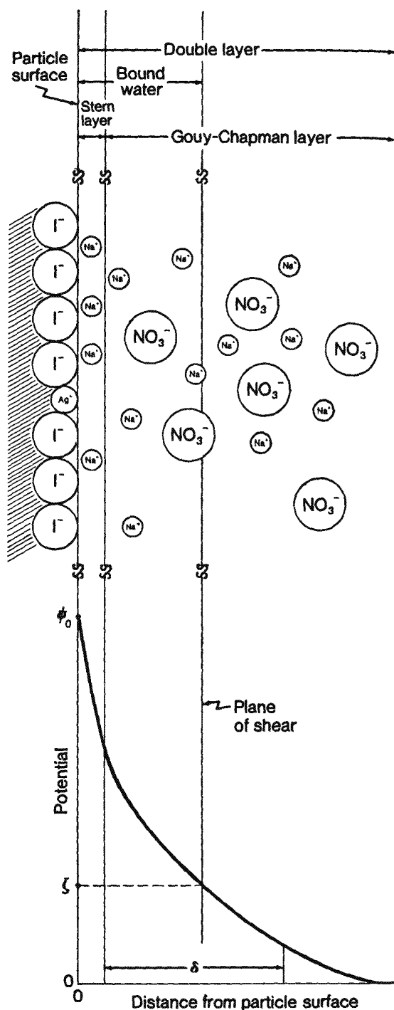
Fig 19-28. Electric double layer at the surface of a silver iodide particle (upper part) and the corresponding potentials (lower part). The distance from the particle surface, plotted on the horizontal axis, refers to both the upper and lower parts.
