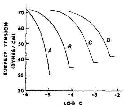
Fig 19-13. The effect of increasing chain length on the surface activity of a surfactant at the air-aqueous solution interface (each figure depicted to differ by two methylene groups with A, the longest chain, and D, the shortest).
