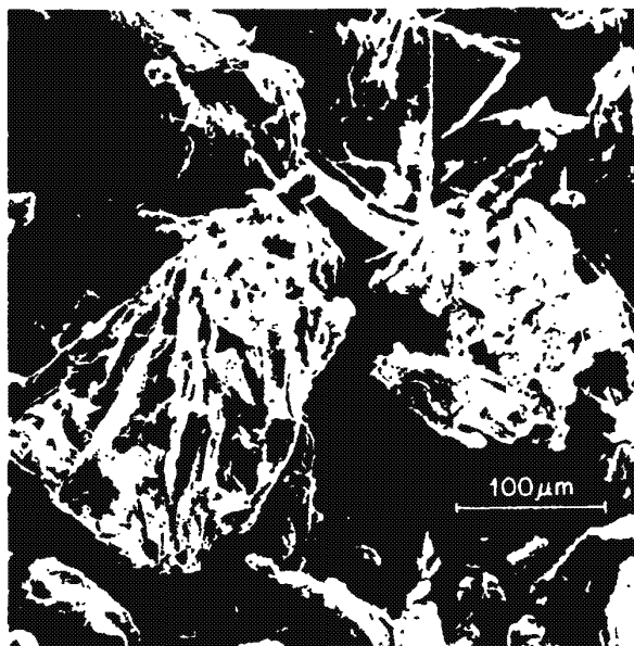
Fig 19-24. Scanning electron micrograph of Avicel PH-102 tabletting grade microcrystalline cellulose. The aggregates of fiber bundles are porous and compressible (courtesy, FMC Corporation; Avicel is a registered trademark of FMC Corporation).
