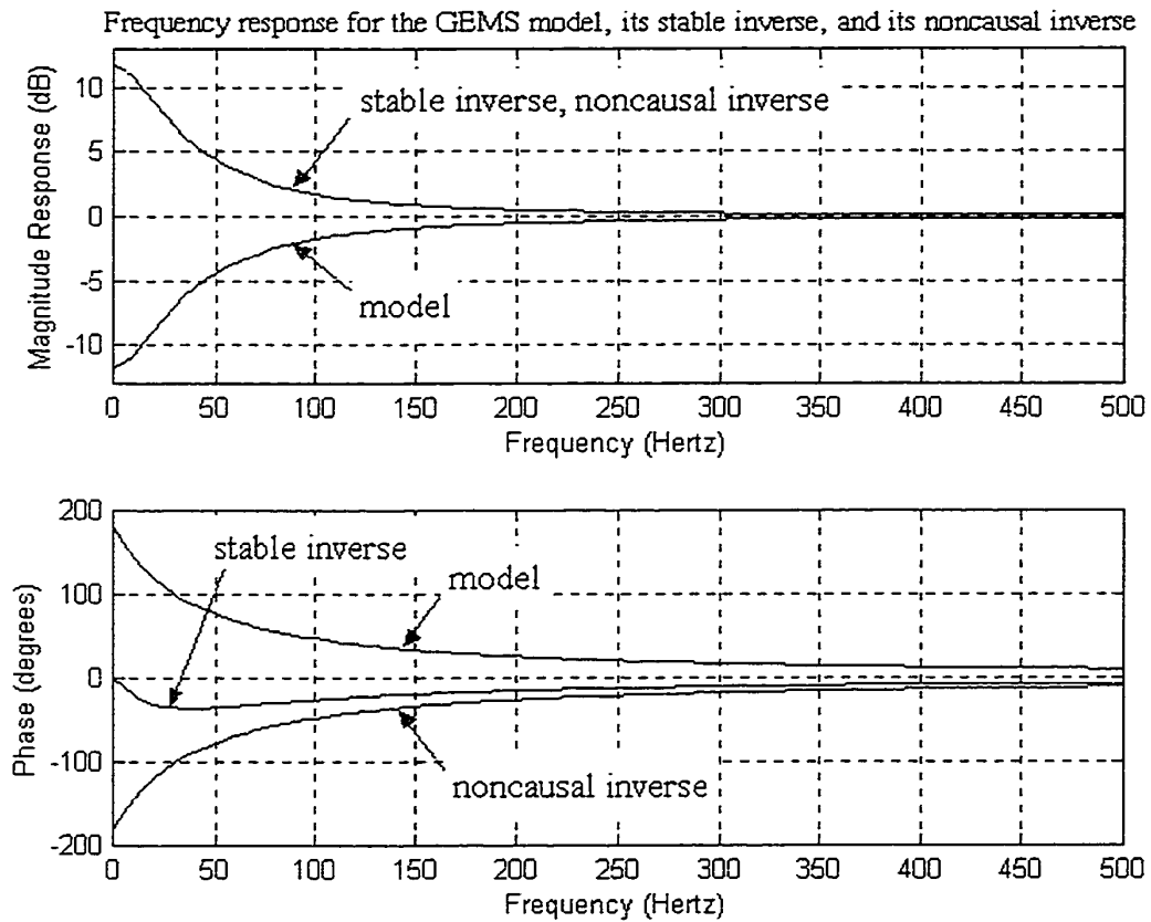
Figure 2.9. Magnitude and phase response for the GEMS, its stable inverse, and its noncausal inverse.
