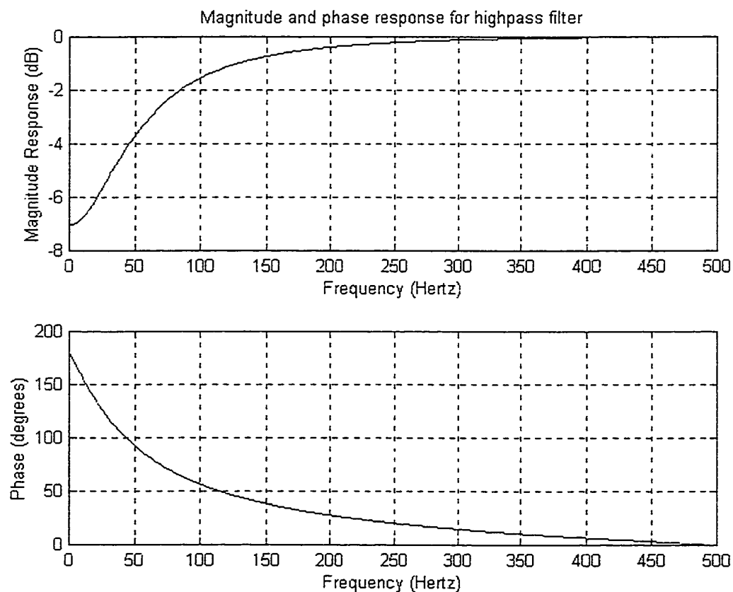
Figure A.1. Normalized frequency response for the example highpass filter.
