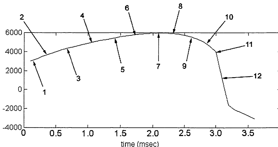
Figure 3.10. Approximate locations on the GEMS return for the frames analysis.
