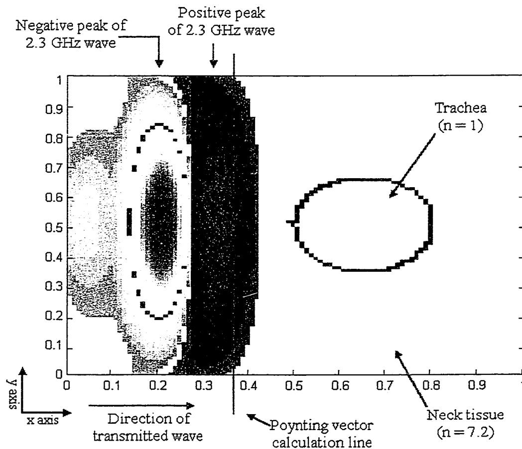
Figure 3.4. Frame from tracheal reflectivity simulation with 2.3 GHz wave. The frame is slightly stretched in the x direction due to machine graphics incompatibilities.
