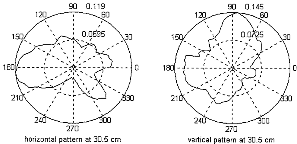
Figure 2.6. Measured antenna patterns for the GEMS antennae at 30.5 cm in Volts.
