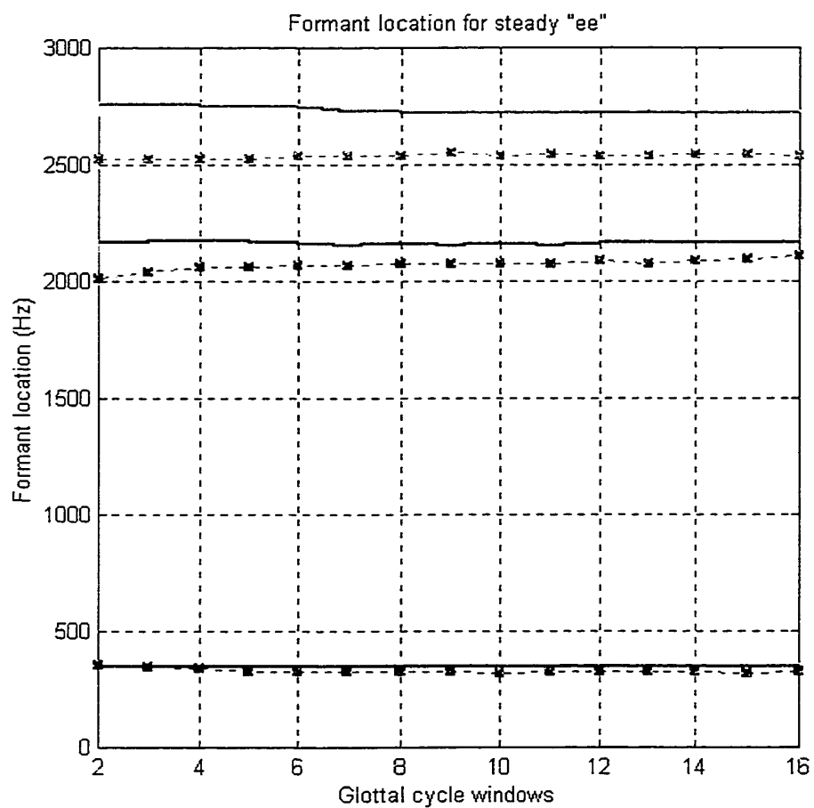
Figure 4.14. Formant location trend for /i/ for subjects GB and TG.
