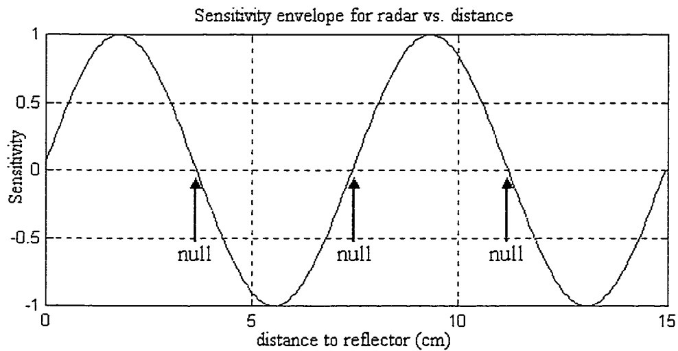
Figure 2.3. Theoretical sensitivity envelope for the radar as a function of distance away from the antennae assuming n_2 > n_1 reflection and a 15 cm wavelength.
