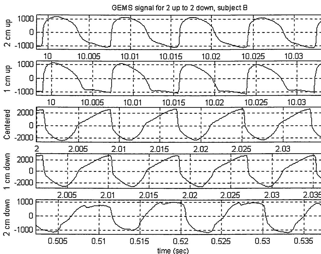
Figure 3.19. Data from position experiments when the GEMS is moved from 2 cm above the laryngeal prominence to 2 cm below it. Note the phase change from the positions above to the center.
