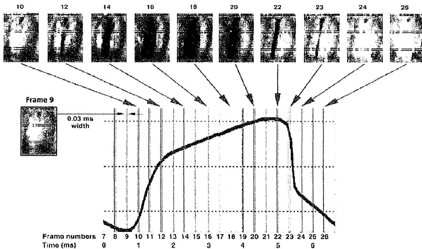
Figure C.3. GEMS signal overlaid with the corresponding high-speed vocal fold video frames. Each bar is 30 microseconds wide and represents the exposure time of the frame.
