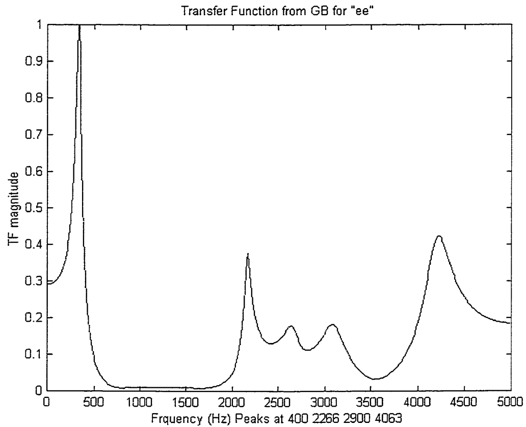
Figure 4.11. Calculated transfer function for /i/, subject GB. The first two formant locations are at 400 and 2266 Hz, normal locations are 200-400 and 2000-4000.
