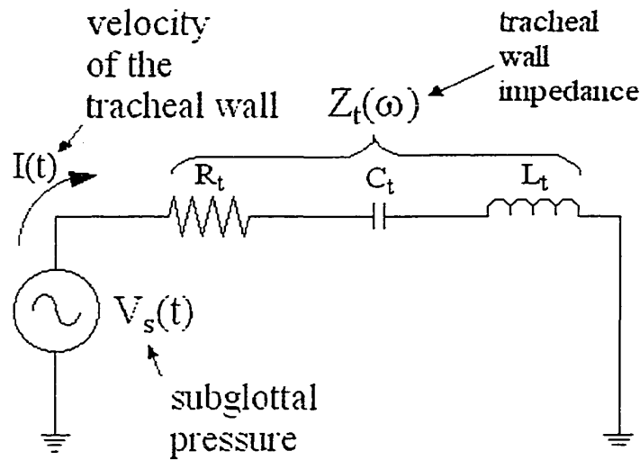
Figure 4.2. Electrical circuit model of the tracheal wall.
