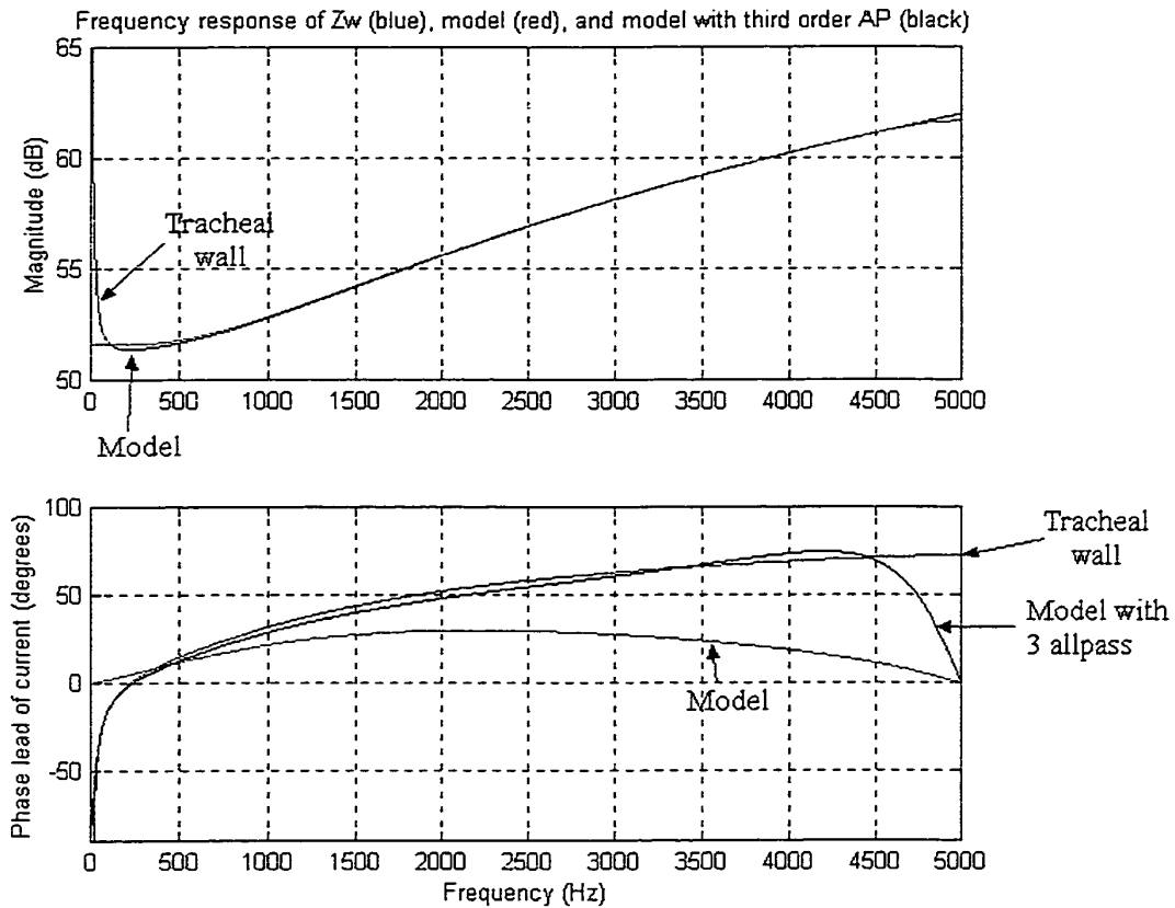
Figure 4.6. Tracheal wall impedance modeled digitally.
