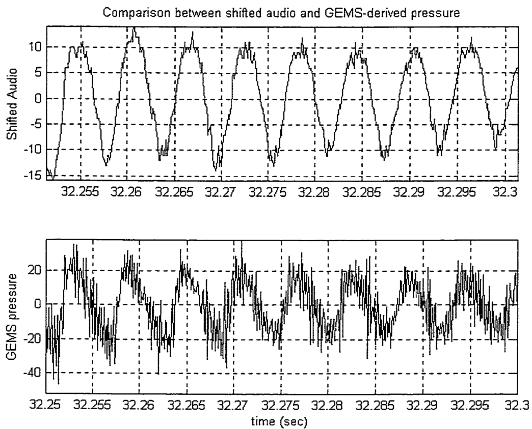
Figure 4.9. The breathy audio and the GEMS-derived pressure from Figure 3.14.
