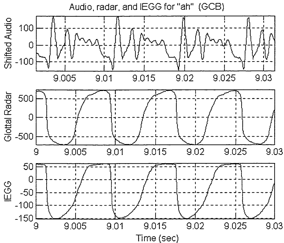
Figure 3.13. Audio, GEMS, and inverted EGG (IEGG) for /a/.
