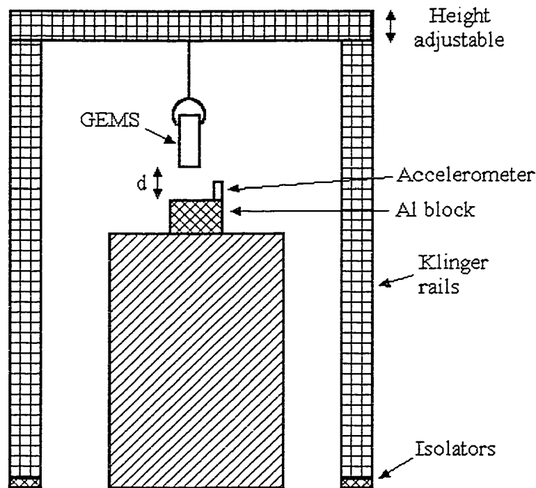
Figure 2.12. Shaker experimental setup.
