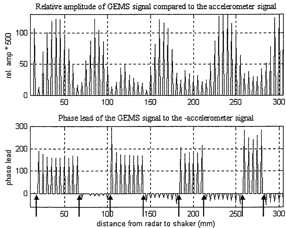
Figure 2.13. Relative amplitude (GEMS/accel) and phase lead of the GEMS vs. distance from the GEMS to the shaker block. The arrows denote points where the GEMS changed phase with respect to the inverted accelerometer signal.
