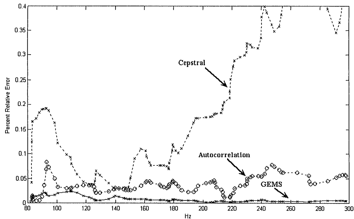
Figure C.6. Relative error vs. actual pitch for each pitch algorithm. A three second long synthetic signal with multiple harmonics was used. Cepstral (-x), autocorrelation (-o), and GEMS (x).
