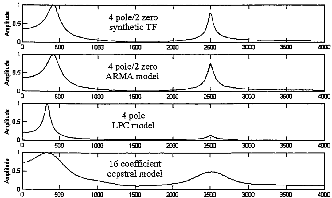
Figure 2.28. Comparison of a synthetic transfer function with 4 poles and two zeros (top) to three models: 4 pole/2 zero ARMA, 4 pole LPC, and 16 coefficient cepstral.
