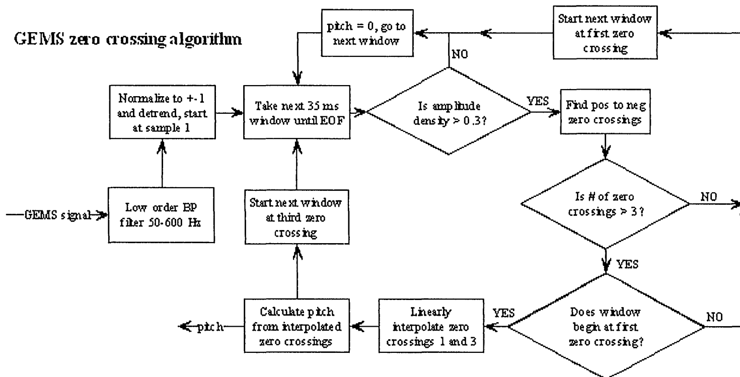
Figure C.4. Block diagram of the GEMS zero-crossing algorithm.
