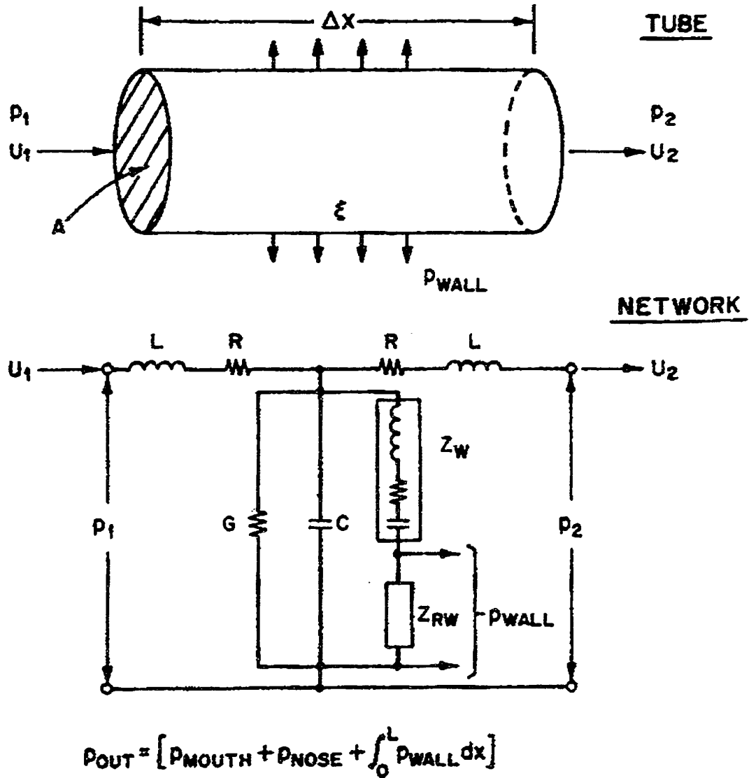
Figure 2.26. Equivalent circuit for plane acoustic wave propagation in an incremental yielding tube (from Ishizaka, French, and Flanagan (1975)).
