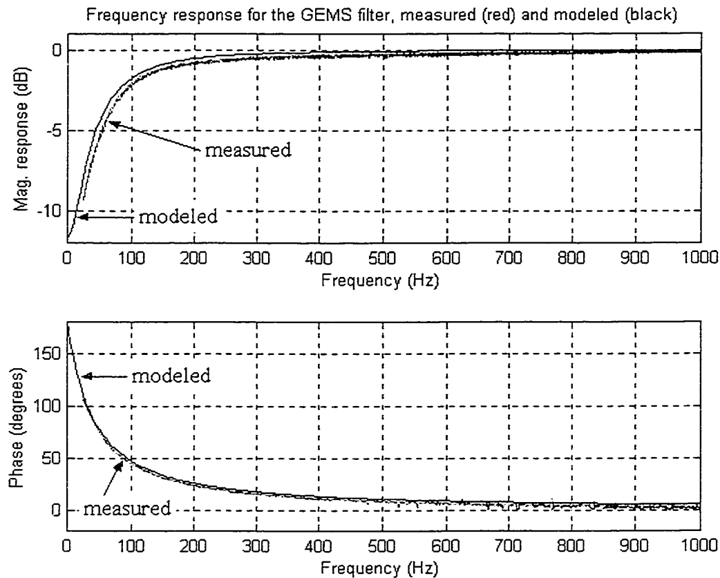
Figure 2.8. Measured GEMS filter response (red) and model response (black)
