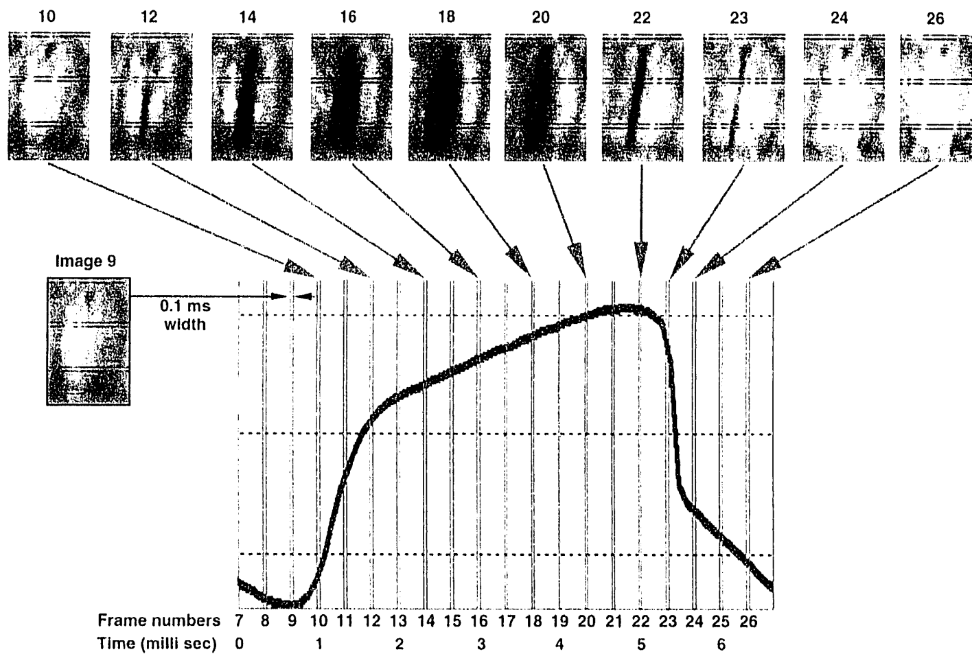
Figure 3.8. One cycle of a GEMS signal with some of the corresponding video frames. The vertical bars superimposed on the GEMS signal denote the exposure time. The GEMS signal has not been inverse filtered. The horizontal bars on the video frames are caused by a camera defect.
