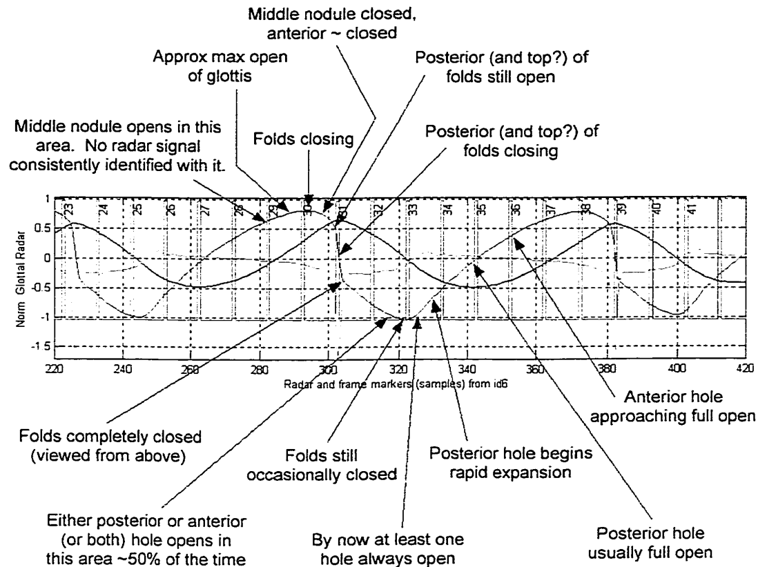
Figure 3.9. Plot of inverse filtered GEMS (blue), first derivative of GEMS (green), and integral of GEMS (black) along with the frame markers (red) for the abnormal physiology subject. The width of the frame markers denotes the exposure time of the frame. Observations for the dataset are included. The time scale is in samples, at 10000 samples/second.
