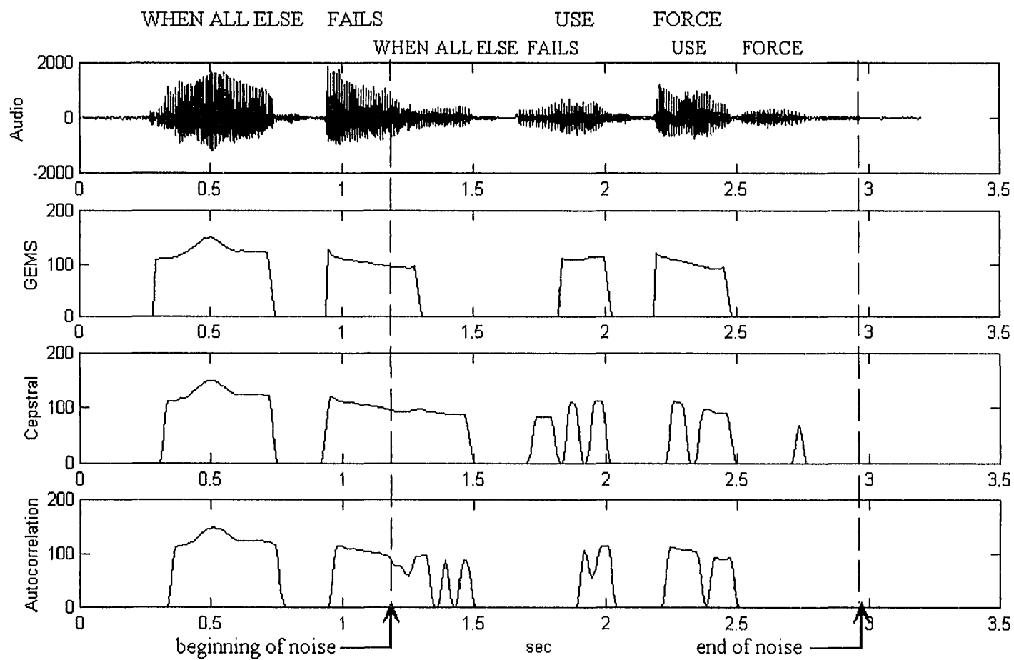
Figure C.8. Noisy (includes a second male speaker) audio signal ("When all else fails, use force") with pitch contours for GEMS, cepstral, and autocorrelation methods. Again the GEMS signal is unaffected.
