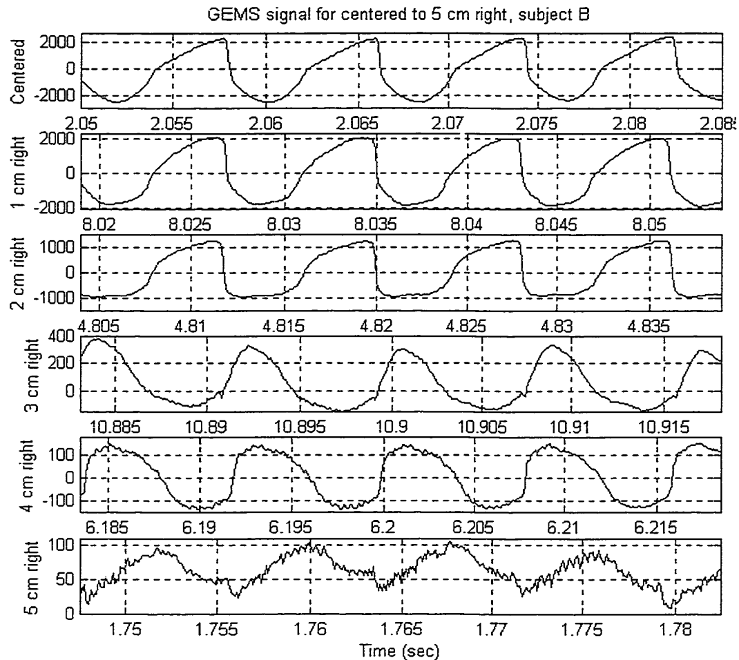
Figure 3.16. Data from position experiments when GEMS is moved from the center of the trachea (the laryngeal prominence) to 5 cm to the right of the prominence. Note the phase change at 3 cm and again at 5 cm.
