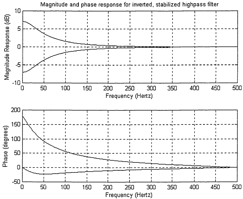
Figure A.4. The inverted, stable filter H_s(z) . The magnitude is perfectly inverted but the phase is not.
