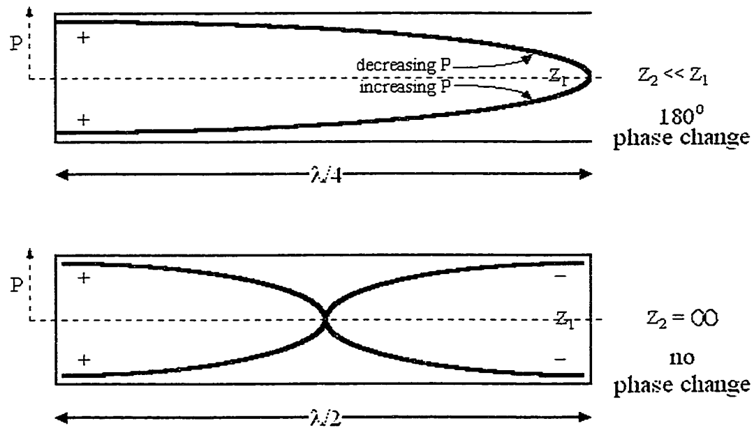
Figure 2.19. Standing pressure waves for the lowest resonances in an open-ended tube (top) and close-ended tube (bottom)
