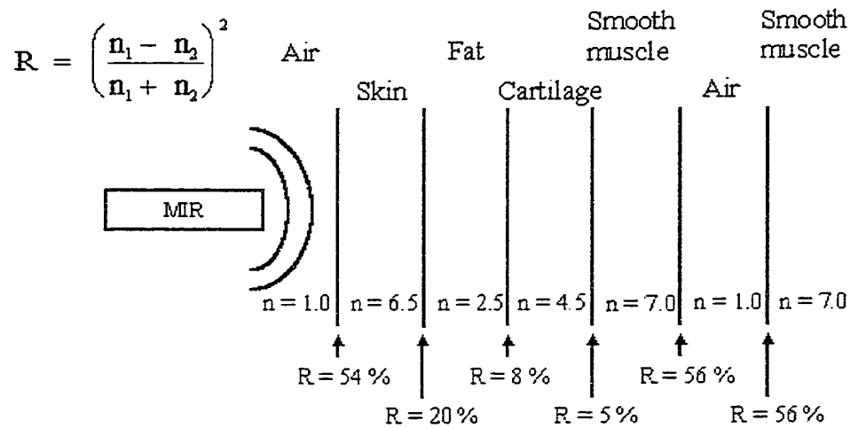
Figure 3.2. Simple planar calculation of the neck tissue layers' reflectivity, neglecting geometrical factors, multiple reflections, and conductivity.
