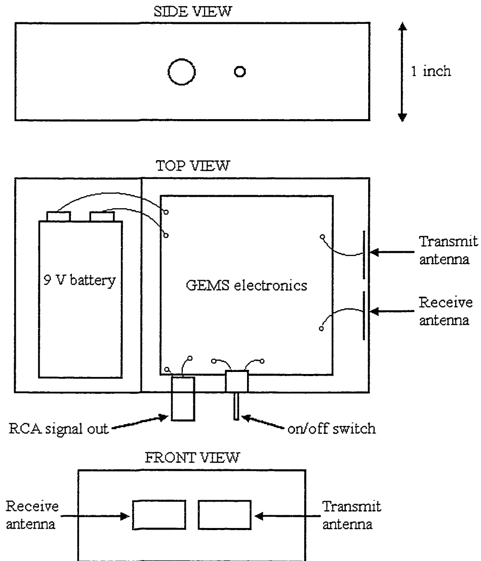
Figure 2.4. Overview of the GEMS's physical configuration.
