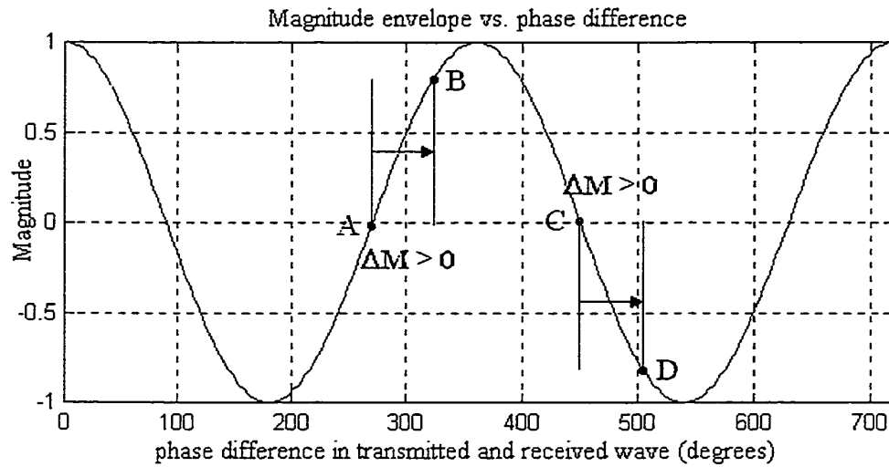
Figure 2.2. Theoretical magnitude response vs. phase difference \phi in the transmitted and reflected waves for a homodyne system. The same change in position results in two different values for the change in magnitude depending on the phase difference between the transmitted and reflected waves (or distance to the reflecting interface).
