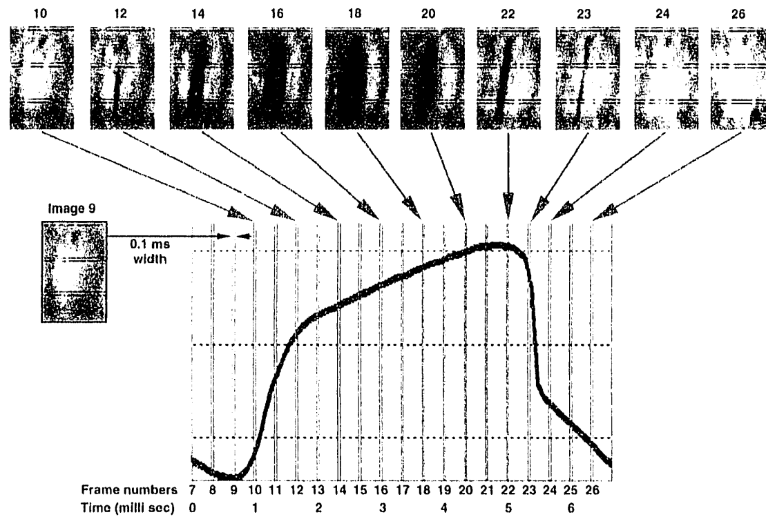
Figure B.5. GEMS signal overlaid with "ext sync" data. The exposure time is much smaller than the frame rate period and this results in sharp images.
