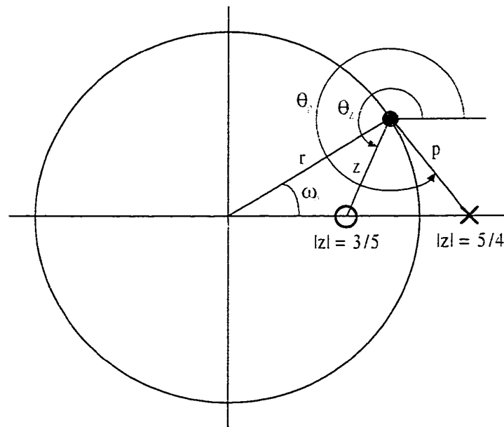
Figure A.2. An unstable filter in the z plane, and the method used to calculate the phase ( \theta_p and \theta_z ) and magnitude ( z and p ) contribution from each pole and zero.
