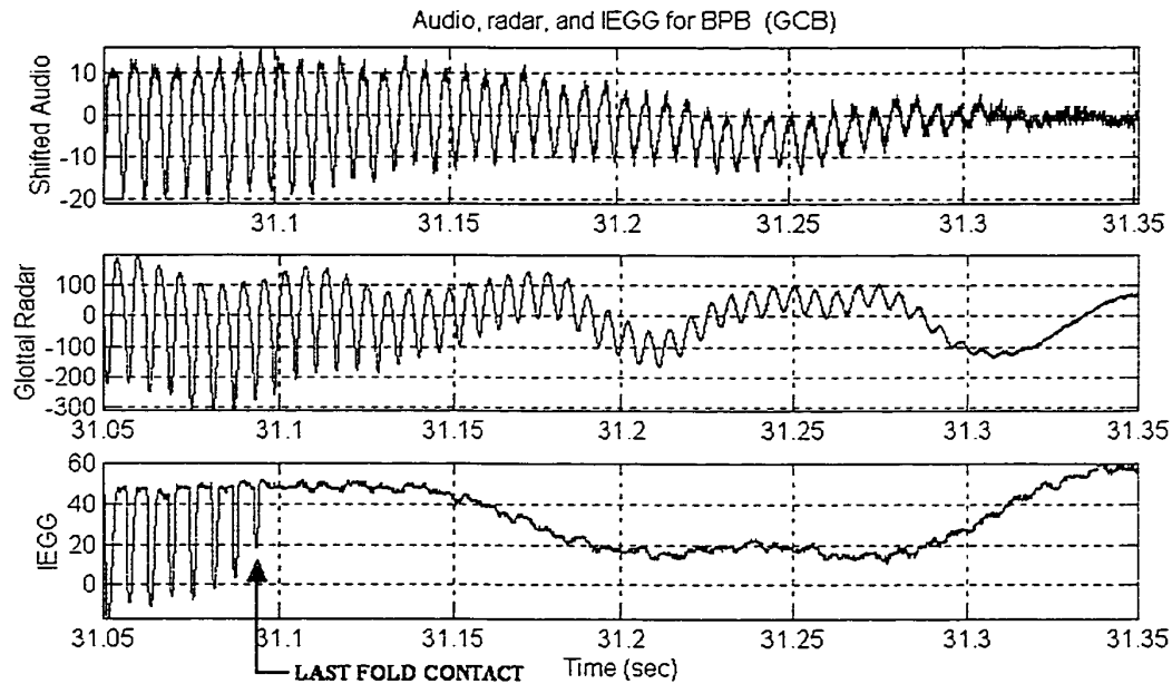
Figure 3.14. Plot of audio, GEMS, and IEGG for breathy cessation of speech. Note the total lack of EGG signal as contact is lost, and also the similarity of the audio and GEMS near the end of the speech.
