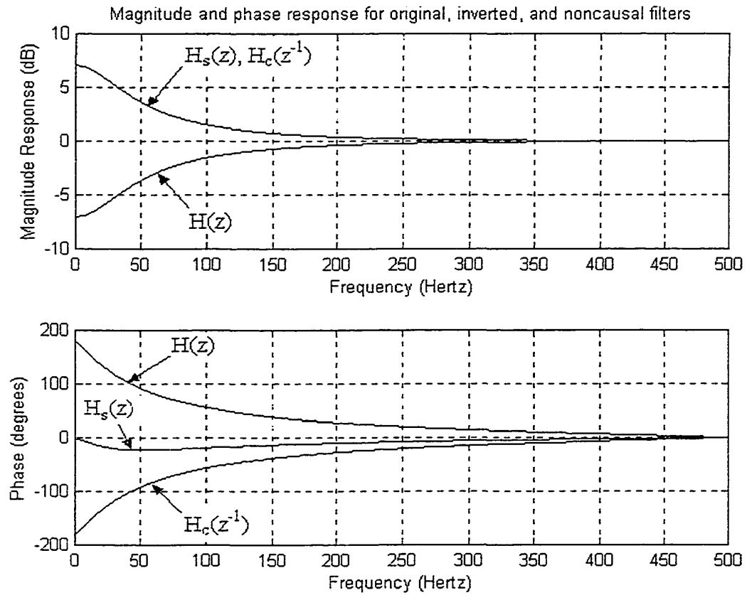
Figure A.7. The frequency response for the original filter H(z) , the stable inverted filter H_s(z) , and the noncausal filter H_c(z^{-1}) .
