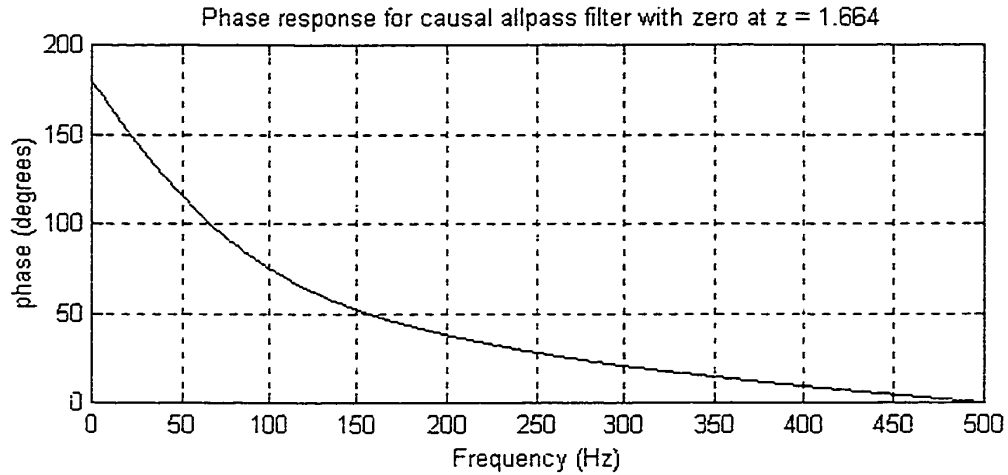
Figure A.6. Phase response for causal allpass filter designed to have a phase shift of 75 degrees at 100 Hz.
