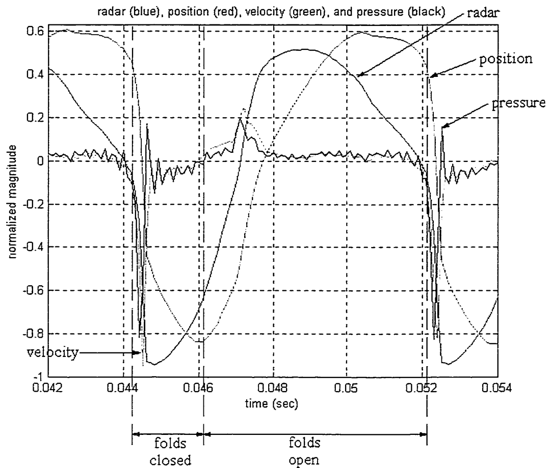
Figure 4.7. GEMS, position, velocity, and pressure for subject GB.
