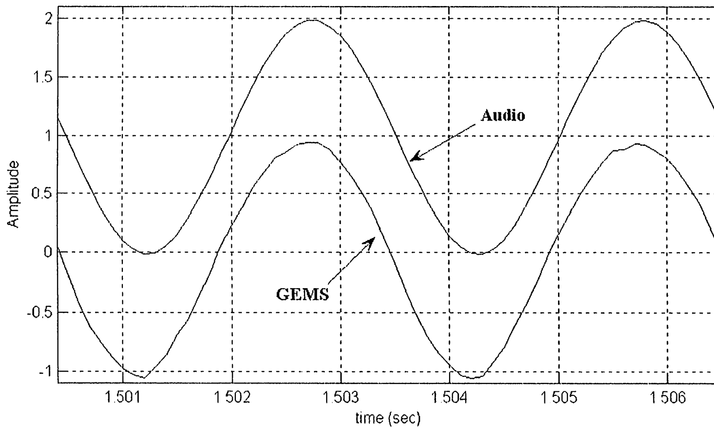
Figure C.5. Normalized signals from a tuning fork. The audio (upper) is offset in the y direction to facilitate comparison to the GEMS signal (lower).
