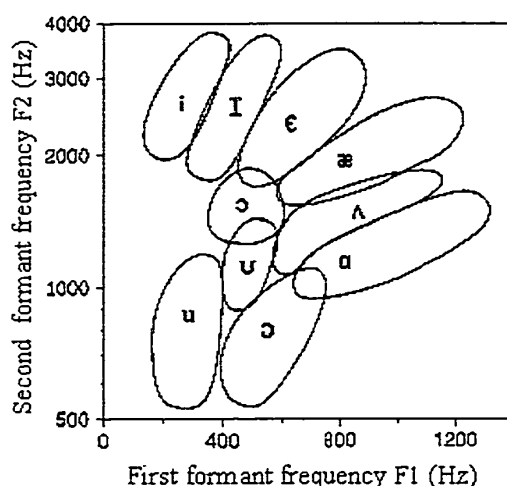
Figure 2.21. Vowel chart showing regions of F_1 and F_2 for 10 English vowels (from Titze, Principles of Voice Production , 1994. All rights reserved. Reprinted by permission of Allyn & Bacon).
