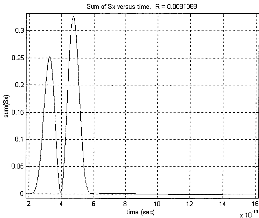
Figure 3.7. Energy vs. time for the fully open folds experiment. Note the almost total lack of (negative) reflected energy. R = 0.8\% .
