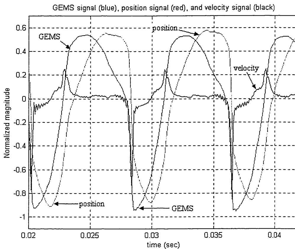
Figure 2.11. Plot of GEMS signal (blue), inverse filtered GEMS (position, red), and the derivative of the position (velocity, black) for a normal chest phonation.
