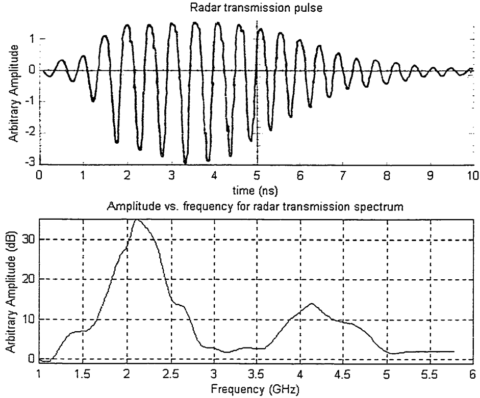
Figure 2.5. Plots of the GEMS pulse and frequency spectrum.
