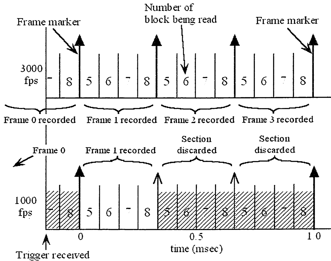
Figure B.6. How to determine where the exposure occurs when the intensifier is not available and the "frame marker" is used. In this example, 1/3 of the screen is used and an exposure time of 1/3000 of a second is selected. The top plot depicts operation at 3000 fps and the bottom at 1000 fps.
