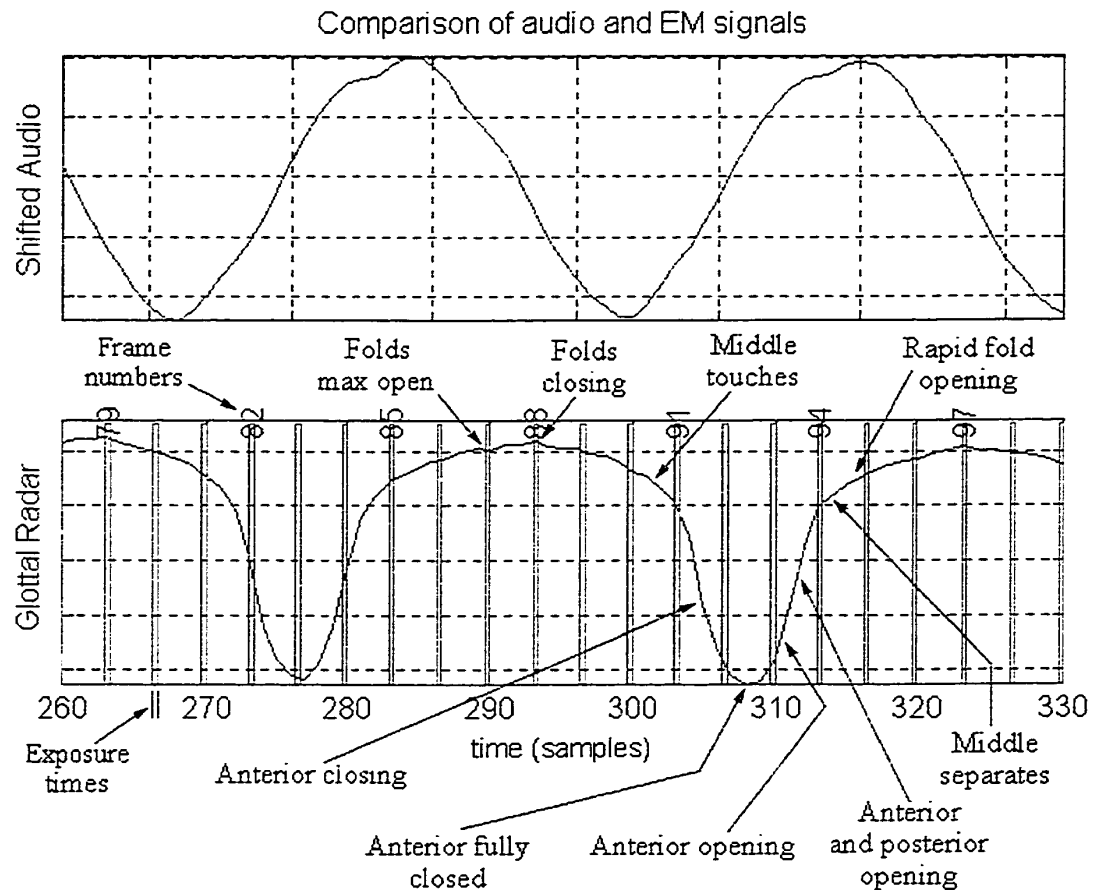
Figure 3.12. Summary of observations for the falsetto portion of the normal physiology. The time scale is in samples, at 10000 samples/second.
