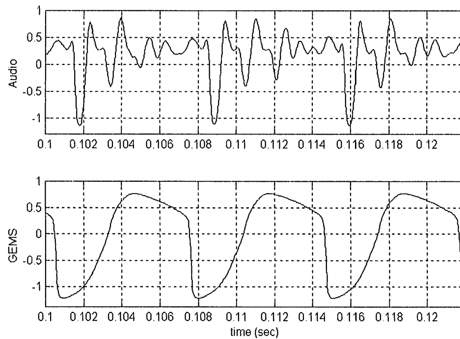
Figure C.2. Audio and GEMS signals from 29 year old male native English speaker, voicing /a/ ("ah")
