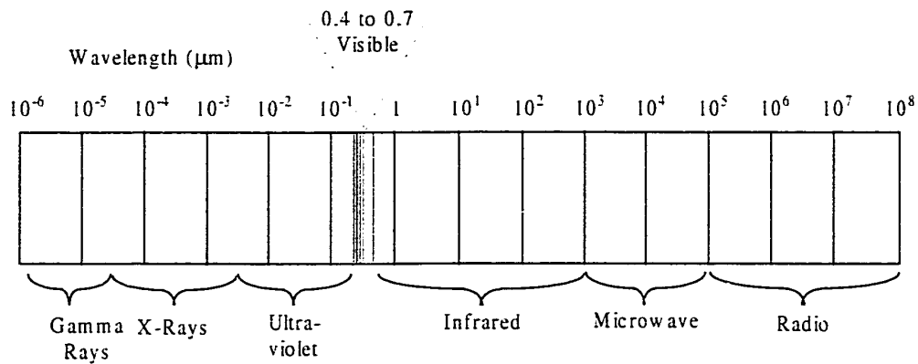
Figure 2.1. Classification of the spectrum based on wavelength
