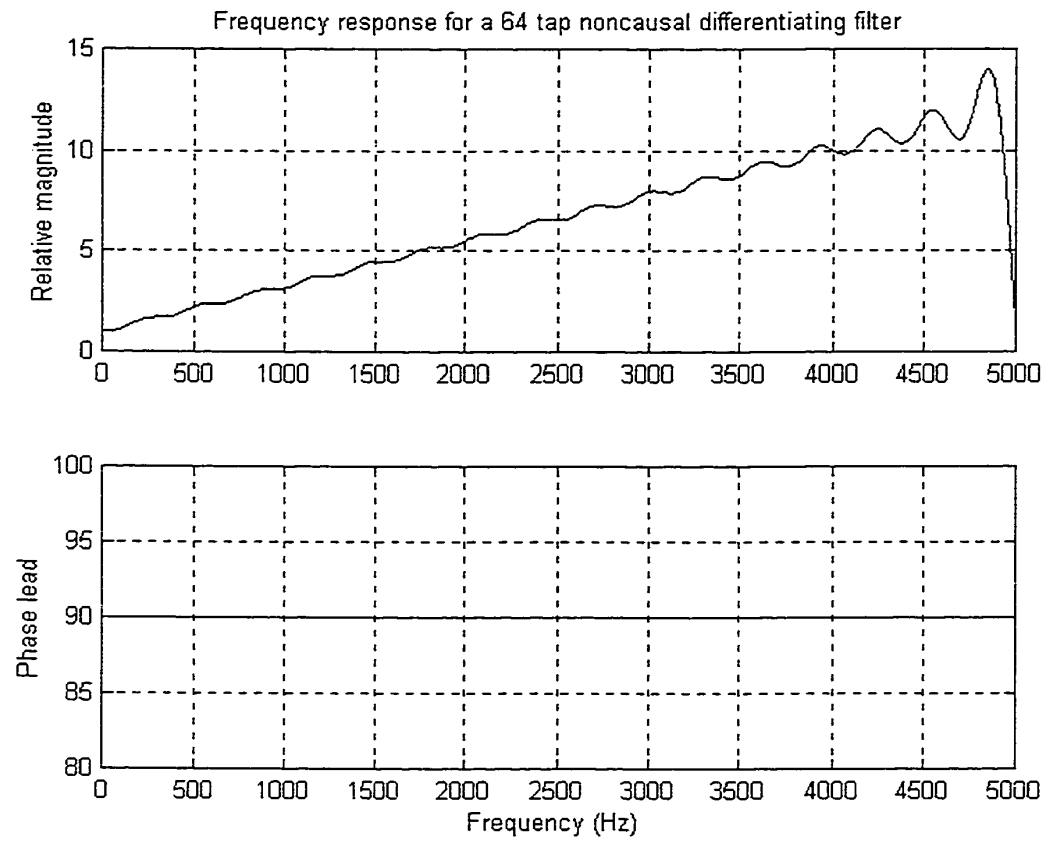
Figure 2.10. Magnitude and phase response for a 64 tap FIR noncausal differentiator.
