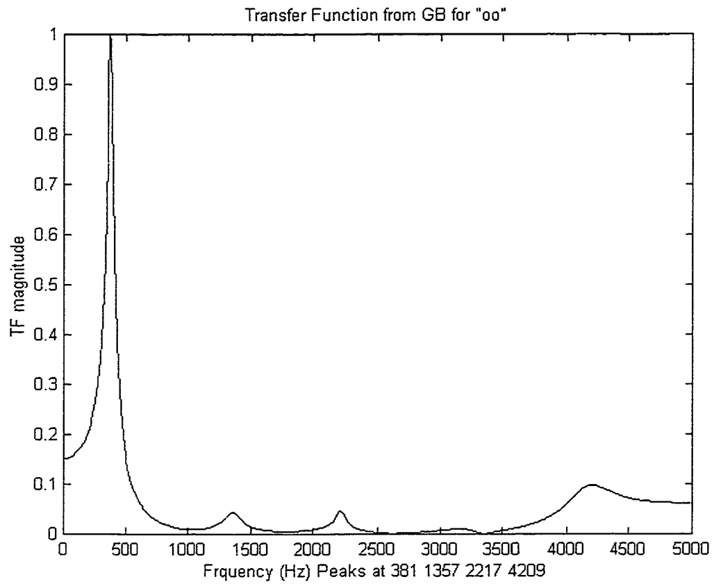
Figure 4.12. Calculated transfer function for /u/, subject GB. The first two formant locations are at 381 and 1357 Hz, normal locations are 400-600 and 900-1400.
