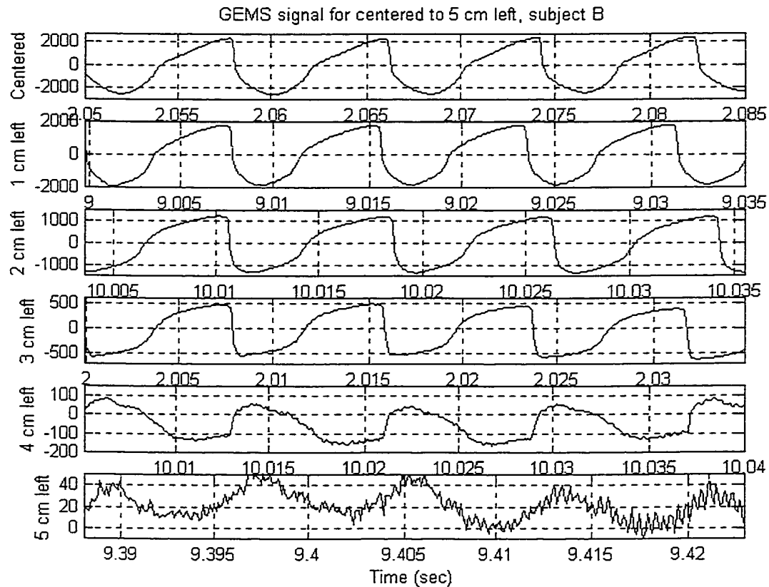
Figure 3.15. Data from position experiments when GEMS is moved from the center of the trachea (the laryngeal prominence) to 5 cm to the left of the prominence. Note the phase change at 4 cm.
