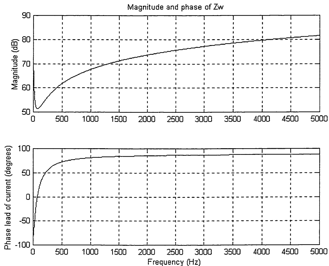
Figure 4.3. Magnitude and phase lead of the impedance Z_w of the lumped-element circuit model of the vocal tract.
