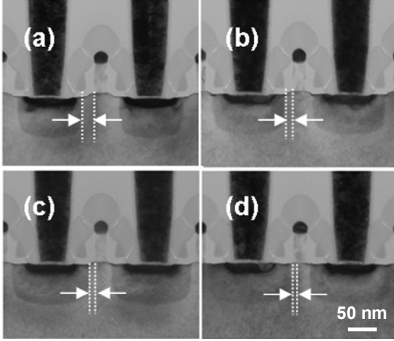
Figure 3. Cross-sectional TEM pictures of MOSFETs with different eSiGe proximity which is controlled by dummy spacer thickness.
