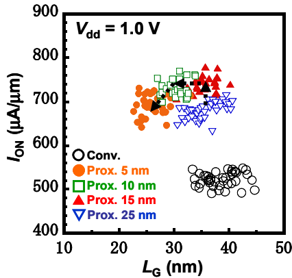
Figure 4. I_{ON} - L_G characteristics of each eSiGe proximity device
