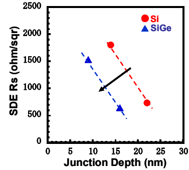
Figure 10. X_j -SDE R_s relationships. Suppression of Boron diffusion and higher activation in SiGe region improves X_j - R_s relationships in eSiGe devices.
