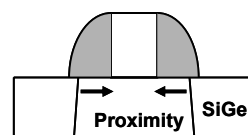
Figure 1. eSiGe proximity is key for mobility enhancement and SDE resistance reduction.
