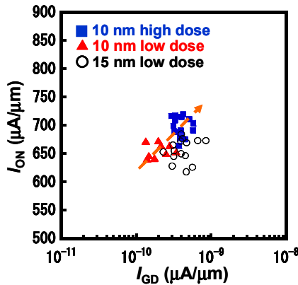
Figure 12. I_{ON} - I_{GD} characteristics. 10 nm eSiGe proximity device with higher SDE implantation dosage exhibits improved drive current at the same I_{GD} .
