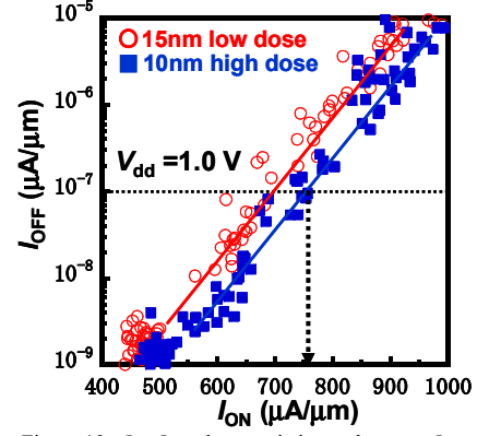
Figure 13. I_{ON} - I_{OFF} characteristics at the same I_{GD} .
