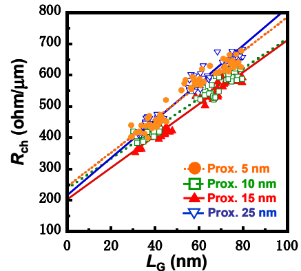
Figure 6. R_{ch} - L_G characteristics of each eSiGe proximity device
