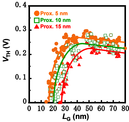
Figure 7. V_{TH} roll-off characteristics of each eSiGe proximity device.
