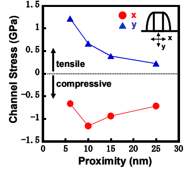
Figure 5. Channel stress vs eSiGe proximity. Channel stress enhancement is observed with reduction of eSiGe proximity.
