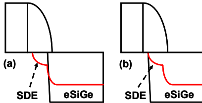
Figure 8. Schematic of correlation between eSiGe and SDE positions. Here, eSiGe proximity is (a) 15 nm (b) 5, 10 nm.
