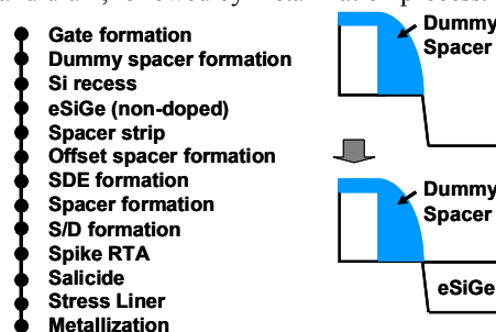
Figure 2. Process sequence of pMOSFET
