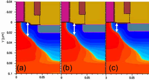
Figure 11. Boron profiles for each device by TCAD simulation. eSiGe Proximity is (a) 15 nm (b) 10 nm (c) 5 nm
