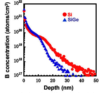
Figure 9. SIMS depth profiles of boron in Si and SiGe regions.
