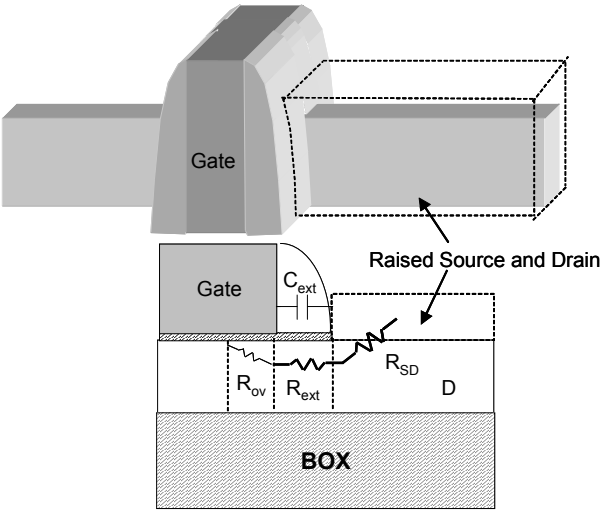
Fig. 2.33. The raised source and drain structure reduces the R_{SD} but increases C_{ext} .
