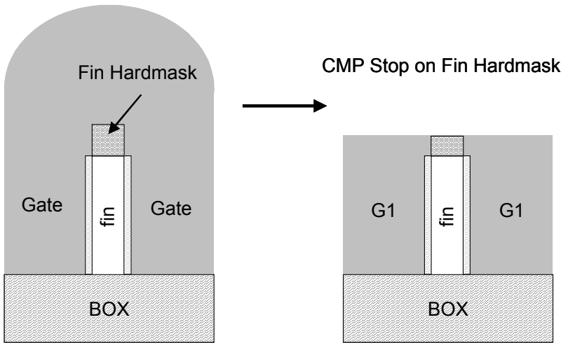
Fig. 2.29: Fabrication of a 4T-MuGFET: The unwanted gate electrode material is removed by Chemical Mechanical Polishing (CMP). The fin hardmask serves as CMP etch stop.
