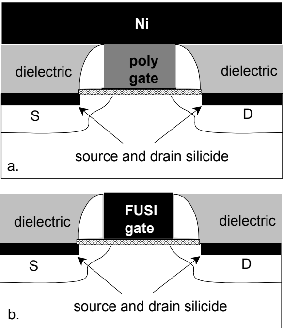
Fig. 2.22. Planar MOSFET Fully Silicided (FUSI) metal gate fabrication concept.
