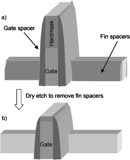
Fig. 2.34. Parasitic fin spacers are formed at the same time as gate spacer. The fin spacer must be removed prior to RSD growth process.
