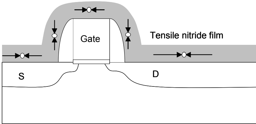
Fig. 2.39. A tensile stressor tends to shrink. The stressor on the source and drain pulls apart the ends of the channel and produce a tensile strain \sigma_{xx} in the silicon. The stressor on top of the gate squeezes the gate and produces a compressive stress \sigma_{zz} .
