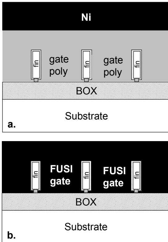
Fig. 2.23. Multi-gate FUSI metal gate formation, a) after metal deposition and b) after silicide formation. Fin topography creates differential gate poly thickness between the fin top and fin bottom. The silicide formation front first reaches the fin top, and must continue to the bottom of the fin. The silicide phase uniformity throughout the gate thickness must be controlled and metal diffusion through the gate dielectric through the extended silicidation process must be limited.
