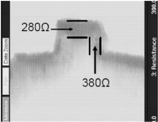
Fig. 2.32. SSRM profile of a PLAD implanted fin. The doping uniformity of the fin top and fin sidewall is not perfect, but it is better than what can be achieved by 45 degree tilt implant.[100] Copyright© 2006 IEEE.
