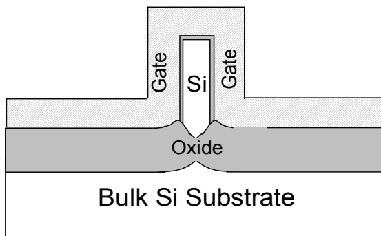
Fig. 2.1. DELTA MOSFET [1-2]. The oxide under the Si fin was formed through LOCOS oxidation while the Si fin was protected by the nitride hard mask and a nitride spacer prior to the oxidation process.
