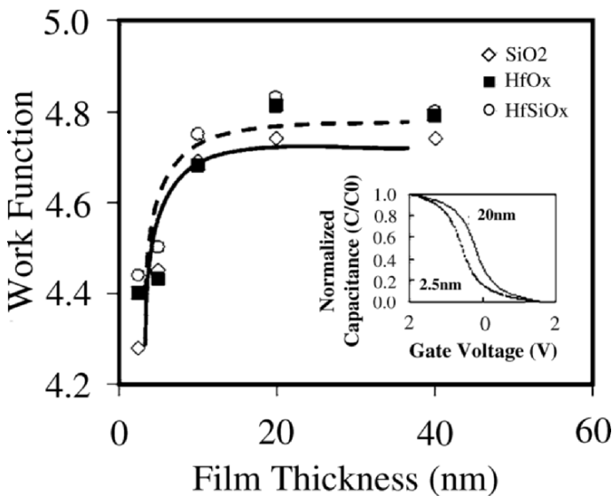
Fig. 2.24. TiSiN effective workfunction as a function of the TiSiN film thickness and gate dielectric materials. REPRINTED WITH PERMISSION FROM [17]. COPYRIGHT 2006 AMERICAN INSTITUTE OF PHYSICS.
