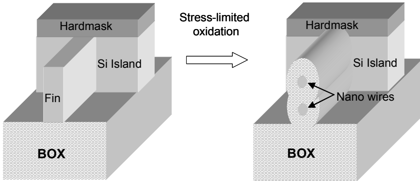
Fig. 2.16: Twin Si nanowires formed through stress-limited oxidation. A hard mask is needed to keep the Si island region from oxidizing. The presence of Si island at the end of the wires is needed to anchor the wires.
