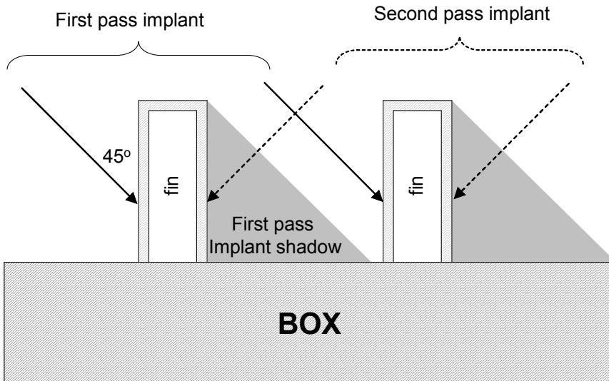
Fig. 2.30. Tilted S/D implant.
