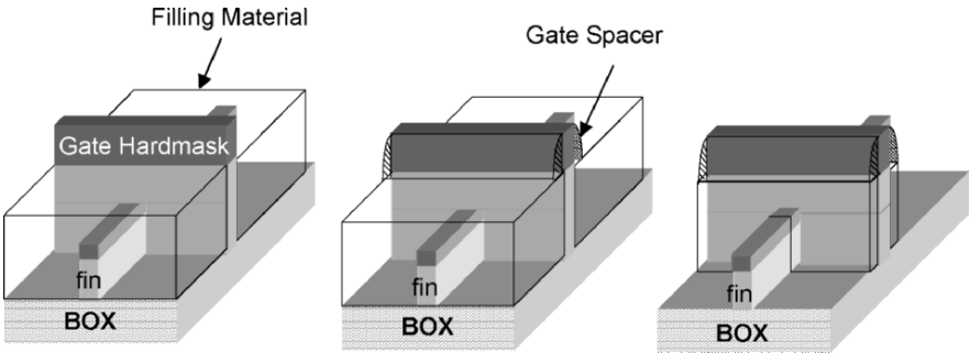
Fig. 2.36. Integration scheme to form gate spacer without parasitic fin spacer.
