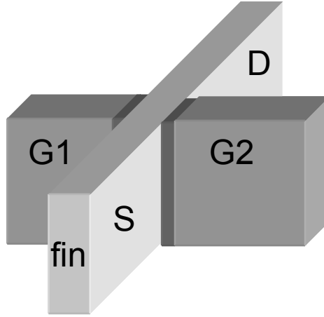
Fig. 2.27. 4T-MuGFET, Gate 1 (G1) and Gate 2 (G2) are electrically isolated from one another. This configuration allows for the independent biasing of G1 and G2.
