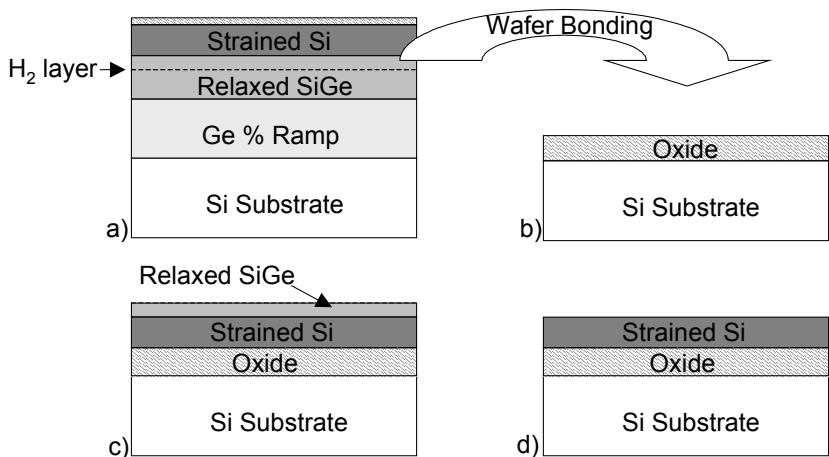
Fig. 2.42. Illustration of the fabrication sequence of a sSOI wafer. a) Starting bulk sSi wafer is implanted with H_2 . b) The sSi wafer is bonded to a host wafer, and c) an ion-cut process is used for layer transfer. d) The remaining SiGe is selectively etched away from the strained Silicon on Insulator material.
