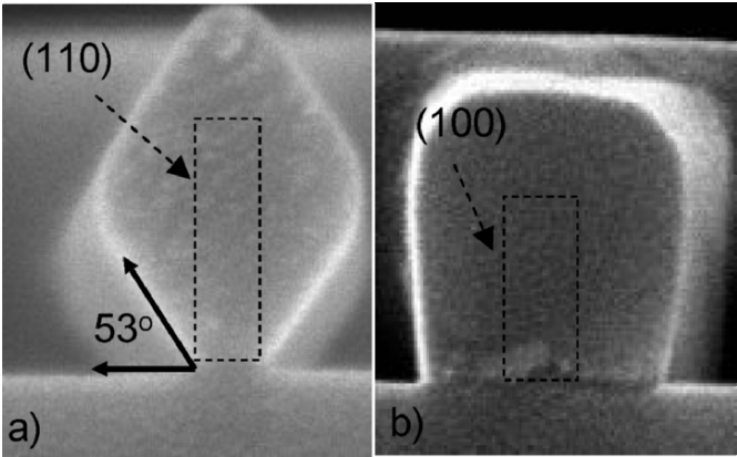
Fig. 2.37. Cross sectional SEM images on fins after epitaxial growth. a) (110) side wall surface result in diamond-shaped fin; b) (100) sidewall surface result in square-shaped fin.
