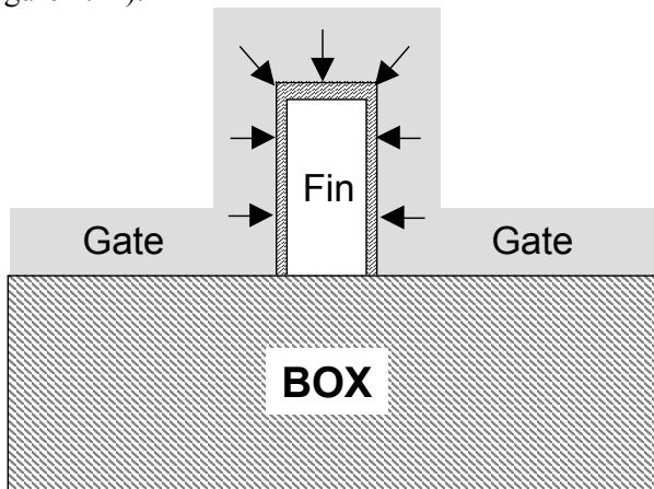
Fig. 2.41. Expansion of metal gate electrode during thermal processing exerts a compressive stress in the fin.
