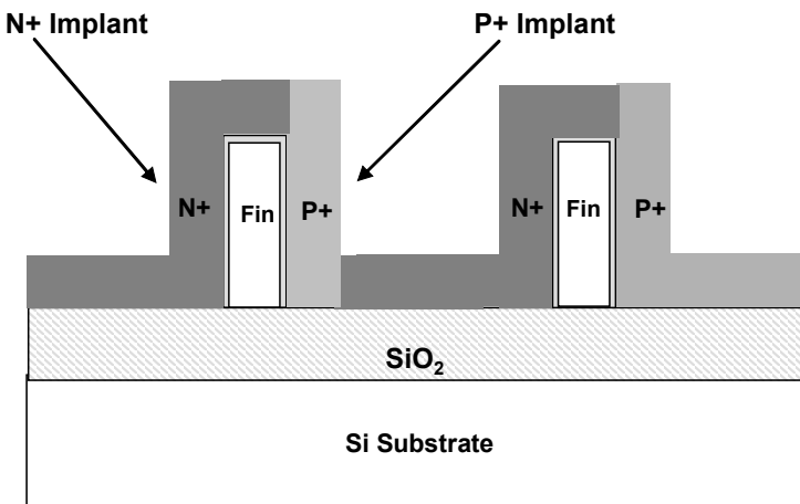
Fig. 2.21. \text{N}^+ and \text{P}^+ asymmetrical poly-gate formation. Large-tilt-angle gate implant is employed to dope the gates on one side of the fin \text{N}^+ , and the other side \text{P}^+ . The implant shadowing effect created by the tall fin helps to achieve this result.
