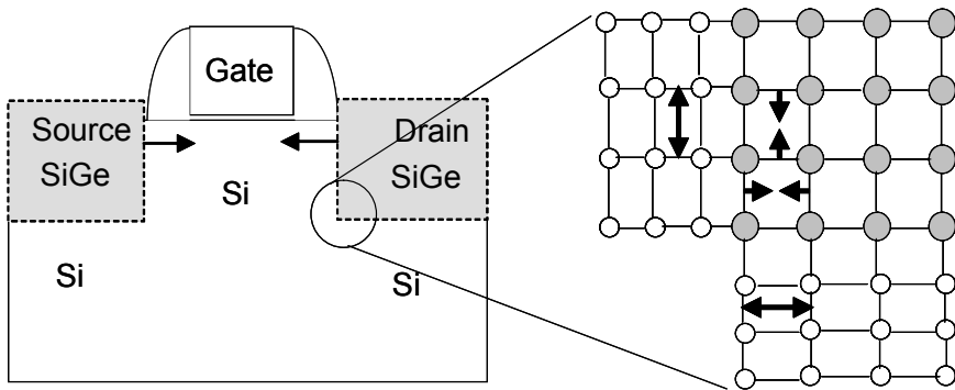
Fig. 2.40. The lattice mismatch between SiGe and Si results in channel compressive stress in the \sigma_{xx} direction and tensile stress in the \sigma_{yy} direction. \sigma_{xx} compressive stress improves hole mobility.
