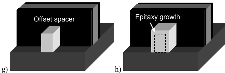
Fig. 2.2. General Fabrication Sequence of a Tri-gate MOSFET.
