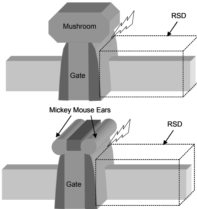
Fig. 2.35. If the polysilicon gates are NOT completely covered by protective dielectric, gate “mushroom” or “Mickey Mouse Ears” defects will occur. Both defects can cause short circuit between gate and source and drain.
