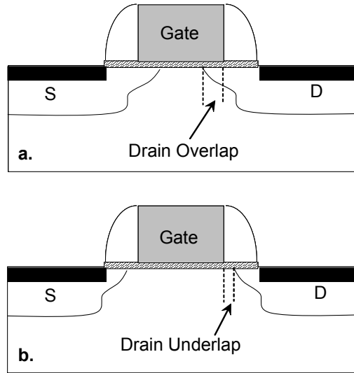
Fig. 2.26. a) Drain overlap MOSFET: GIDL occurs in the overlap region; b) Drain underlap MOSFET: Drain is moved away from the gate. As a result, the electrical field and the GIDL current are reduced.
