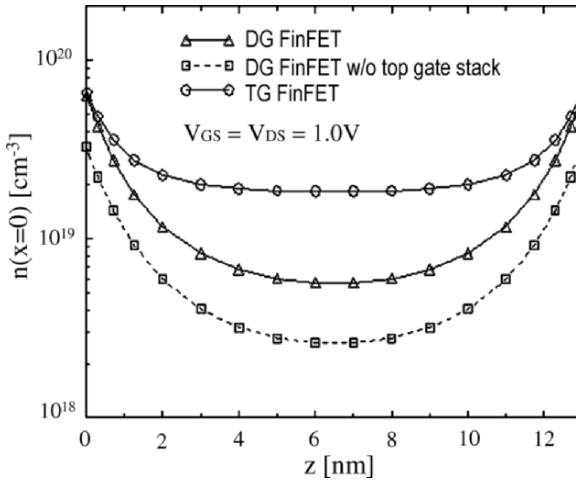
Fig. 2.6. Davinci prediction of on-state electron density along the top fin surface at the center of the channel ( x=1/2 L_{eff} ). DG stands for double gate. TG stands for tri-gate. Due to bulk inversion, the electron density on the top fin surface for DG FinFET is comparable to that in the TG device [26]. Copyright© 2005 IEEE.
