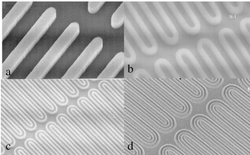
Fig. 2.9. SEM pictures of three progressive spacer-defined fin formation processes. a) initial optical lithography of sacrificial pattern. b) after first spacer imaging; c) after second spacer imaging; and d) after third spacer imaging. The final pattern pitch is 6 times smaller than the optical lithography pitch. REPRINTED WITH PERMISSION FROM [33]. COPYRIGHT 2003 AMERICAN INSTITUTE OF PHYSICS.
