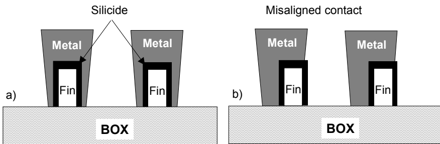
Fig. 2.44. Saddle contact: a) perfect contact to fin alignment; b) misaligned contact.
