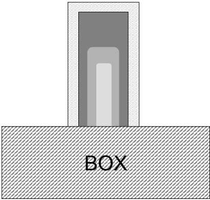
Fig. 2.31. Illustration of the impact of tilted implant on the doping profile in the fin. The darker color represents a higher doping concentration. Double implants on the top of the fin result in non-uniform doping concentration and resistance.
