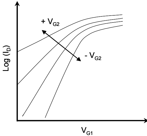
Fig. 2.28. 4T-MuGFET drain current as a function of G1 voltage ( V_{G1} ) and G2 voltage ( V_{G2} ). V_{G2} affects the I_D vs. V_{G1} curves.
