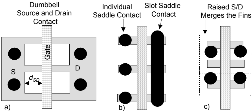
Fig. 2.43. Three contact options for MuGFETs: a) contact to the dumbbell source and drain; b) saddle contact to individual fin, or slot contact; c) contact to the merged-fin source and drain.
