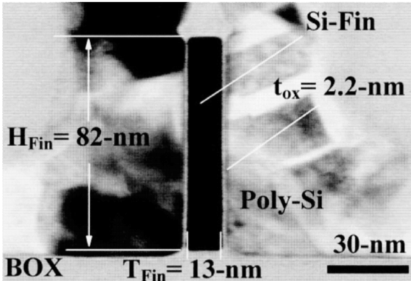
Fig. 2.13. Cross-sectional TEM of a (111)-surface sidewall fin. The smooth rectangular shaped fins were formed using surface-orientation dependent wet etch chemistry.[19] Copyright© 2003 IEEE.
