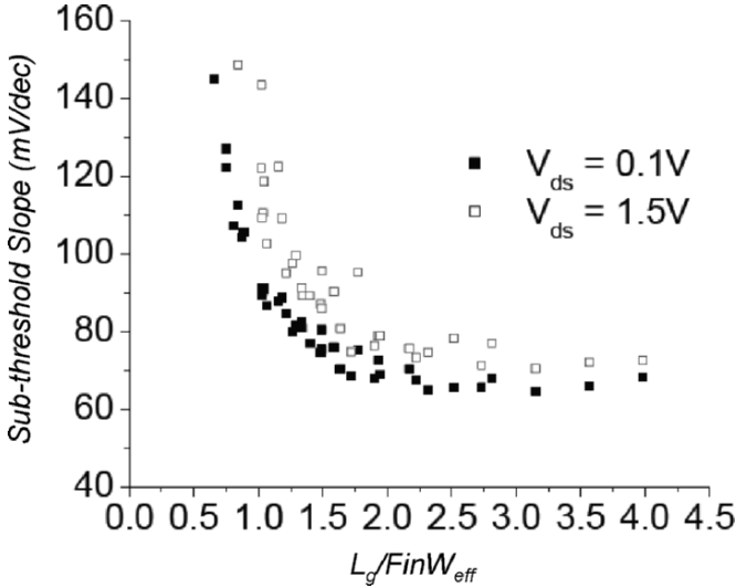
Fig. 2.4. Measured subthreshold swing vs. L_g/FinW_{eff} . Fin_{WIDTH} varies from 20nm to 90nm; L_g varies from 30nm to 120nm. The subthreshold slope is shown for both for V_d=0.1V and 1.5V.[22] Copyright© 2001 IEEE.
