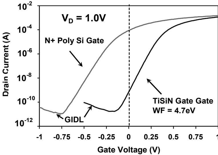
Fig. 2.25. GIDL current as a function of gate voltage and gate electrode workfunction. Using a higher gate effective workfunction shifts the I_d(V_g) curve to the right and increases the GIDL current at any given gate voltage.[67]
