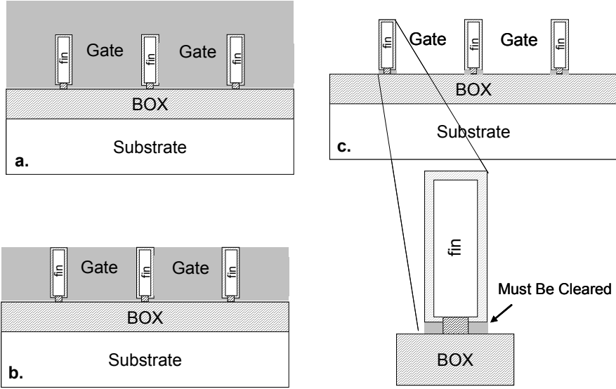
Fig. 2.19. The key aspects of the gate etch are the ability to etch the gate material between the fins without damaging the fin (a,b), the removal of the gate material in the undercut region between the fin and buried oxide (c).
