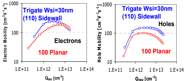
Fig. 4a Electron mobility comparison of a planar <100> vs. a Trigate device.
