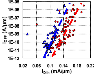
Fig. 8a I_{D,lin} versus I_{off} for SiGe raised with & without undercut etch.
