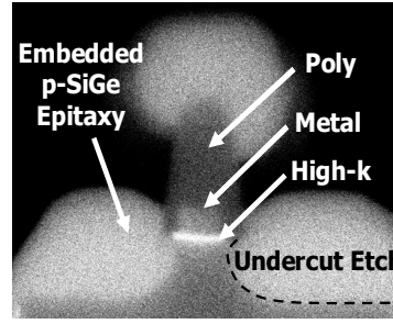
Fig. 7a X-dir. cross-section of PMOS Trigate with SiGe raised source/drain
