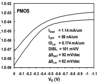
Fig. 10b I_D - V_G for PMOS Trigate device at V_{DS}=1.1 and 0.05V
