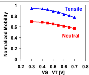
Fig. 6 Normalized electron mobility for tensile versus neutral strain.
