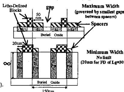
Figure 14. Period of Tri-Gate structures using spacer printing approach for both max. width and min. width dimensions to maintain full depletion
