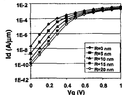
Figure 12. Simulation of the Id-Vg characteristics of the corner device, with different radii of curvature and Lg=30nm.
