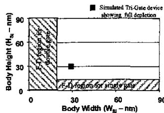
Figure 7. Regions of fully depleted and partially depleted behavior for single gate and double-gate @Lg=30nm. Tri-Gate body shows more relaxed body dimensions than either.
