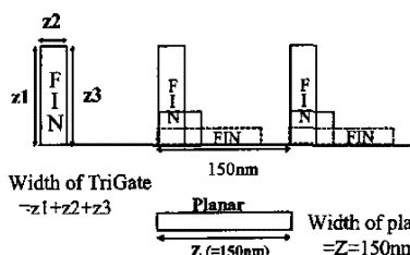
Figure 13. Measurement of drive current per unit width (period). Tri-gate: z1+z2+z3. Planar: Z. A variety of potential Tri-Gate dimensions is also shown, each of which would have different perimeter width per unit period
