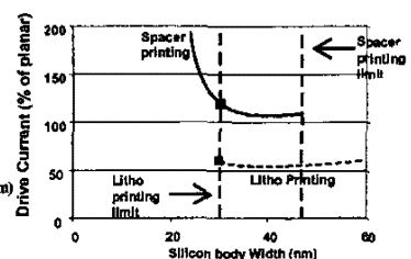
Figure 15. Drive current obtained for the various shapes of fully-depleted silicon fin for both litho printing and spacer printing. The silicon height is adjusted to maintain full depletion.
