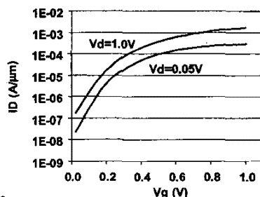
Figure 8. 3-D Simulation of a 30nm Tri-Gate transistor.
