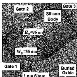
Figure 4. Cross-section of silicon body for the nMOS Tri-Gate Transistor of Figs 2 & 3.
