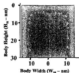
Figure 11. Simulation of electron density in the body at mid-point between source and drain, for Vd=1V, Vg=0.4.
