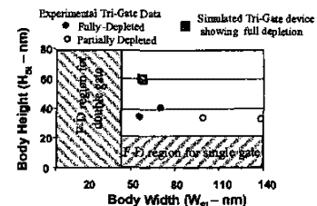
Figure 6. Regions of fully-depleted and partially-depleted behavior for Single gate and double-gate @Lg=60nm. Tri-Gate body shows more relaxed body dimensions than either.
