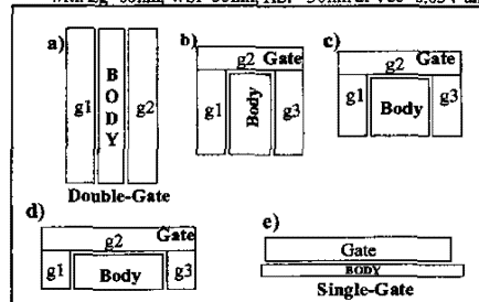
Figure 5. Schematic illustration of the types of fully-depleted transistor architectures. The Tri-Gate (b-d) offers flexibility in silicon body geometry.
