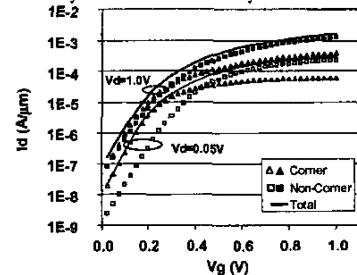
Figure 9. 3-D Simulation of Lg=30nm Tri-Gate device, showing current contributions of corner and non-corner regions.
