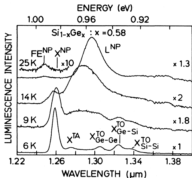
FIG. 3. Photoluminescence spectra of a bulk \text{Si}_{1-x}\text{Ge}_x ( x=0.58 ) sample at different temperatures.
