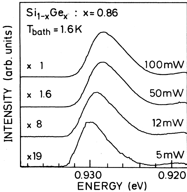
FIG. 5. Line shape of the X^{\text{NP}} transition for different laser powers. The \text{Si}_{1-x}\text{Ge}_x sample has a composition of x = 0.86 . The excited area of the sample is approximately 1 \text{ mm}^2 .
