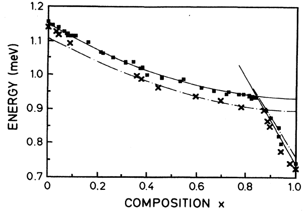
FIG. 9. Excitonic band gap (■) vs composition x for \text{Si}_{1-x}\text{Ge}_x alloys, as determined from low-temperature PL spectra. Literature data are included for comparison ( \times ) (Ref. 27). The dotted line corresponds to the analytical expression given in Ref. 33. The solid line gives our fit to the measured data.
