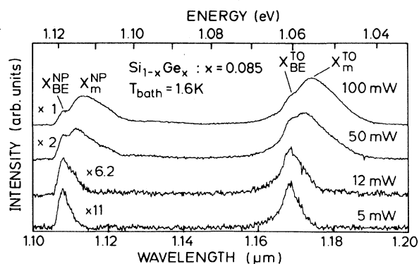
FIG. 4. Dependence of the PL spectra on laser power for sample \text{Si}_{1-x}\text{Ge}_x ( x=0.085 ). The excited area on the samples is approximately 1 \text{ mm}^2 .
