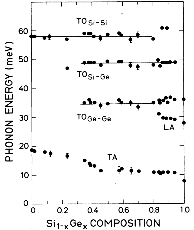
FIG. 8. Phonon energies for different compositions x derived from the energy separation between the NP lines and the phonon replica lines.
