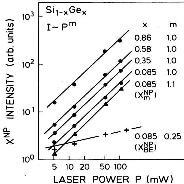
FIG. 6. Intensities of the X^{\text{NP}} transitions in different samples as a function of the laser power. For the sample with composition x = 0.085 the intensities of X_m^{\text{NP}} ( \blacktriangle ), X_{\text{BE}}^{\text{NP}} ( + ), and the total intensity X^{\text{NP}} ( \bullet ) are shown.
