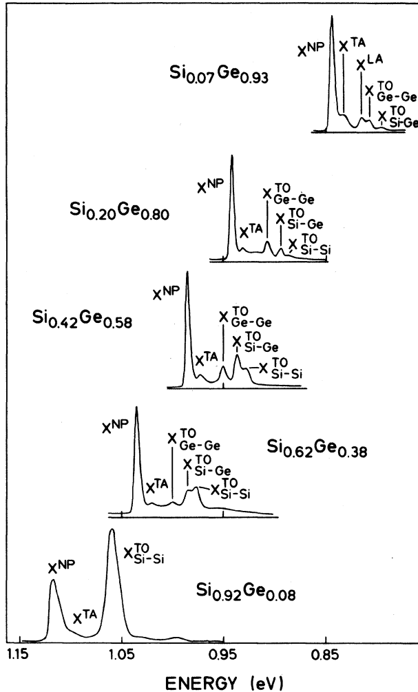
FIG. 1. Near-band-gap photoluminescence spectra for several bulk Si-Ge samples. The optical transitions are named X_j^i where j gives the type of transition (no-phonon or phonon participation) and i specifies the nature of the phonon.
