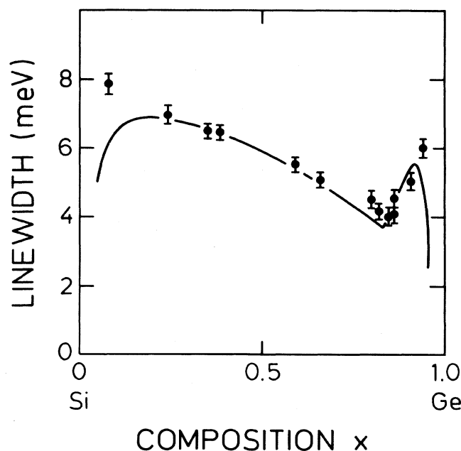
FIG. 10. Linewidth of the X_{BE}^{NP} transition vs composition. The solid line is the predicted linewidth using Eq. (4).
