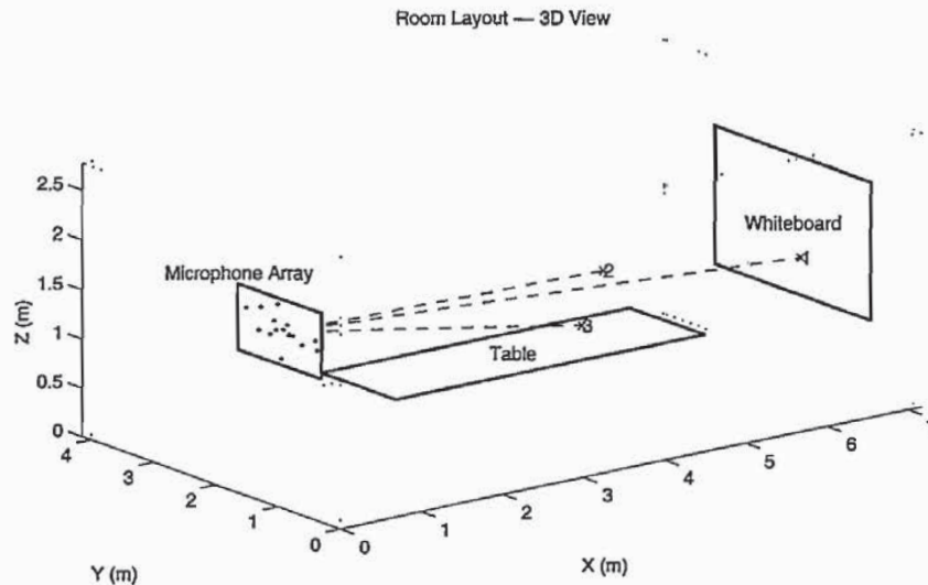
Fig. 8.2. Conference room layout.
