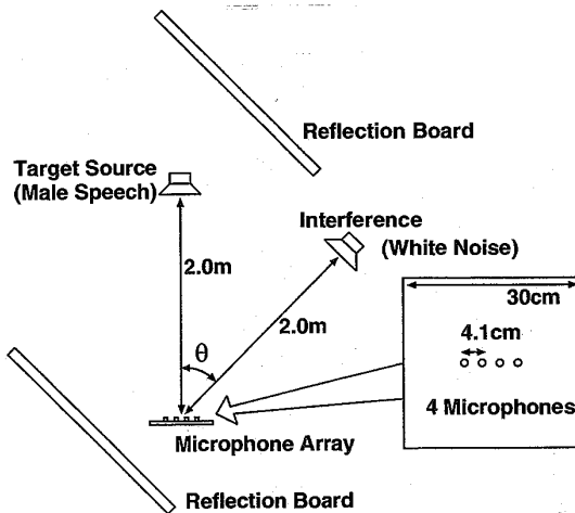
Fig. 5.13. Experimental set-up.
