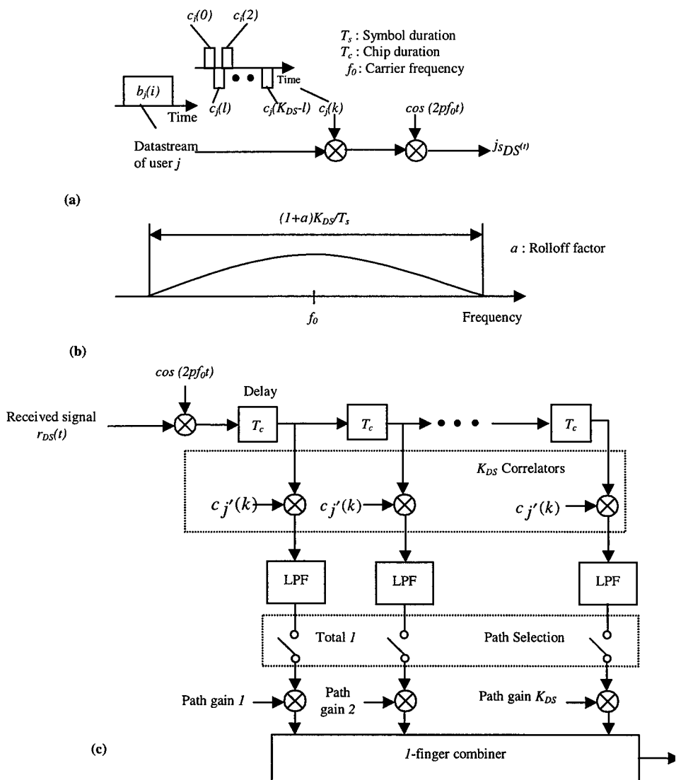
Figure 8.2 DS-SS system: (a) transmitter, (b) power spectrum of its transmitted signal, and (c) RAKE receiver.
