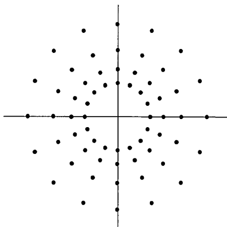
Figure 5.14 64-DAPSK constellation.
