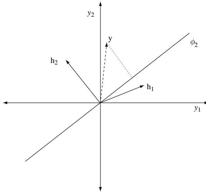
Figure 3.13 Demodulation of x_1 : the received vector y is projected onto the direction \phi_2 orthogonal to h_2 . The effective channel for x_1 is in deep fade whenever the projection of h_1 onto \phi_2 is small.
