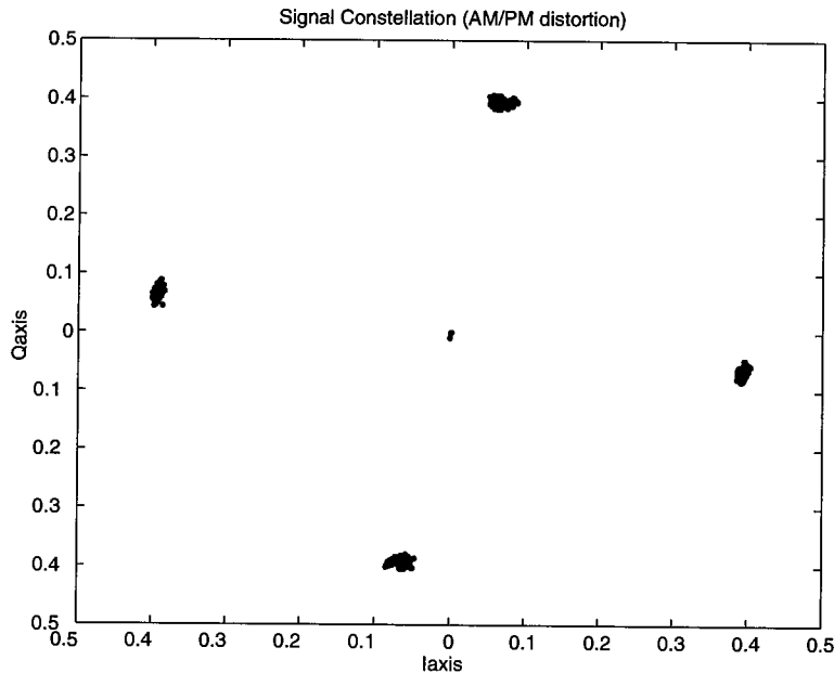
FIGURE 5.6 AM/PM distortions on a quaternary phase shifting keying signal.
