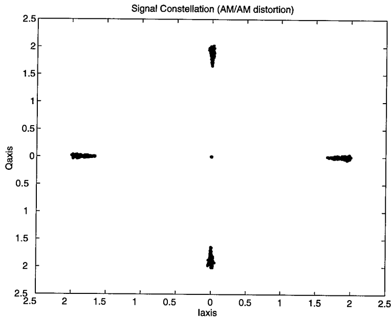
FIGURE 5.5 AM/AM distortion on a quaternary phase shifting keying signal.
