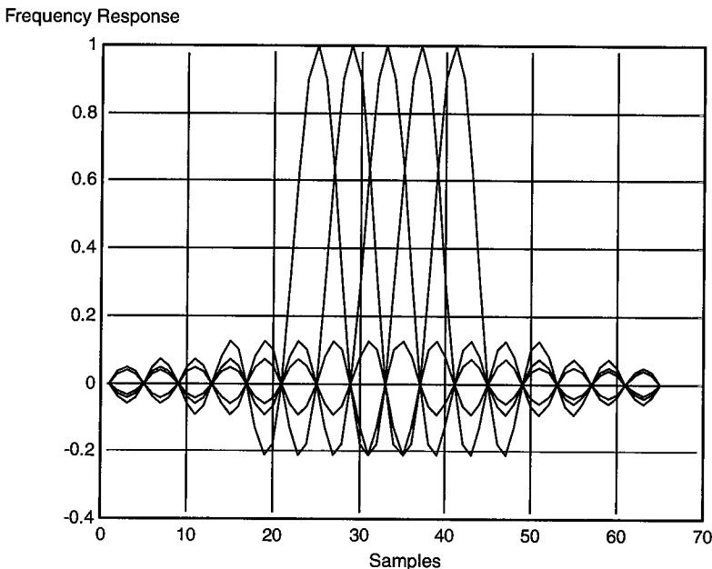
FIGURE 1.12 Overlapping orthogonal carriers.
