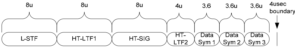
5 6 Figure n65 - Packet alignment example - GF packet with short GI
