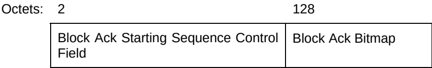
Figure n8 – Simple Block Ack Information field format
