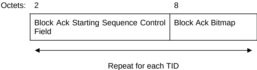
Figure n8 – MTID Block Ack Information field format
