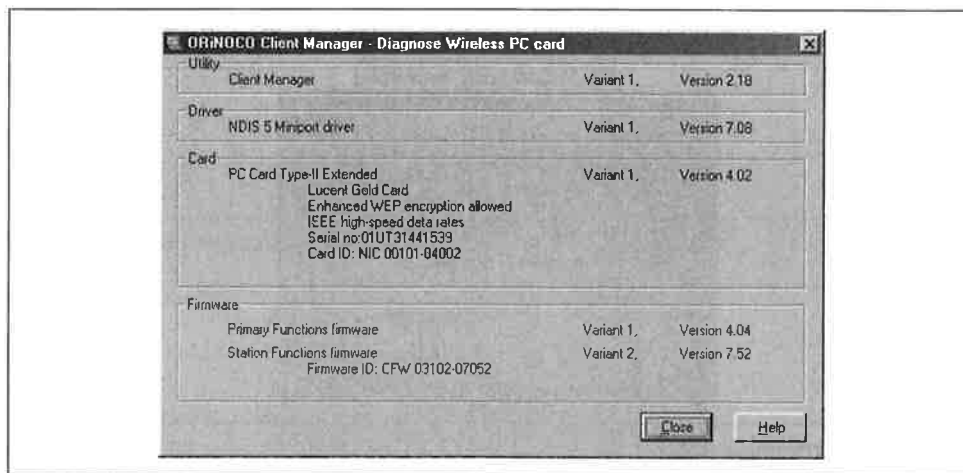
Figure 12-33. Version information
