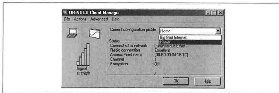
Figure 12-32. Changing profiles
