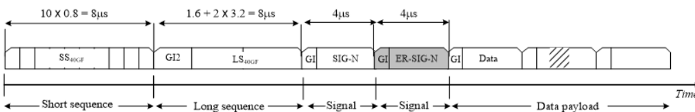
Figure 011 – MIMO-OFDM Training structure for N_{TX}=1 , 40 MHz, greenfield operation. The shaded field indicates the optional duplicate SIG-N for extended range communication.
